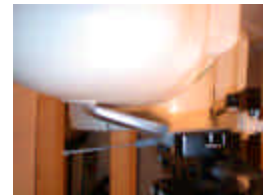
Figure 14.2 Right Head SAR Test Setup -- Ear / Tilt Position --
