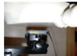
Figure 14.13 Body SAR Test Setup -- w/o Holster --
