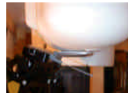
Figure 14.11 Left Head SAR Test Setup -- Cheek / Touch Position --
