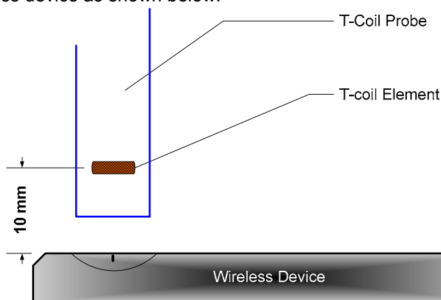
Figure 5-11 Measurement Distance
