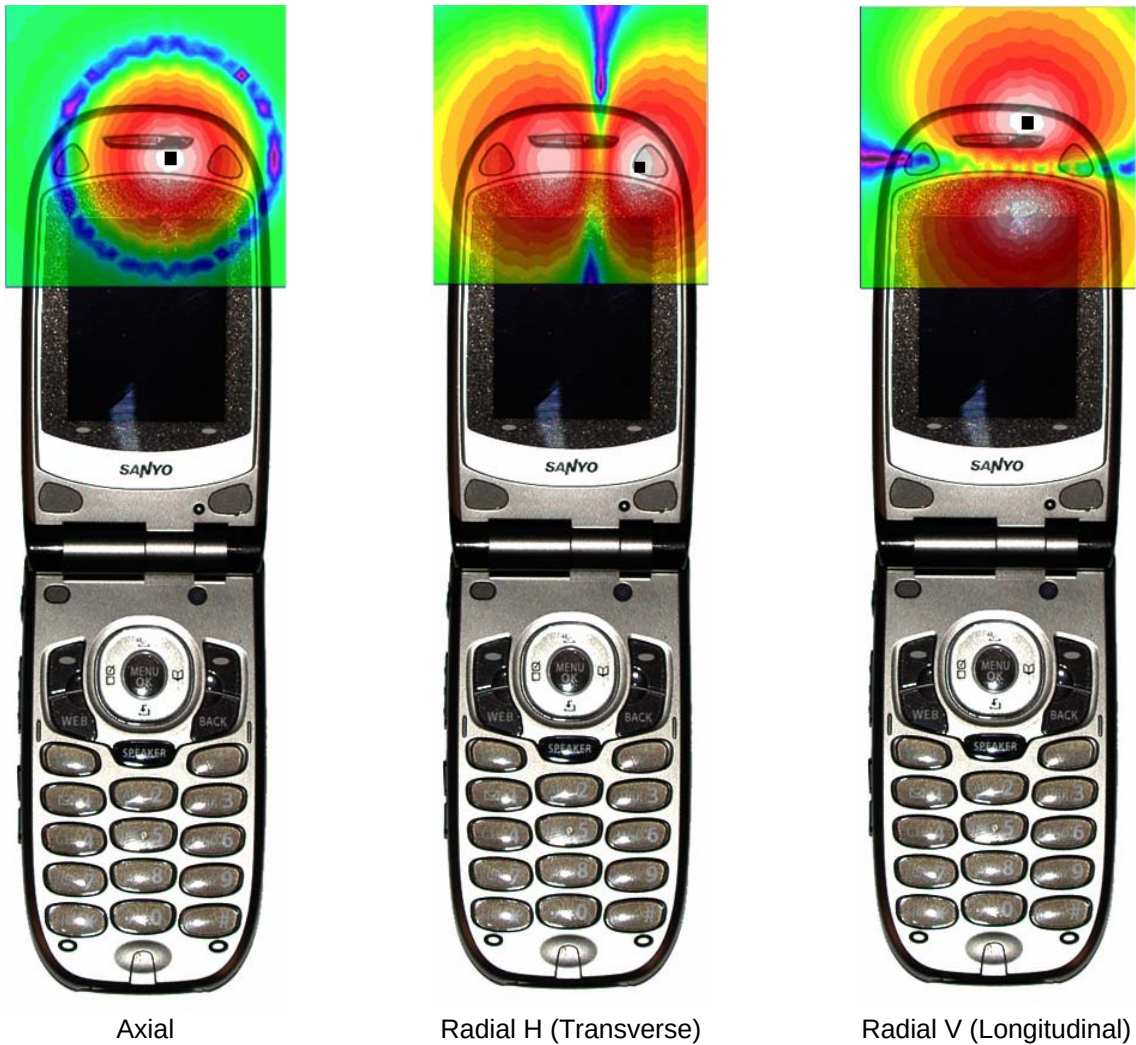
Figure 13-3 T-Coil Scan Overlay Magnetic Field Distributions
