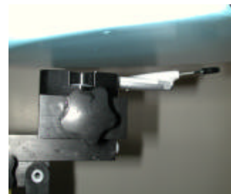
Figure 18. PCS Body SAR Test Setup
