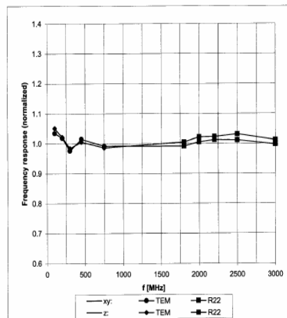
Figure 6 H-Field Probe Frequency Response
