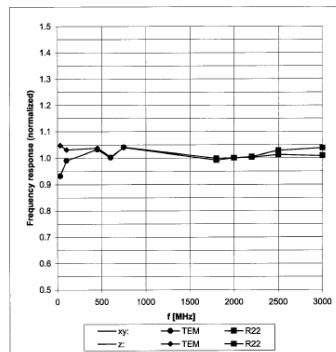
Figure 5 E-Field Probe Frequency Response
