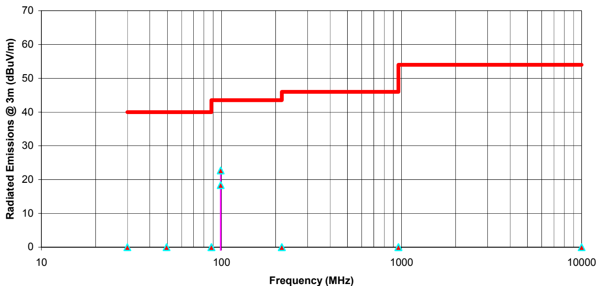
Radiated Emissions Measurements @ 3m OFTS Icom Scanning Receiver, Model IC-706MKIIG Receiver Frequency: 30 MHz in 0.03-200 MHz Band at ANT 1 and ANT 2 Ports
