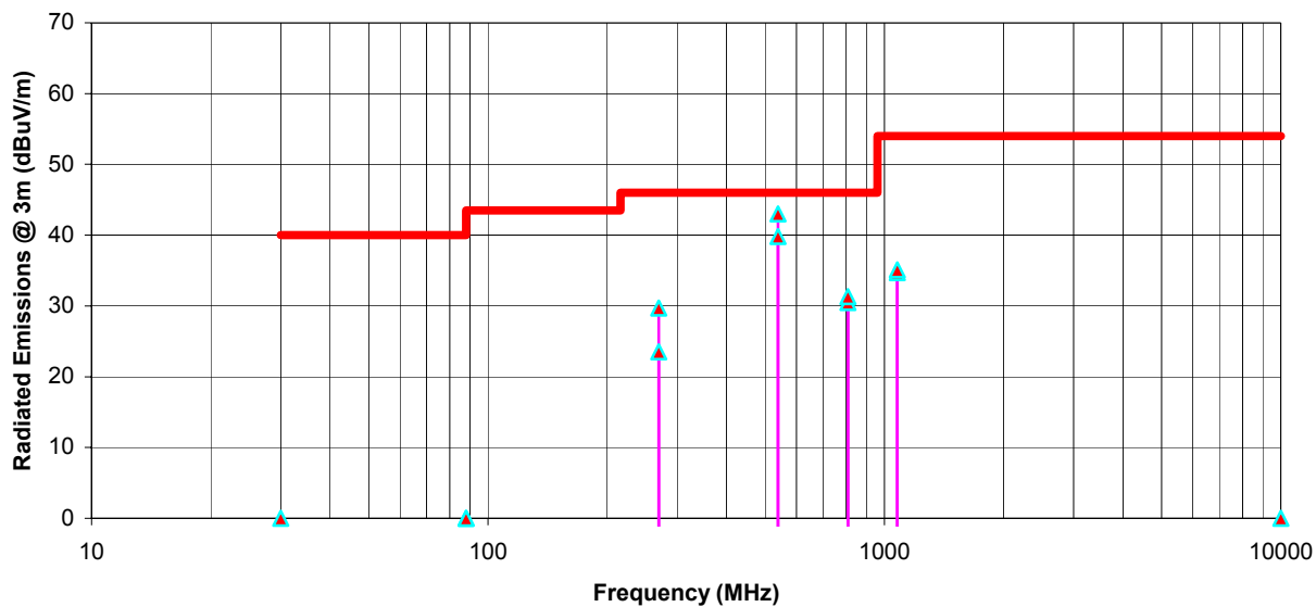
Radiated Emissions Measurements @ 3m OFTS Icom Scanning Receiver, Model IC-706MKIIG Receiver Frequency: 470 MHz in 400-470 MHz Band at ANT 1 and ANT 2 Ports
