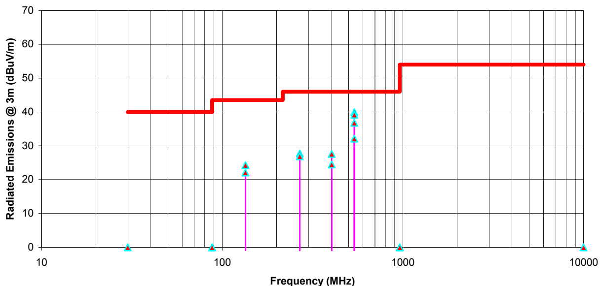
Radiated Emissions Measurements @ 3m OFTS Icom Scanning Receiver, Model IC-706MKIIG Receiver Frequency: 199.9 MHz in 0.03-200 MHz Band at ANT 1 and ANT 2 Ports
