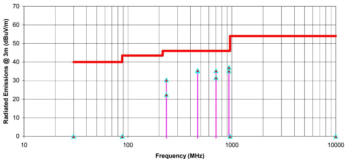
Radiated Emissions Measurements @ 3m OFTS Icom Scanning Receiver, Model IC-706MKIIG Receiver Frequency: 400 MHz in 400-470 MHz Band at ANT 1 and ANT 2 Ports
