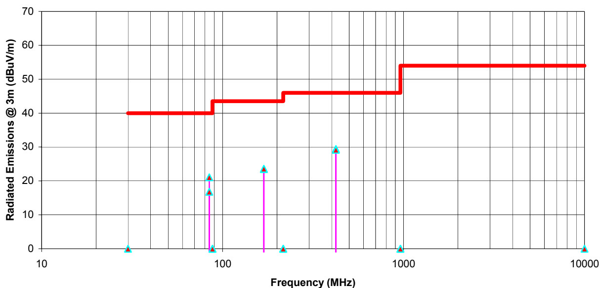
Radiated Emissions Measurements @ 3m OETS Icom Scanning Receiver, Model IC-706MKIIG Receiver Frequency: 100 MHz in 0.03-200 MHz Band at ANT 1 and ANT 2 Ports
