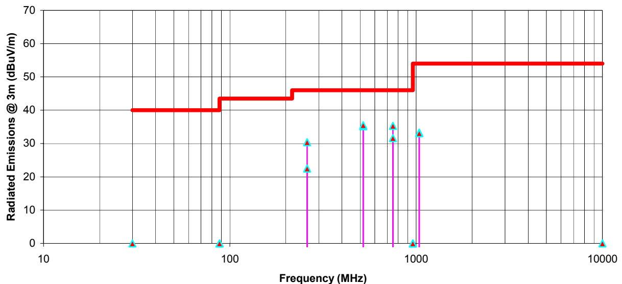
Radiated Emissions Measurements @ 3m OFTS Icom Scanning Receiver, Model IC-706MKIIG Receiver Frequency: 451 MHz in 400-470 MHz Band at ANT 1 and ANT 2 Ports
