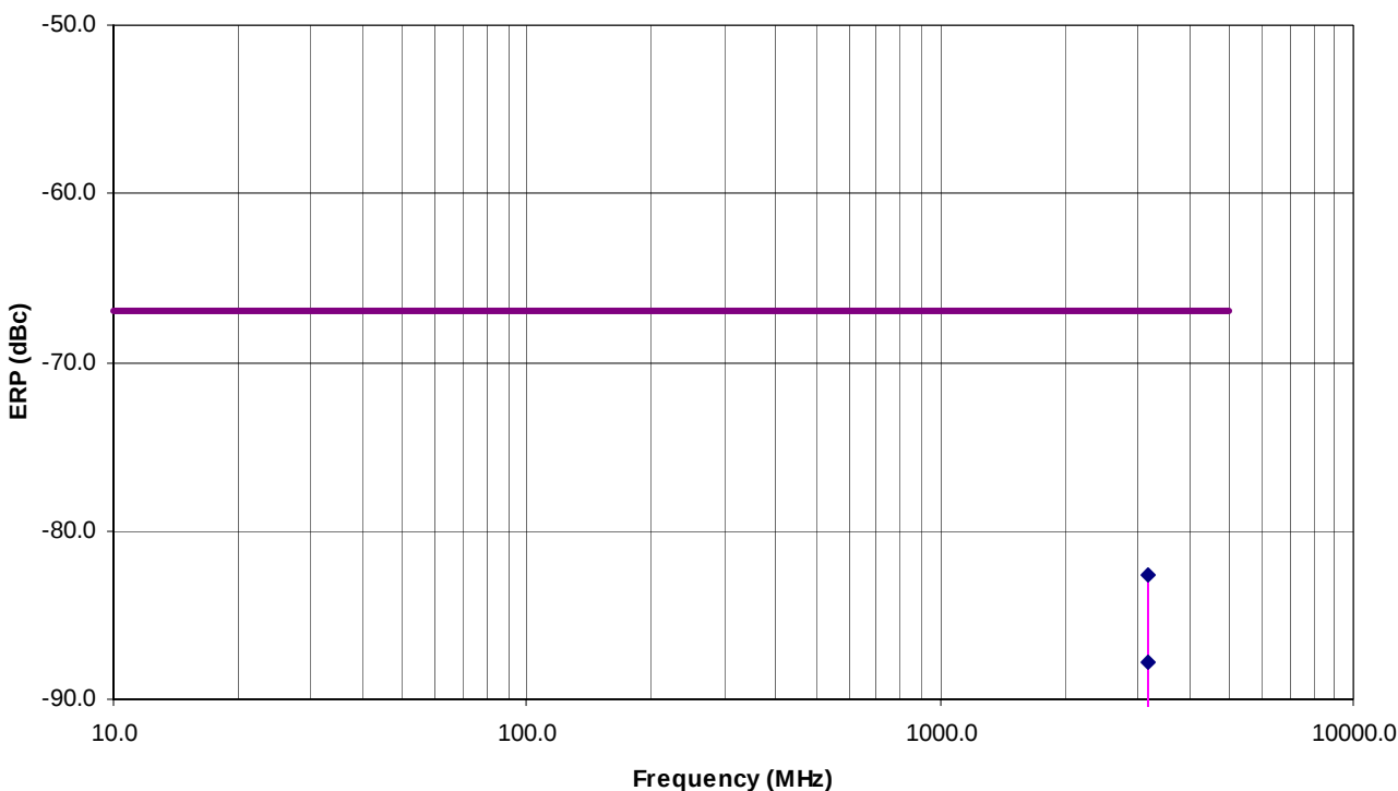
Radiated Emissions Measurements at 3 Meter OFTS ICOM UHF FM REPEATER, Model IC-FR4000-1 Tx Freq. = 400.1 MHz, RF Output: 47 dBm (conducted), Channel Spacing: 12.5 kHz
