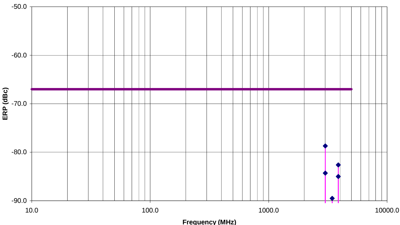
Radiated Emissions Measurements at 3 Meter OFTS ICOM UHF FM REPEATER, Model IC-FR4000-1 Tx Freq. = 429.9 MHz, RF Output: 47 dBm (conducted), Channel Spacing: 12.5 kHz
