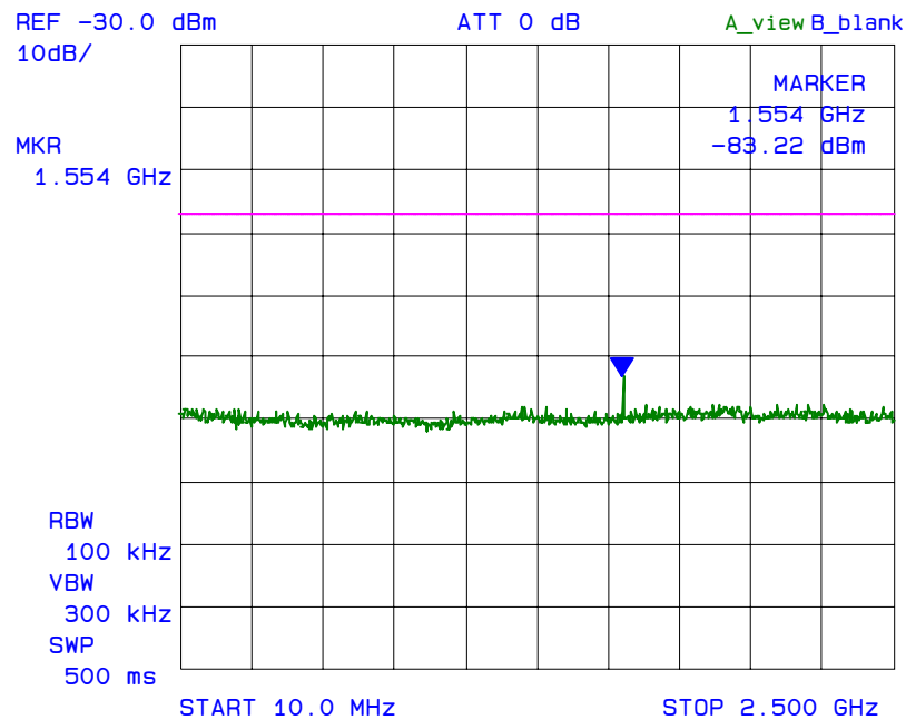
Plot 6.7.5.10 Receiver Conducted Emissions at ANT2 Rx Frequency: 400 MHz
