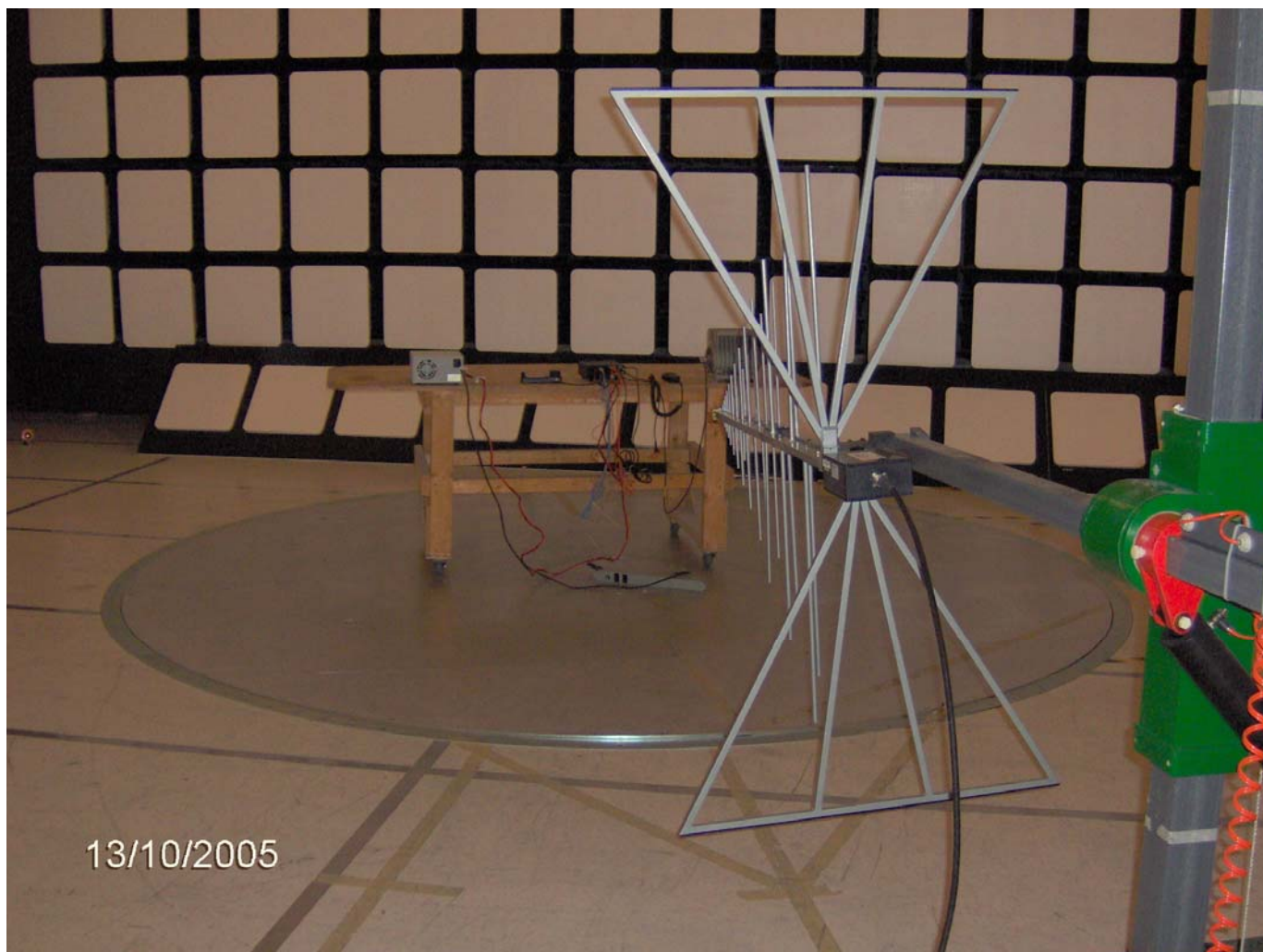
Radiated Emission at 3 Meters Distance
