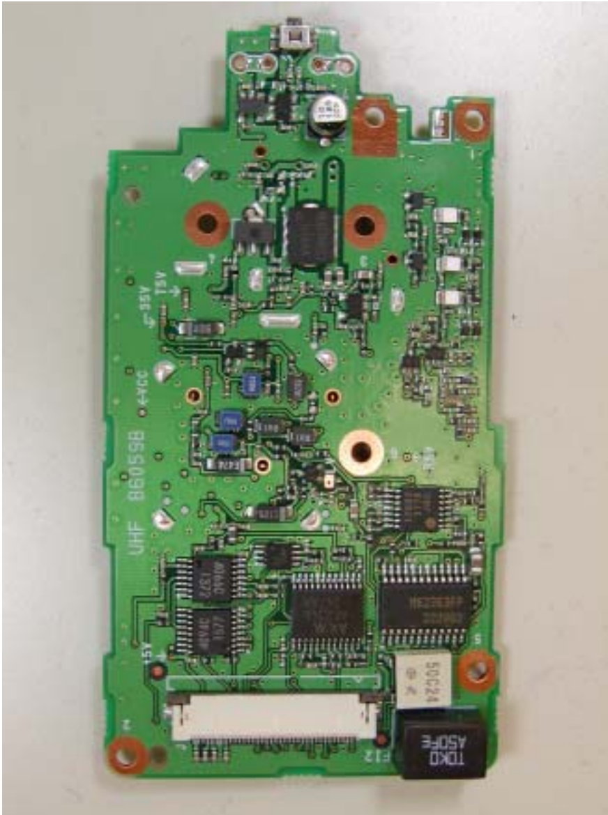
MAIN side A
