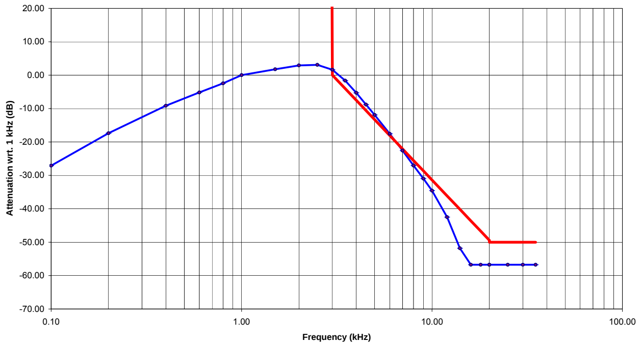
AUDIO FREQUENCY RESPONSE OF ALL MODULATION STAGES ICOM VHF Radio Transceiver, Model IC-M502A (25 kHz Channel Spacing)
