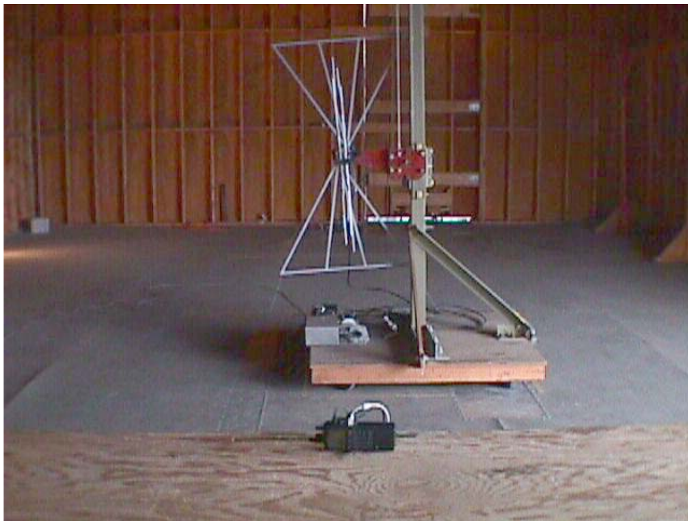
Radiated Emissions at 3 Meters (Orthogonal Position # 3)
