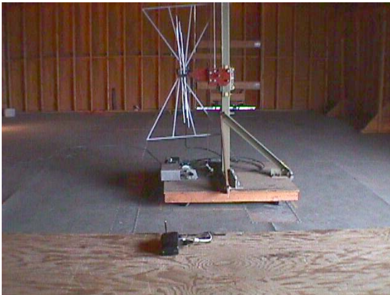
Radiated Emissions at 3 Meters (Orthogonal Position # 2)
