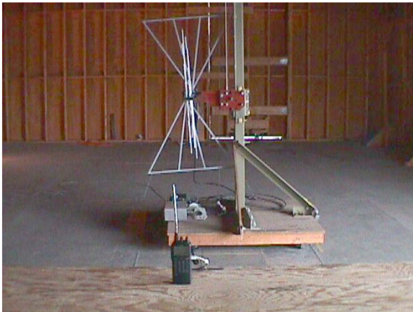
Radiated Emissions at 3 Meters (Orthogonal Position # 1)
