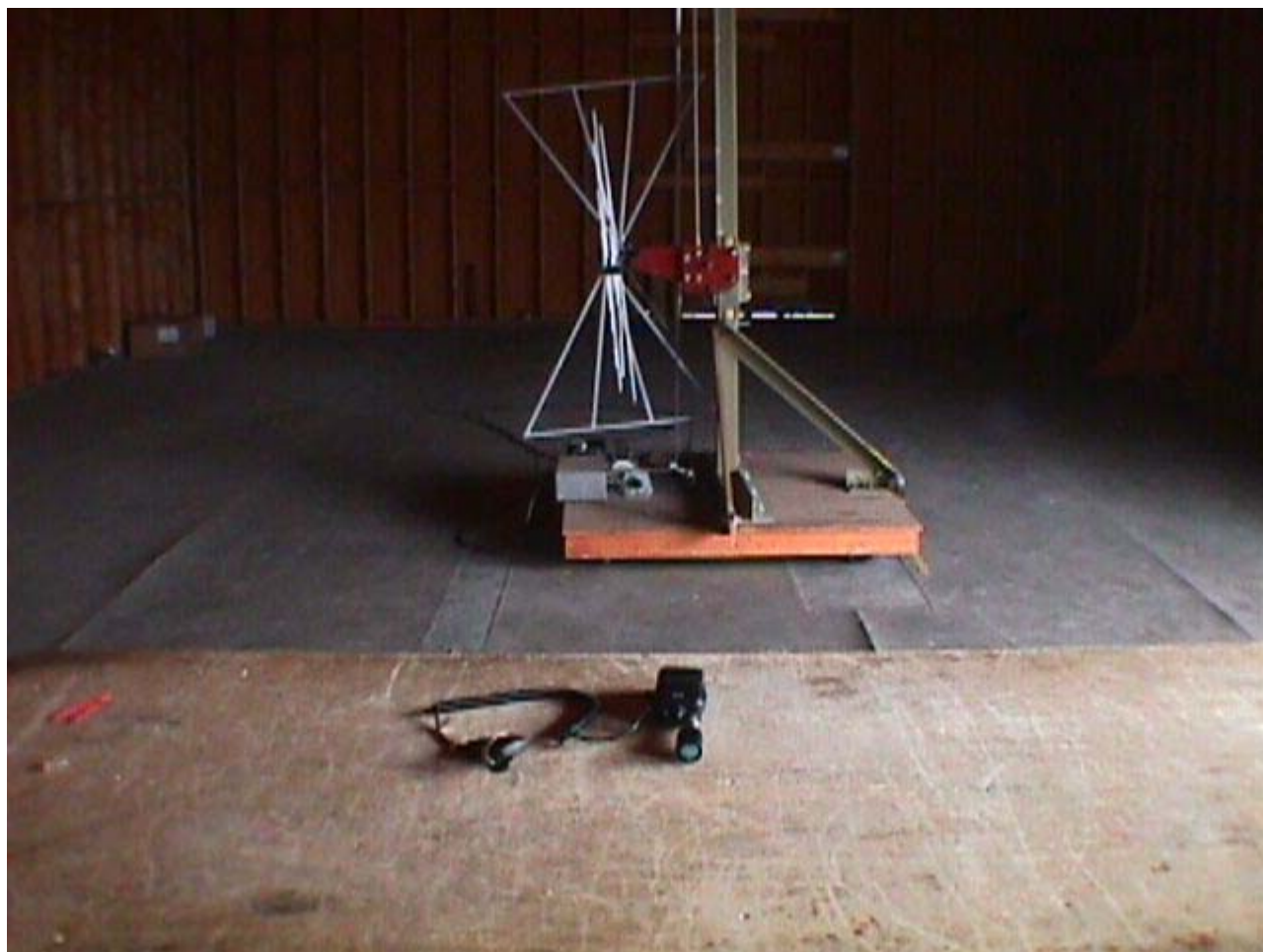
Radiated Emissions Orthogonal Position #2
