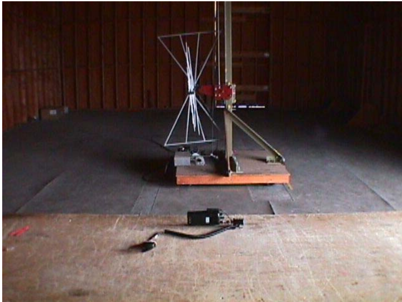
Radiated Emissions Orthogonal Position #3
