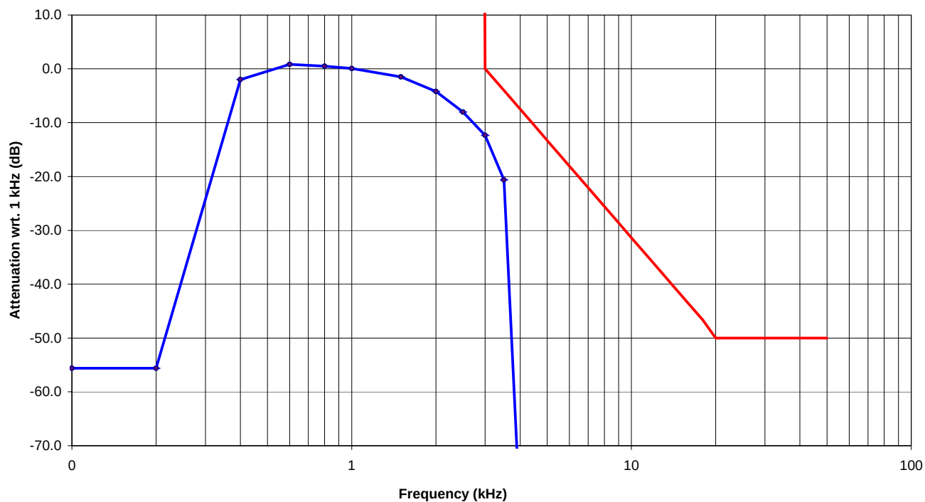
Audio Frequency Response @ FCC 2.1047(a) & 90.242(b)(8) ICOM Model: IC-F24/S, 12.5 kHz Channel Spacing
