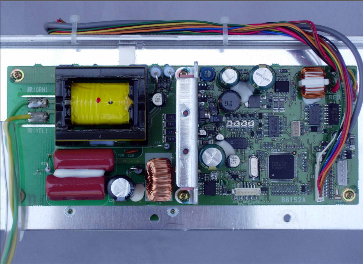
PA Unit
