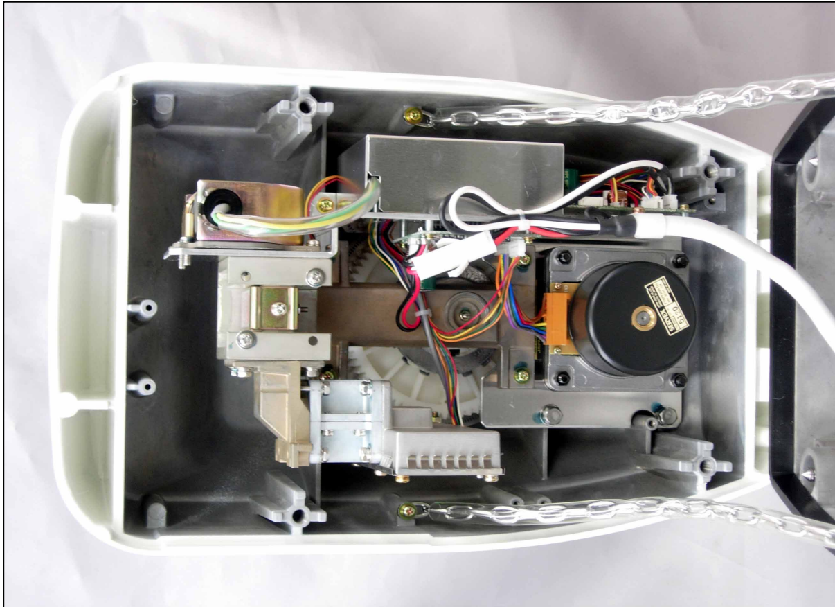
Internal View
