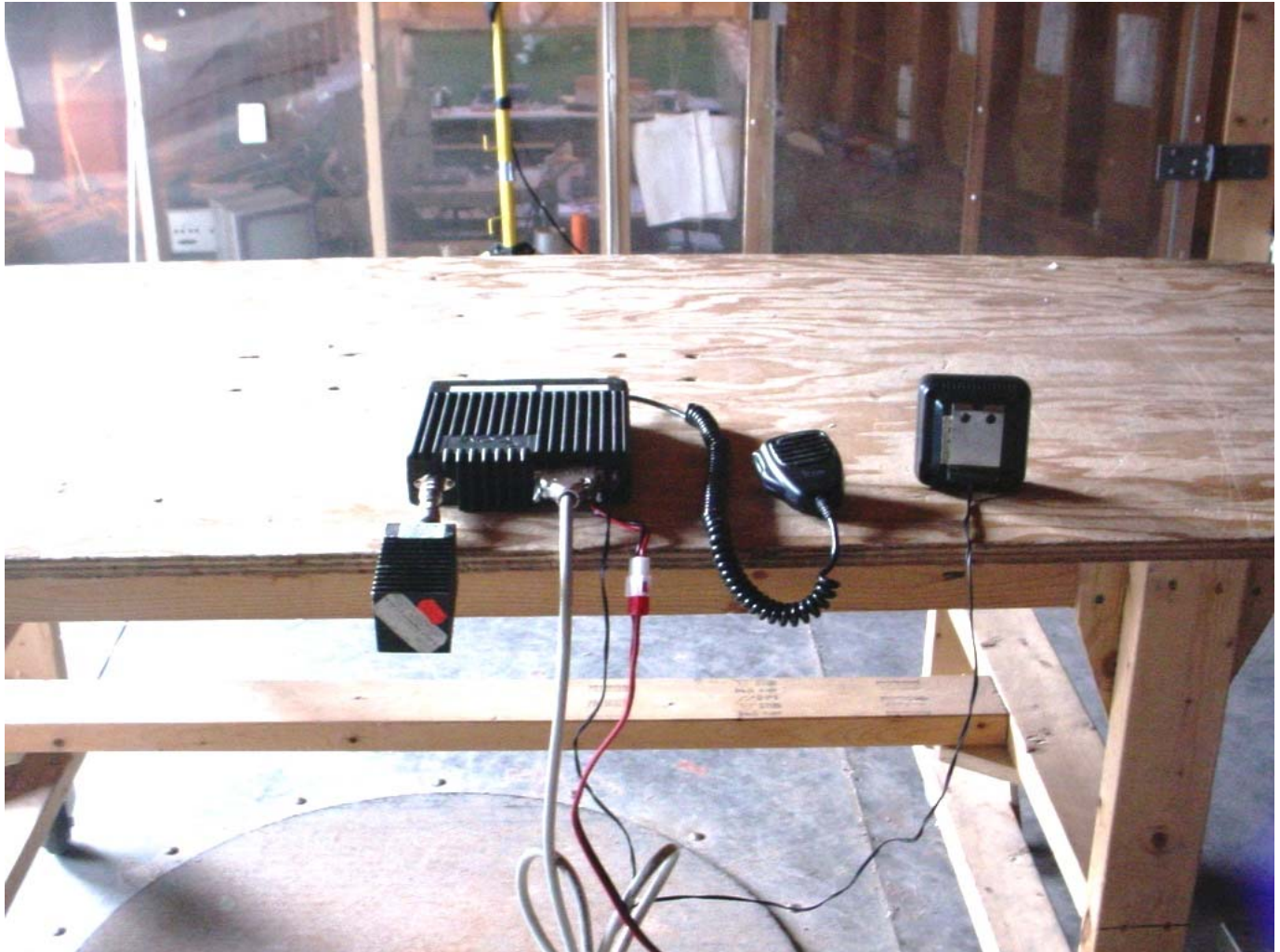
Radiated Emissions at 3 Meters
