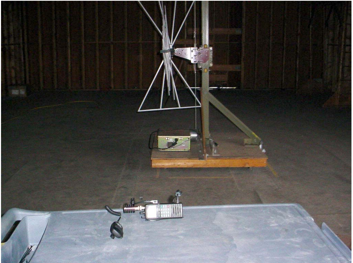
Radiated Emissions Orthogonal Position #2
