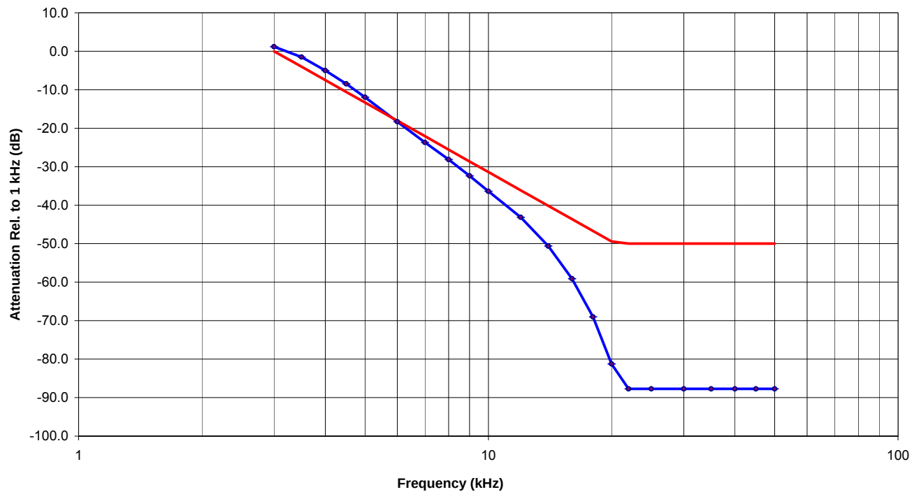
Audio Frequency Response 25 kHz Channel Spacing ICOM Model: IC-M504, VHF Marine Transceiver
