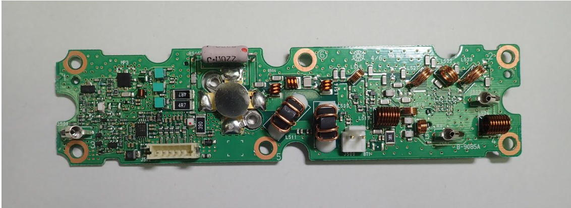
PA-D (TOP)
