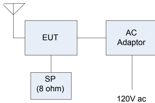
Setup for Unintentional Radiated Emissions from Digital devices
