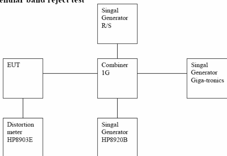
Cellular band reject test
