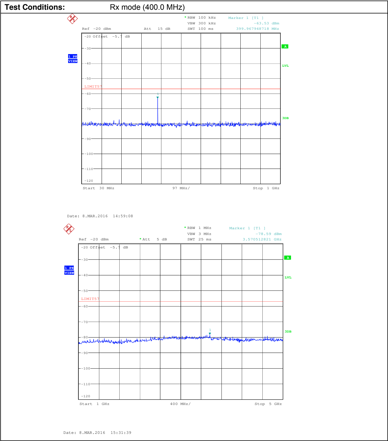
Plot 4: Conducted Receiver Spurious Emissions, 30 MHz – 5.0 GHz
