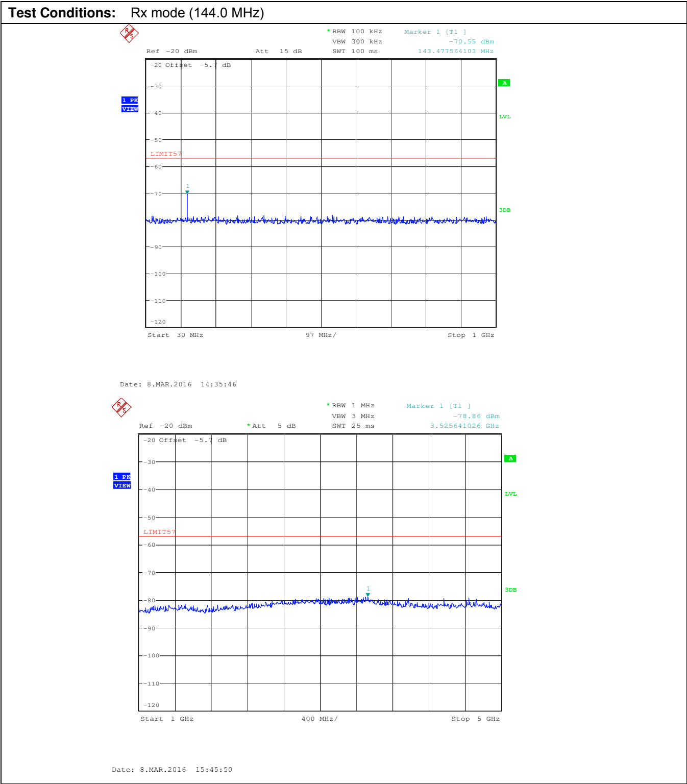
Plot 8: Conducted Receiver Spurious Emissions, 30 MHz – 5 GHz
