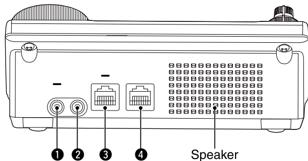
Rear panel
