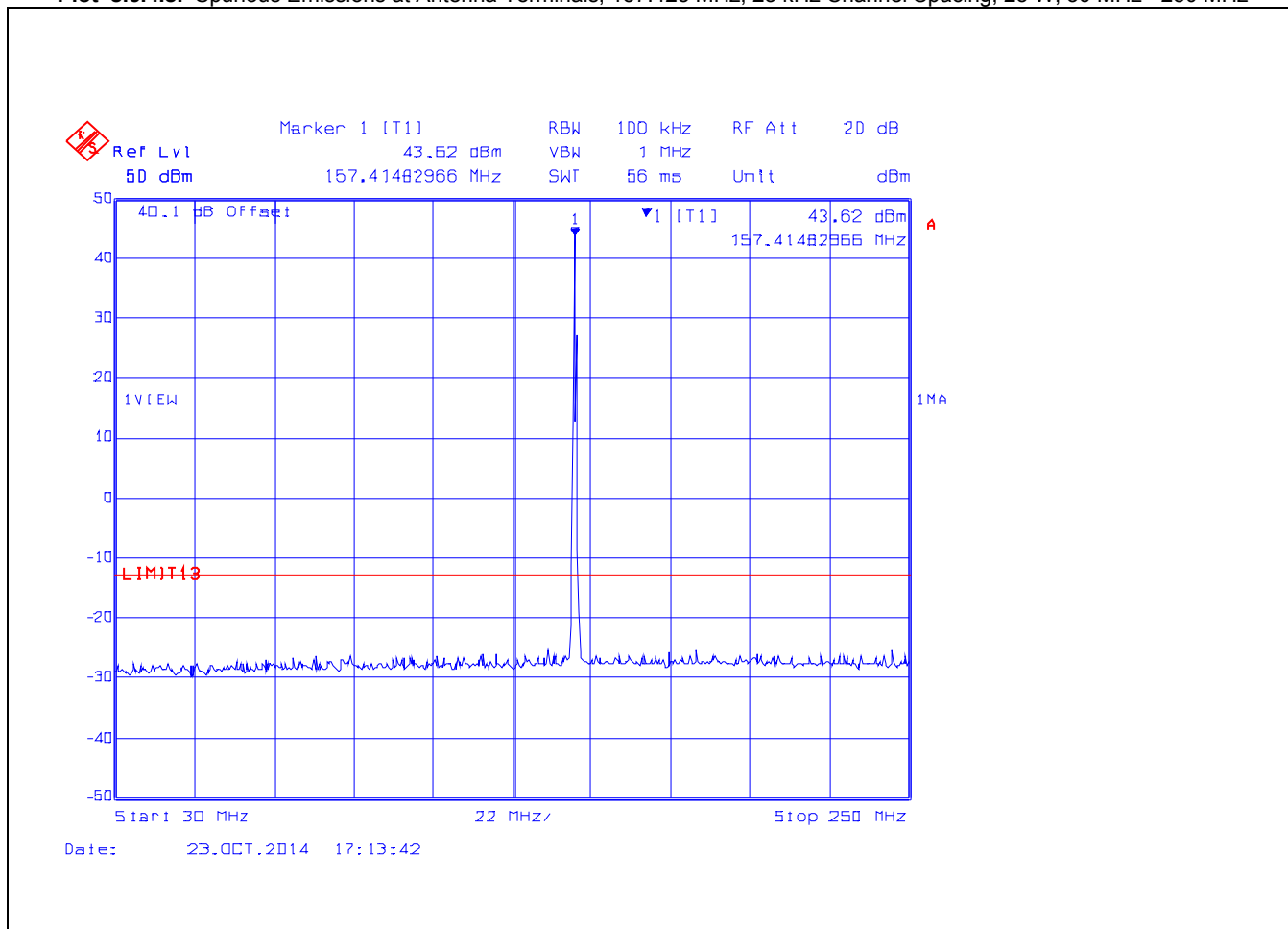
Plot 5.6.4.5. Spurious Emissions at Antenna Terminals, 157.425 MHz, 25 kHz Channel Spacing, 25 W, 30 MHz - 250 MHz
