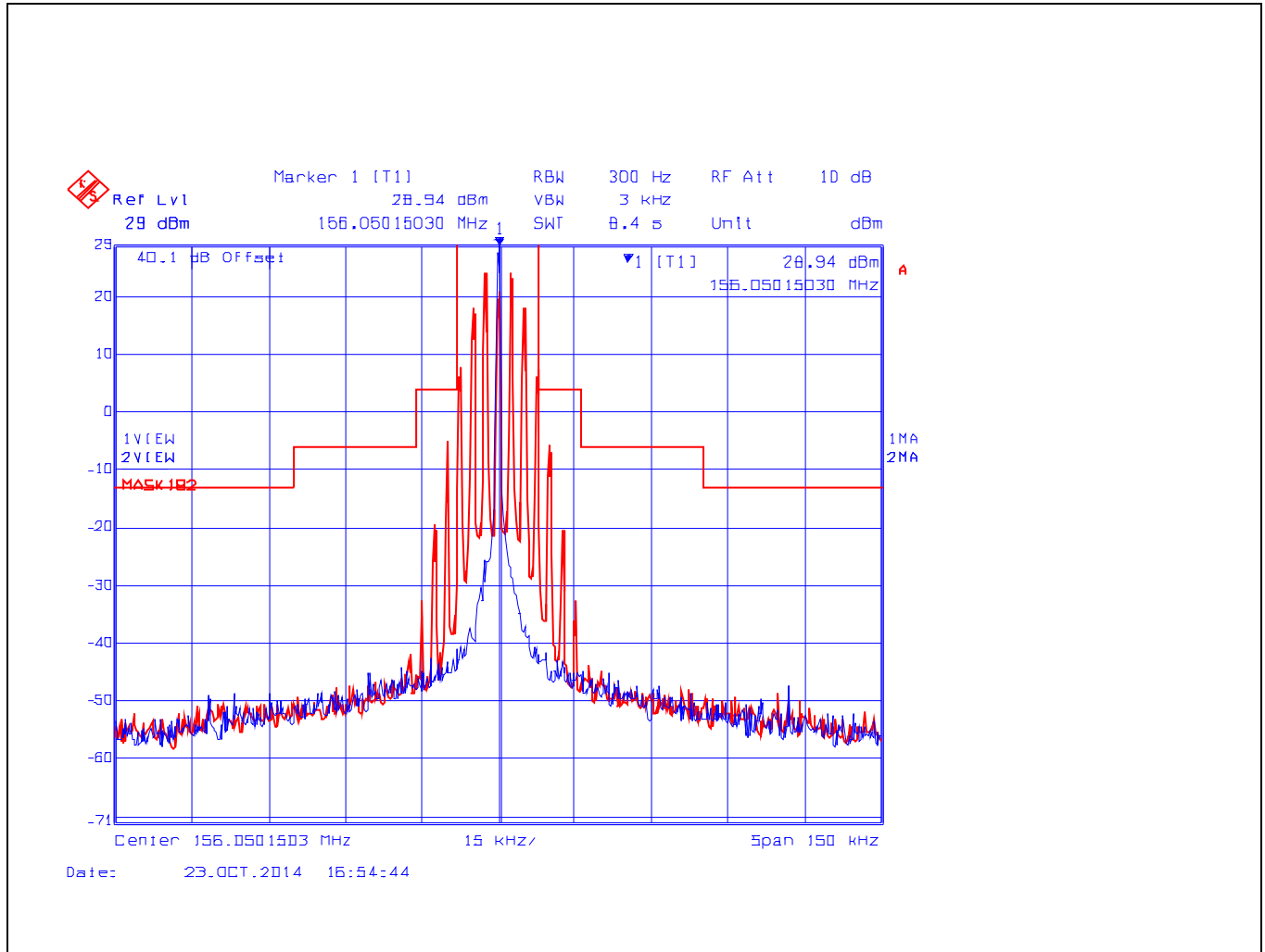
Plot 5.5.4.2.2. Emission Limitation for 156.050 MHz, 25 kHz Channel Spacing, Low Power (1 W), G3E, 150 kHz Span
