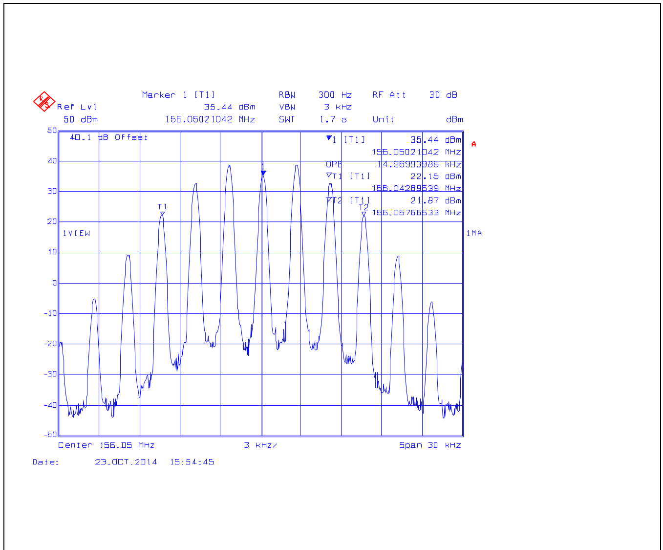
Plot 5.5.4.1.1. Occupied Bandwidth for 156.050 MHz, 25 kHz Channel Spacing, High Power (25 W), G3E
