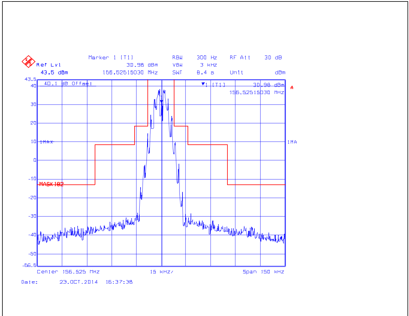
Plot 5.5.4.2.5. Emission Limitation for 156.525 MHz, 25 kHz Channel Spacing, High Power (25 W), DSC-G2B
