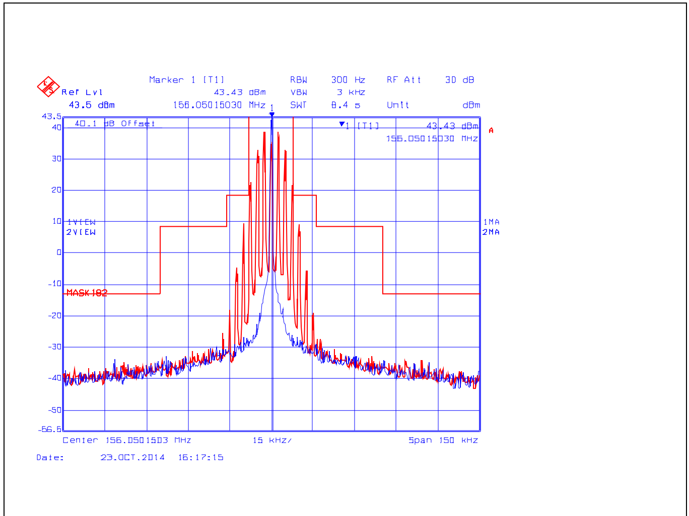
Plot 5.5.4.2.1. Emission Limitation for 156.050 MHz, 25 kHz Channel Spacing, High Power (25 W), G3E, 150 kHz Span
