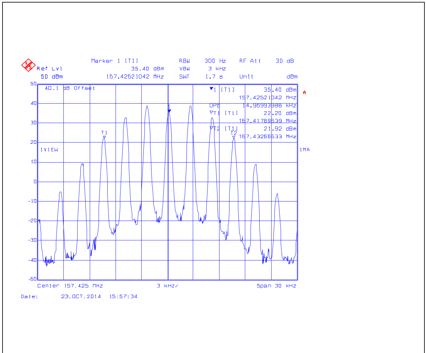
Plot 5.5.4.1.2. Occupied Bandwidth for 157.425 MHz, 25 kHz Channel Spacing, High Power (25 W), G3E
