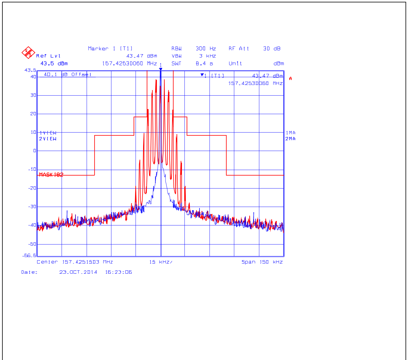
Plot 5.5.4.2.3. Emission Limitation for 157.425 MHz, 25 kHz Channel Spacing, High Power (25 W), G3E, 150 kHz Span
