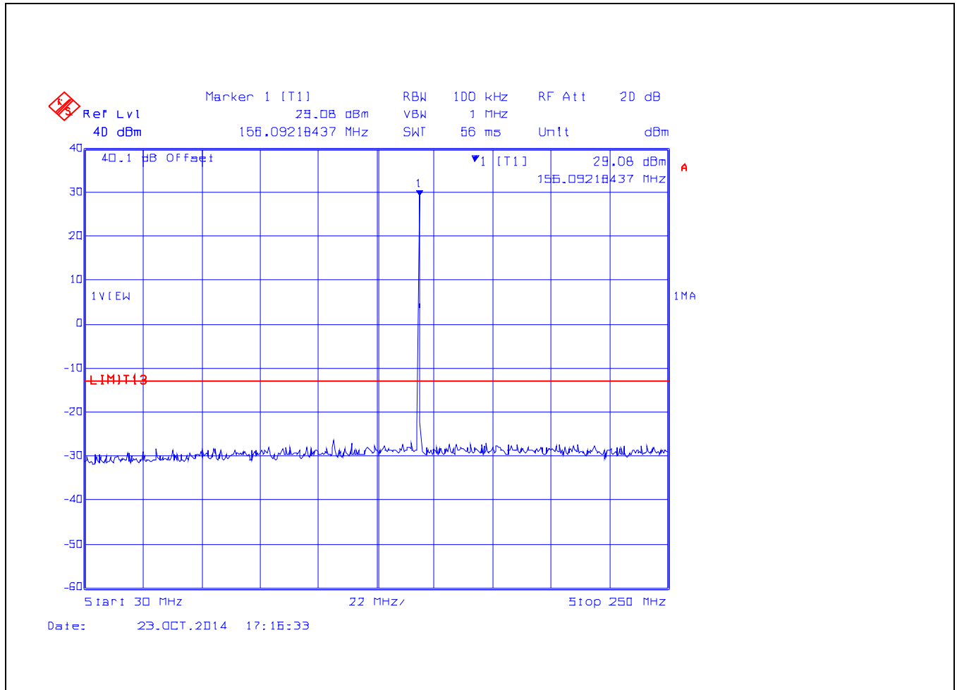
Plot 5.6.4.3. Spurious Emissions at Antenna Terminals, 156.050 MHz, 25 kHz Channel Spacing, 1 W, 30 MHz - 250 MHz
