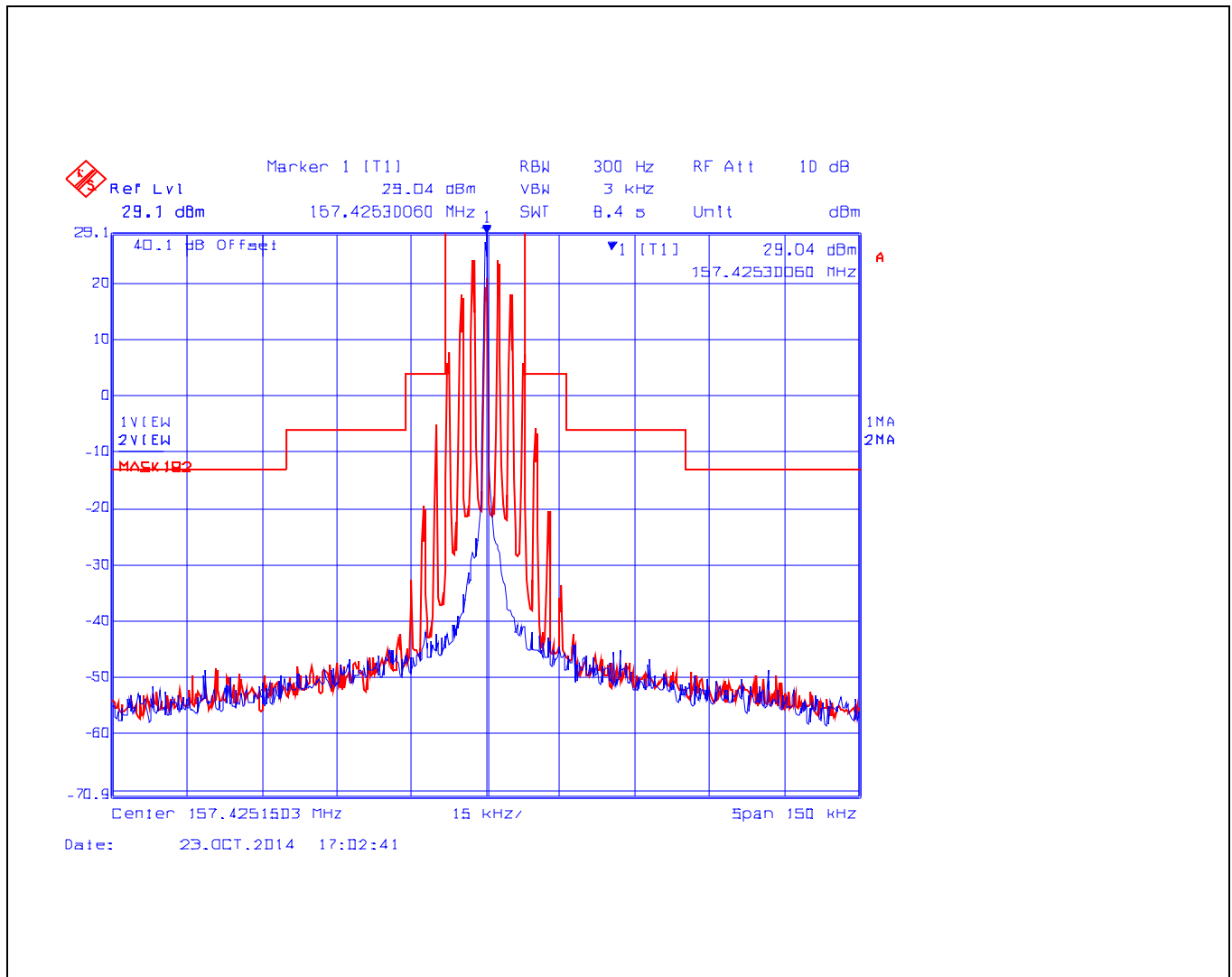
Plot 5.5.4.2.4. Emission Limitation for 157.425 MHz, 25 kHz Channel Spacing, Low Power (1 W), G3E, 150 kHz Span
