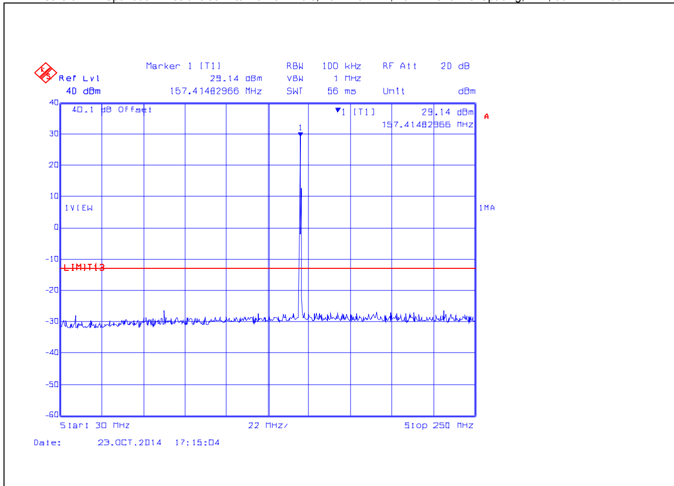
Plot 5.6.4.7. Spurious Emissions at Antenna Terminals, 157.425 MHz, 25 kHz Channel Spacing, 1 W, 30 MHz - 250 MHz
