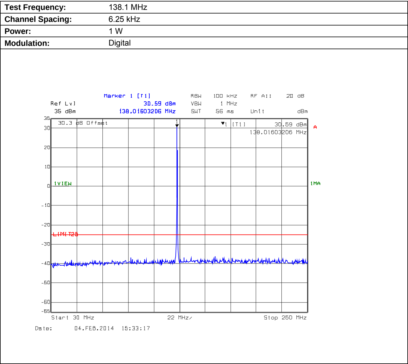
Plot 5.9.4.1.1. Conducted Transmitter Spurious Emissions for 138.1 MHz, High Power, 30 MHz - 250 MHz
