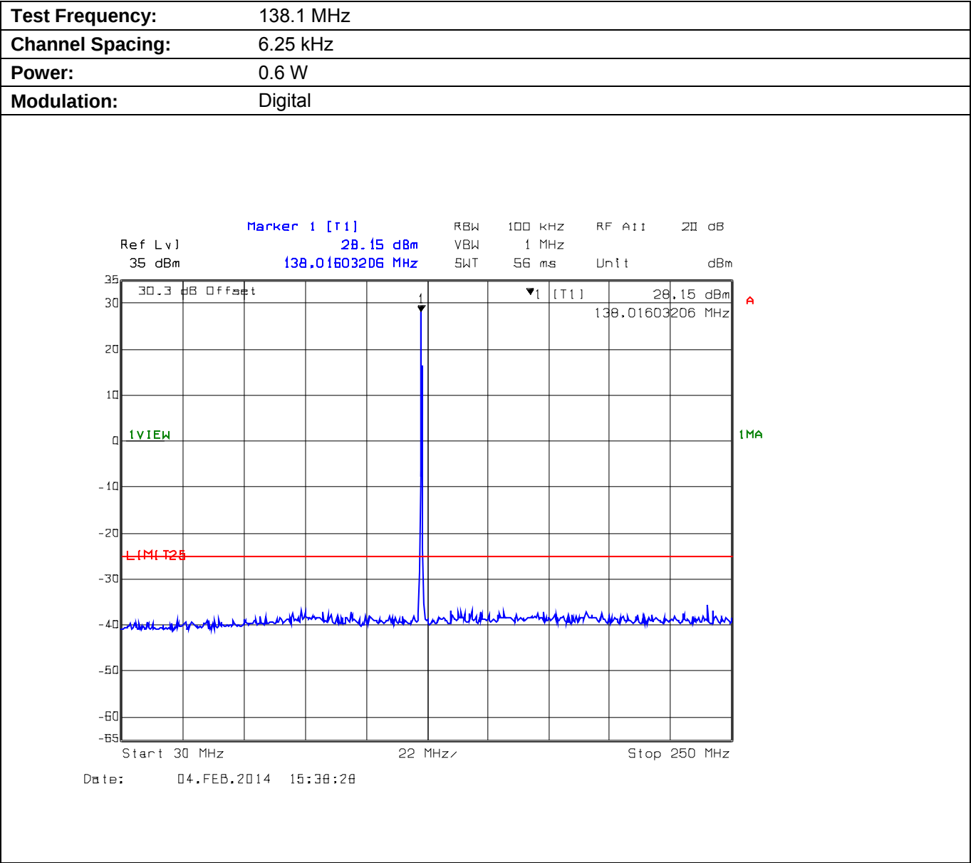
Plot 5.9.4.1.3. Conducted Transmitter Spurious Emissions for 138.1 MHz, Low Power, 30 MHz - 250 MHz
