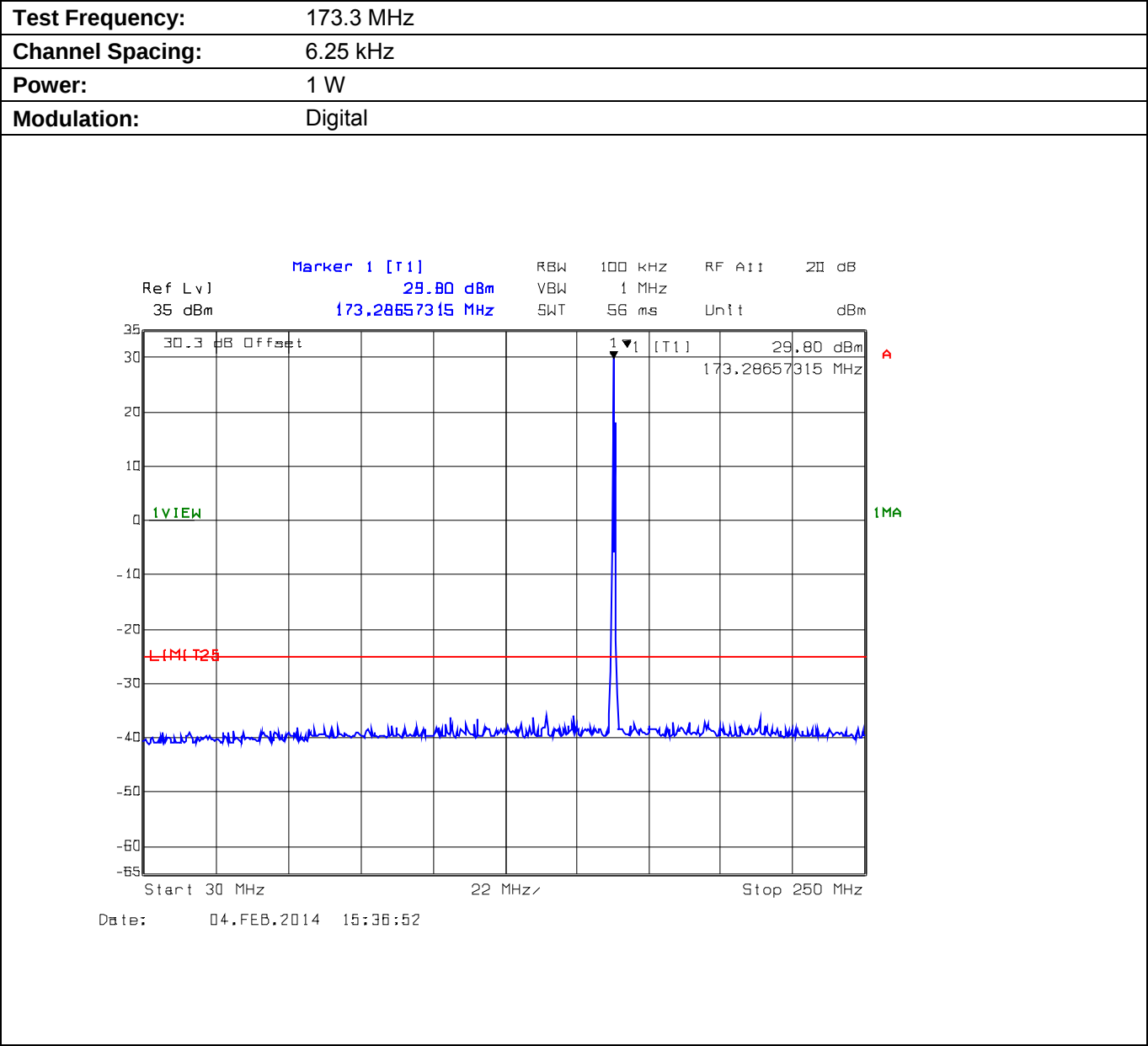
Plot 5.9.4.3.1. Conducted Transmitter Spurious Emissions for 173.3 MHz, High Power, 30 MHz - 250 MHz
