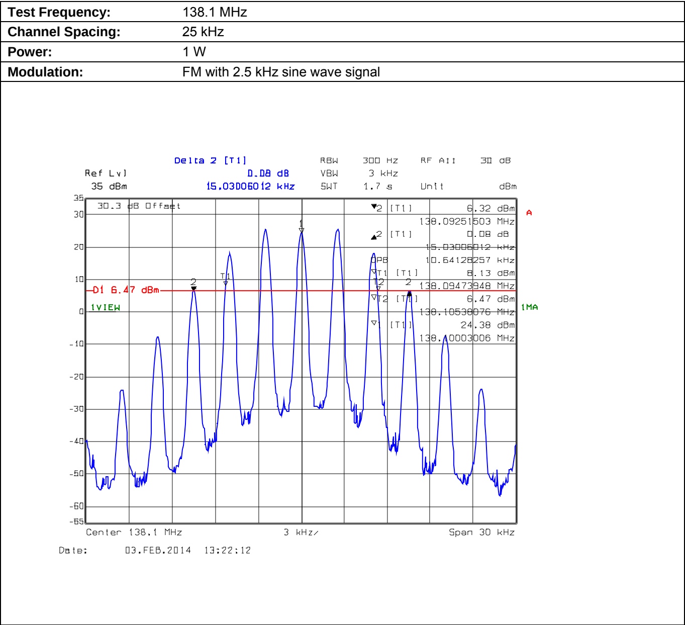
Plot 5.8.4.1.4. Occupied Bandwidth
