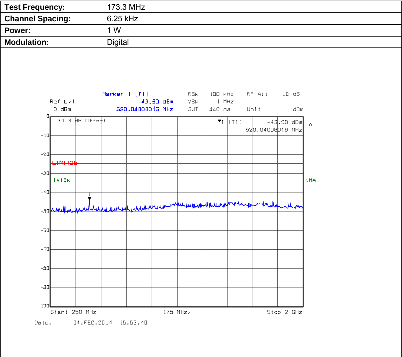
Plot 5.9.4.3.2. Conducted Transmitter Spurious Emissions for 173.3 MHz, High Power, 250 MHz - 2 GHz
