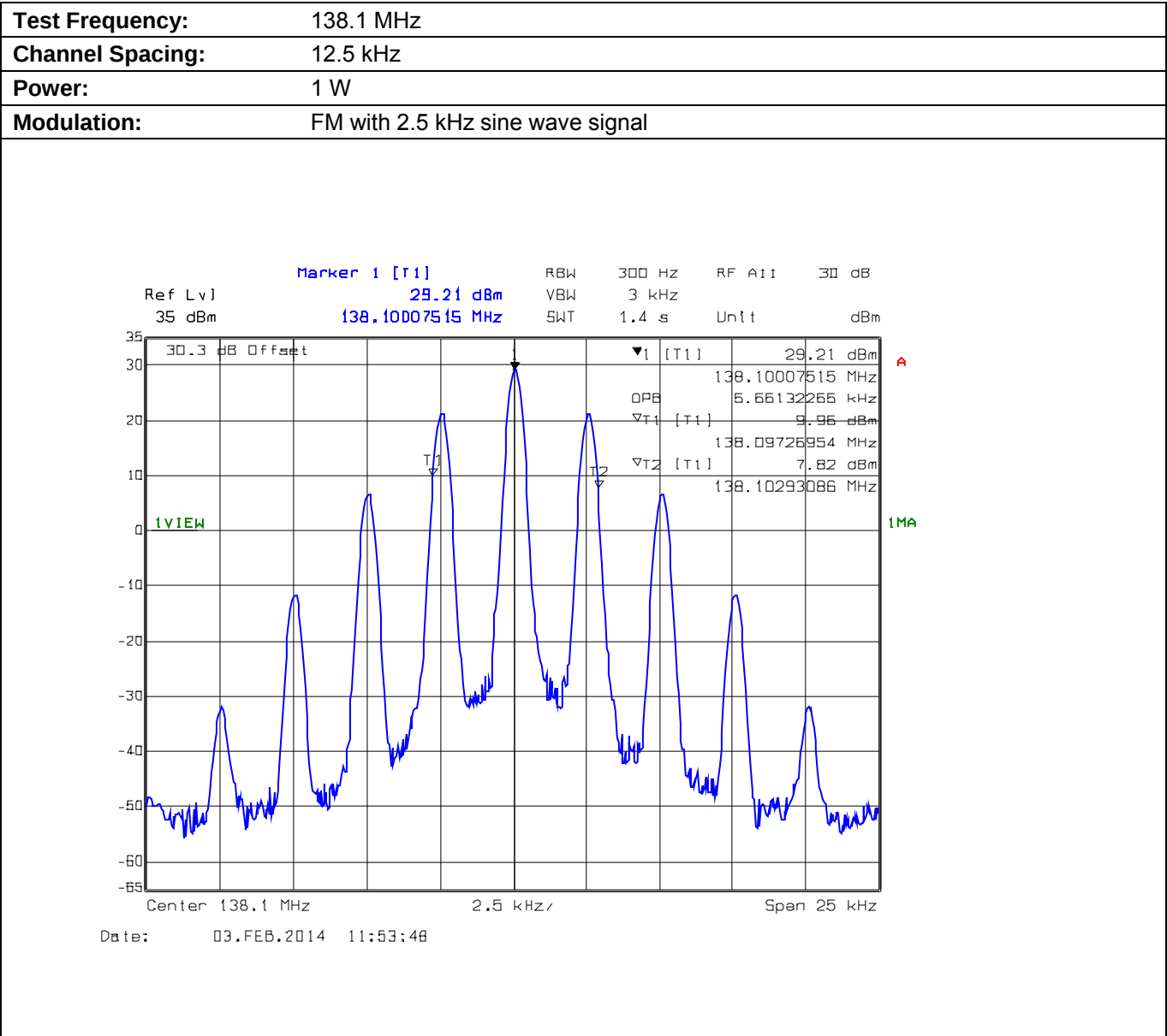
Plot 5.8.4.1.1. Occupied Bandwidth
