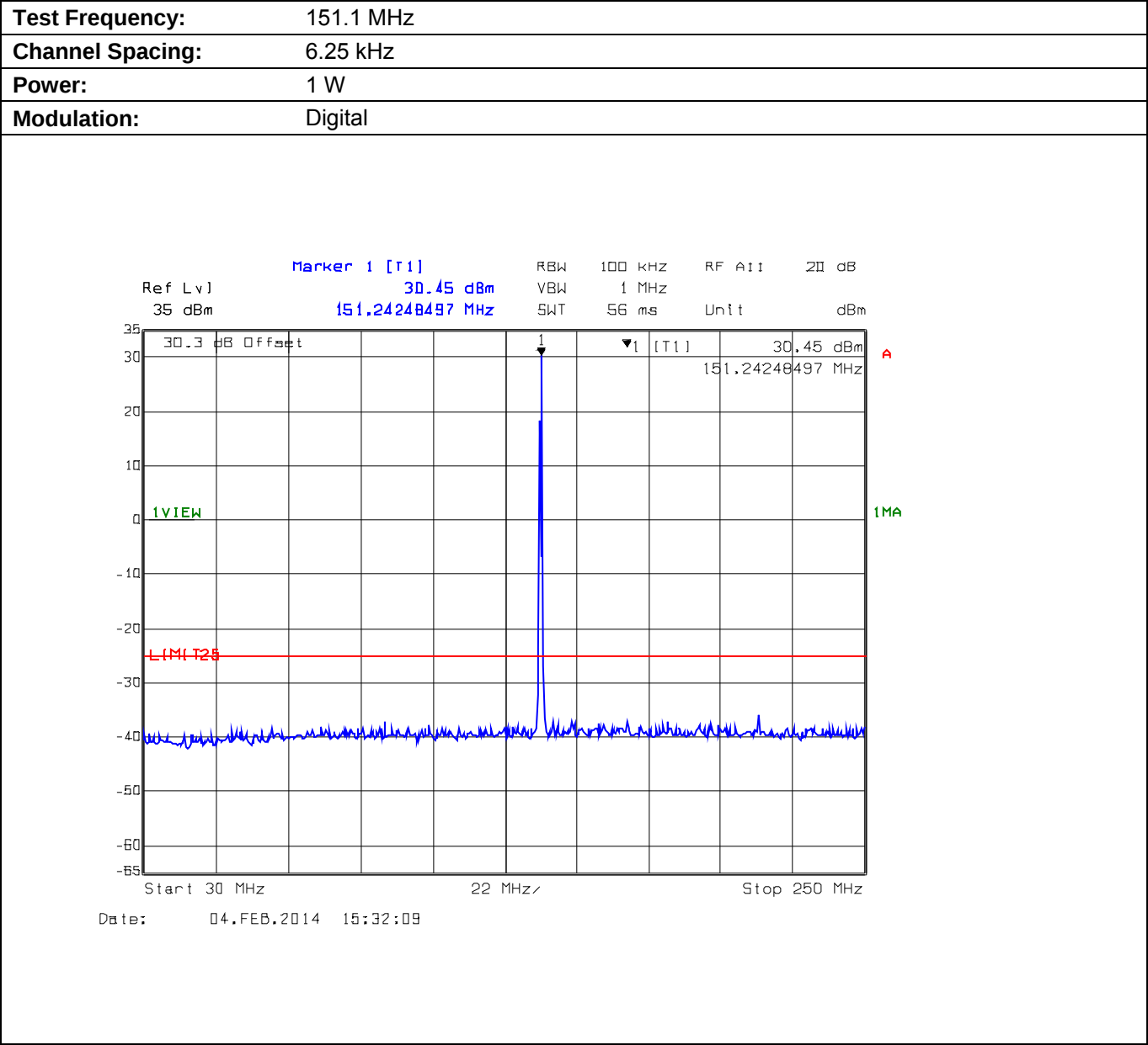
Plot 5.9.4.2.1. Conducted Transmitter Spurious Emissions for 151.1 MHz, High Power, 30 MHz - 250 MHz
