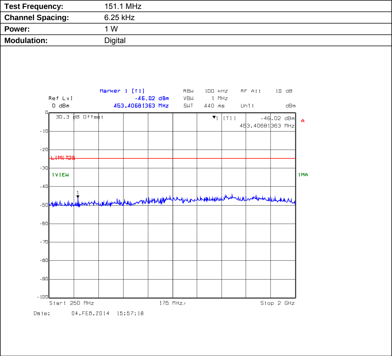
Plot 5.9.4.2.2. Conducted Transmitter Spurious Emissions for 151.1 MHz, High Power, 250 MHz - 2 GHz
