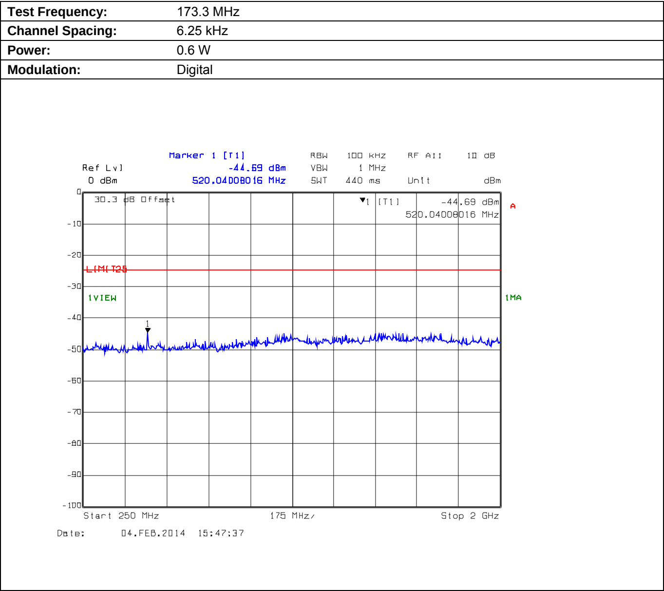
Plot 5.9.4.3.4. Conducted Transmitter Spurious Emissions for 173.3 MHz, Low Power, 250 MHz - 2 GHz
