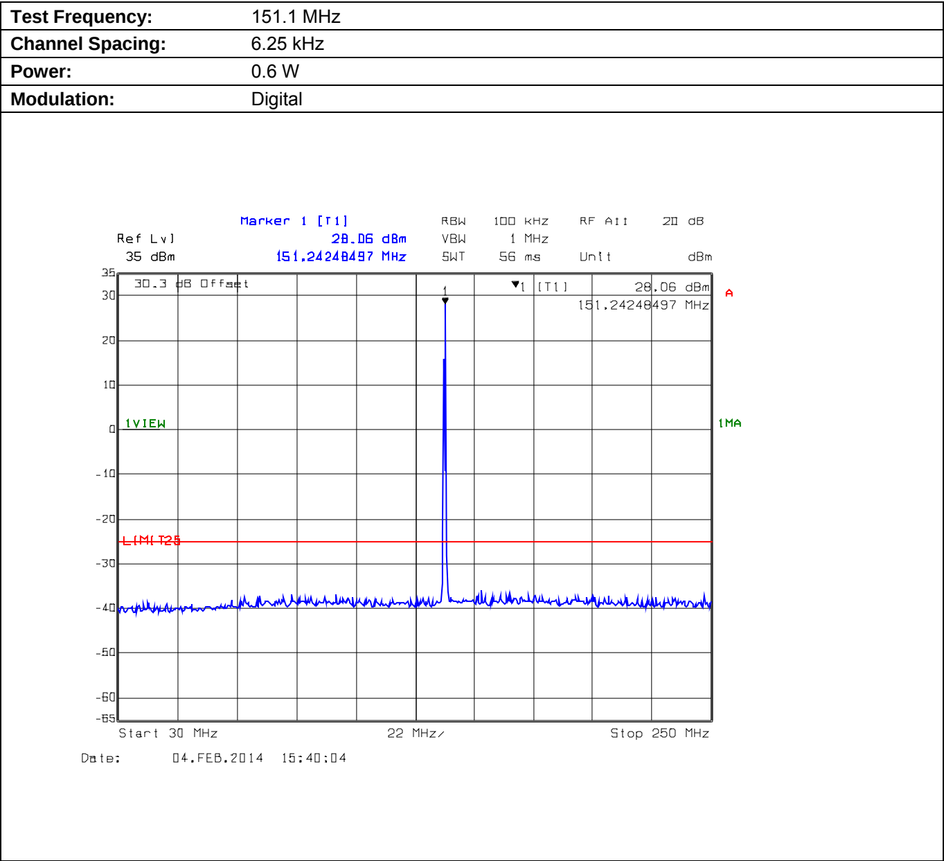
Plot 5.9.4.2.3. Conducted Transmitter Spurious Emissions for 151.1 MHz, Low Power, 30 MHz - 250 MHz
