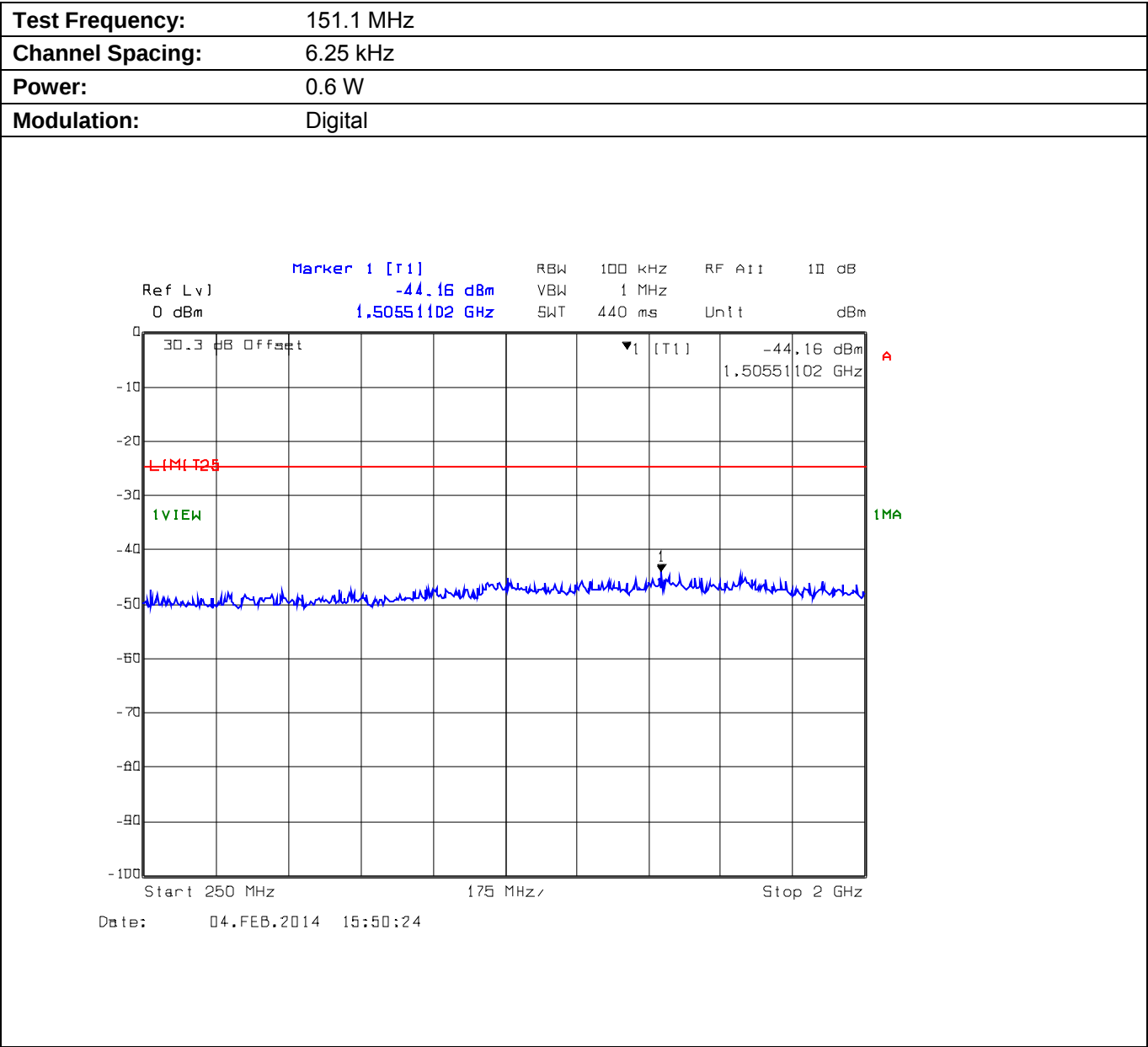
Plot 5.9.4.2.4. Conducted Transmitter Spurious Emissions for 151.1 MHz, Low Power, 250 MHz – 2 GHz
