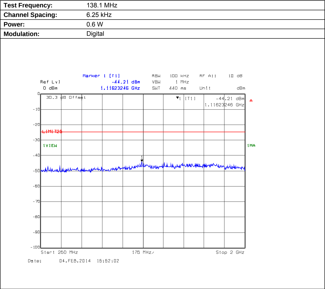
Plot 5.9.4.1.4. Conducted Transmitter Spurious Emissions for 138.1 MHz, Low Power, 250 MHz - 2 GHz
