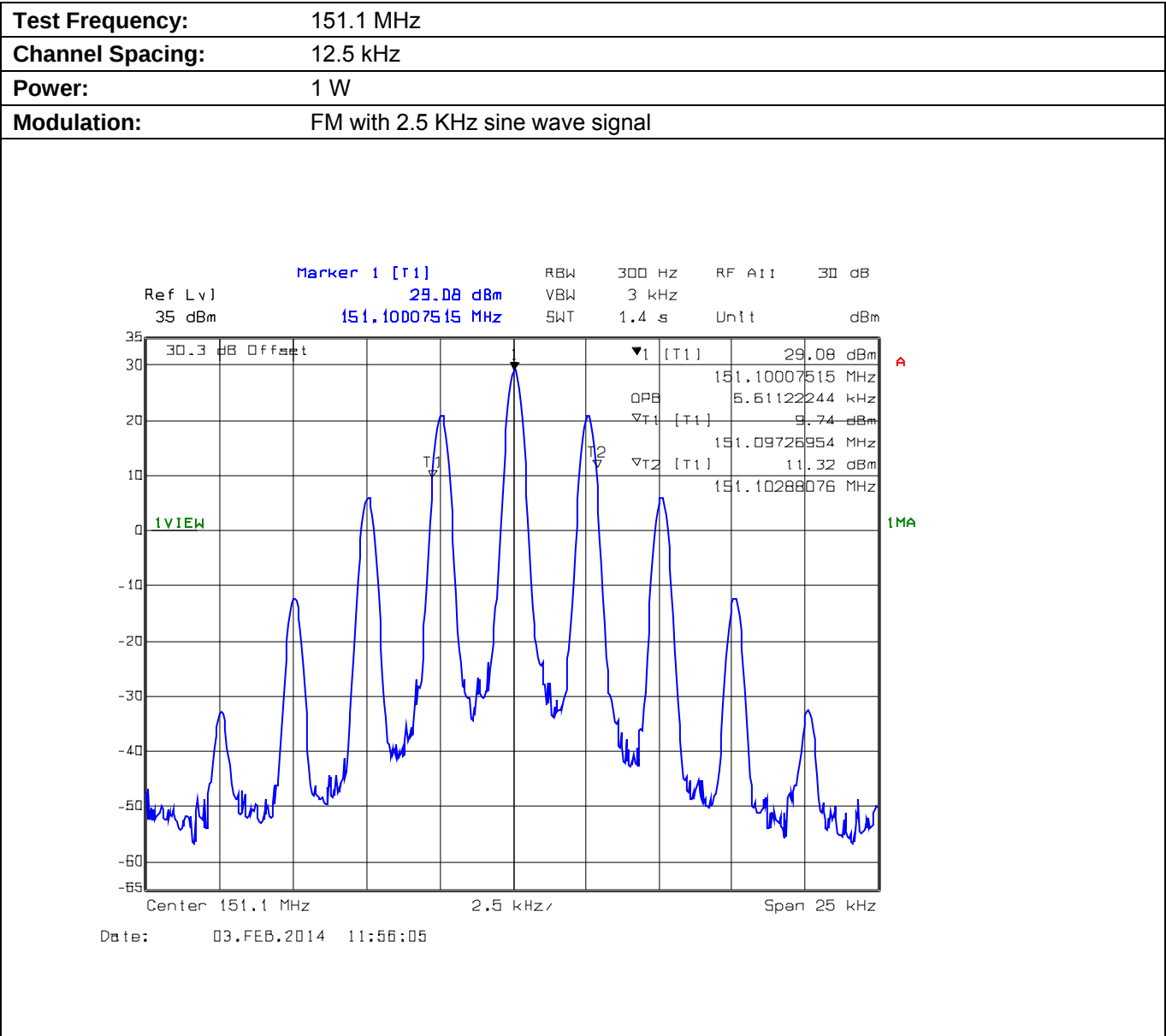
Plot 5.8.4.1.2. Occupied Bandwidth
