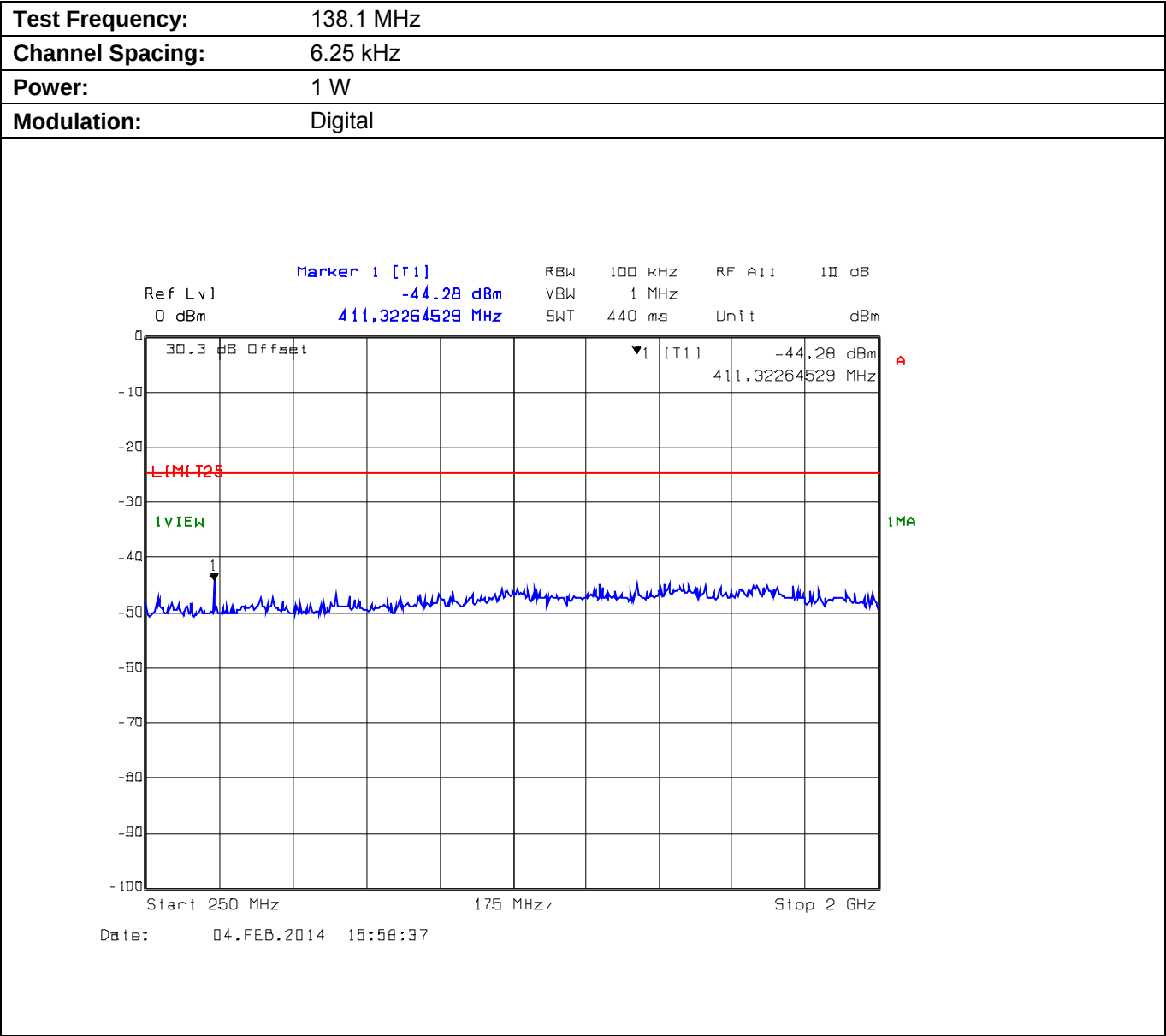
Plot 5.9.4.1.2. Conducted Transmitter Spurious Emissions for 138.1 MHz, High Power, 250 MHz - 2 GHz
