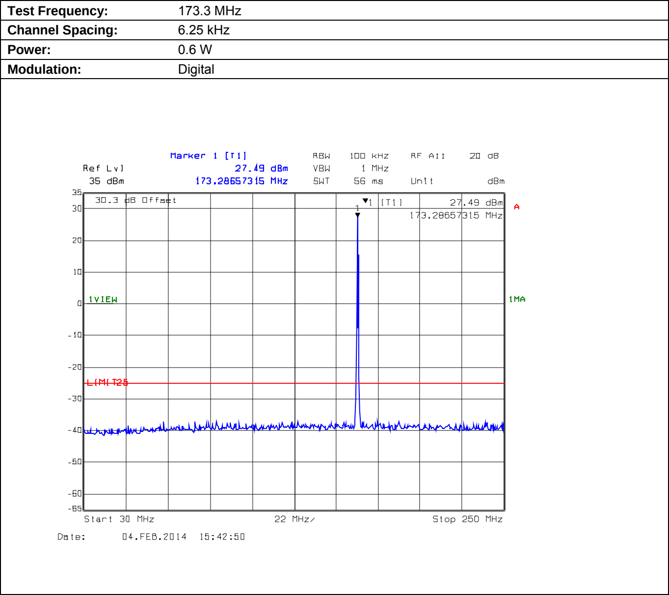
Plot 5.9.4.3.3. Conducted Transmitter Spurious Emissions for 173.3 MHz, Low Power, 30 MHz - 250 MHz
