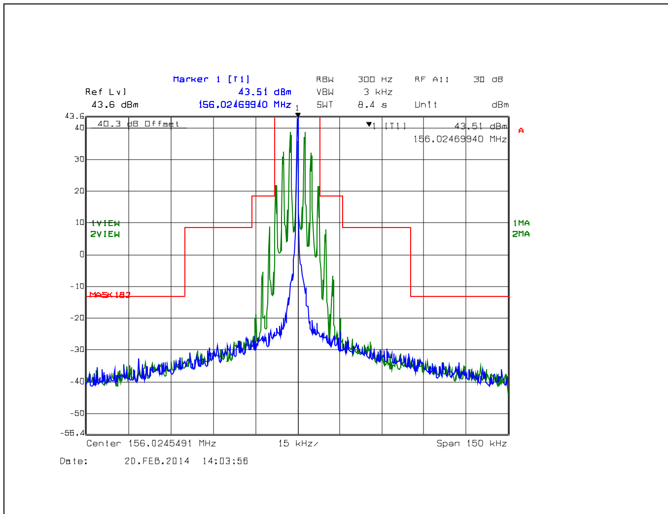
Plot 5.5.4.2.1. Emission Limitation for 156.025 MHz, 25 kHz Channel Spacing, High Power (25 W), G3E, 150 kHz Span
