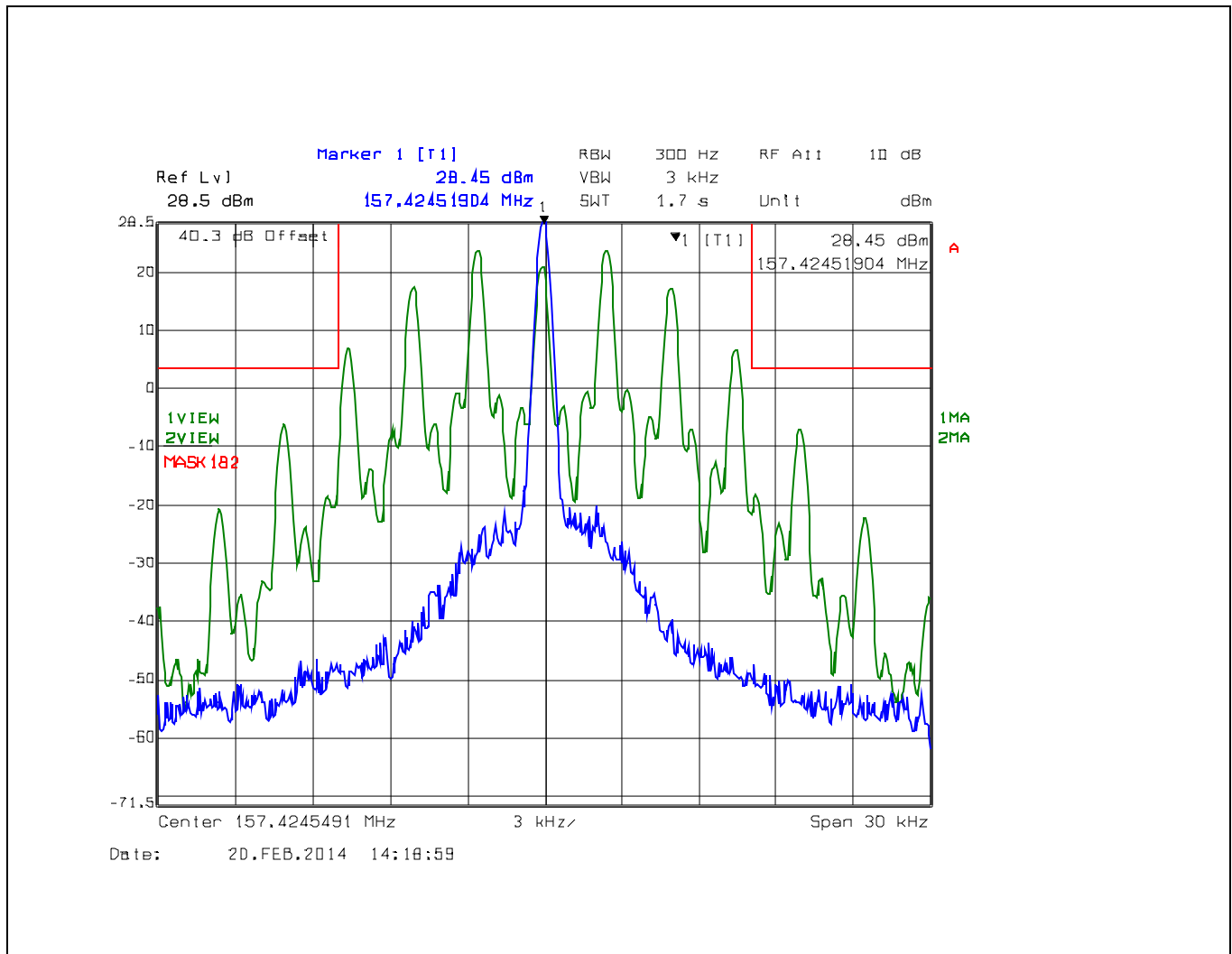
Plot 5.5.4.2.8. Emission Limitation for 157.425 MHz, 25 kHz Channel Spacing, Low Power (1 W), G3E, 30 kHz Span
