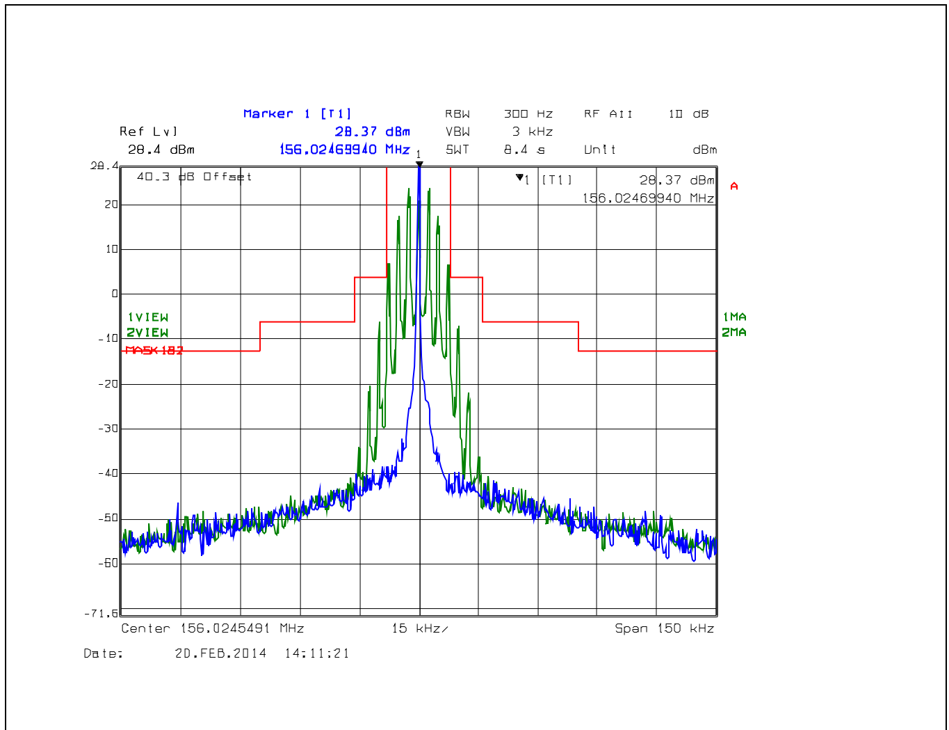
Plot 5.5.4.2.3. Emission Limitation for 156.025 MHz, 25 kHz Channel Spacing, Low Power (1 W), G3E, 150 kHz Span
