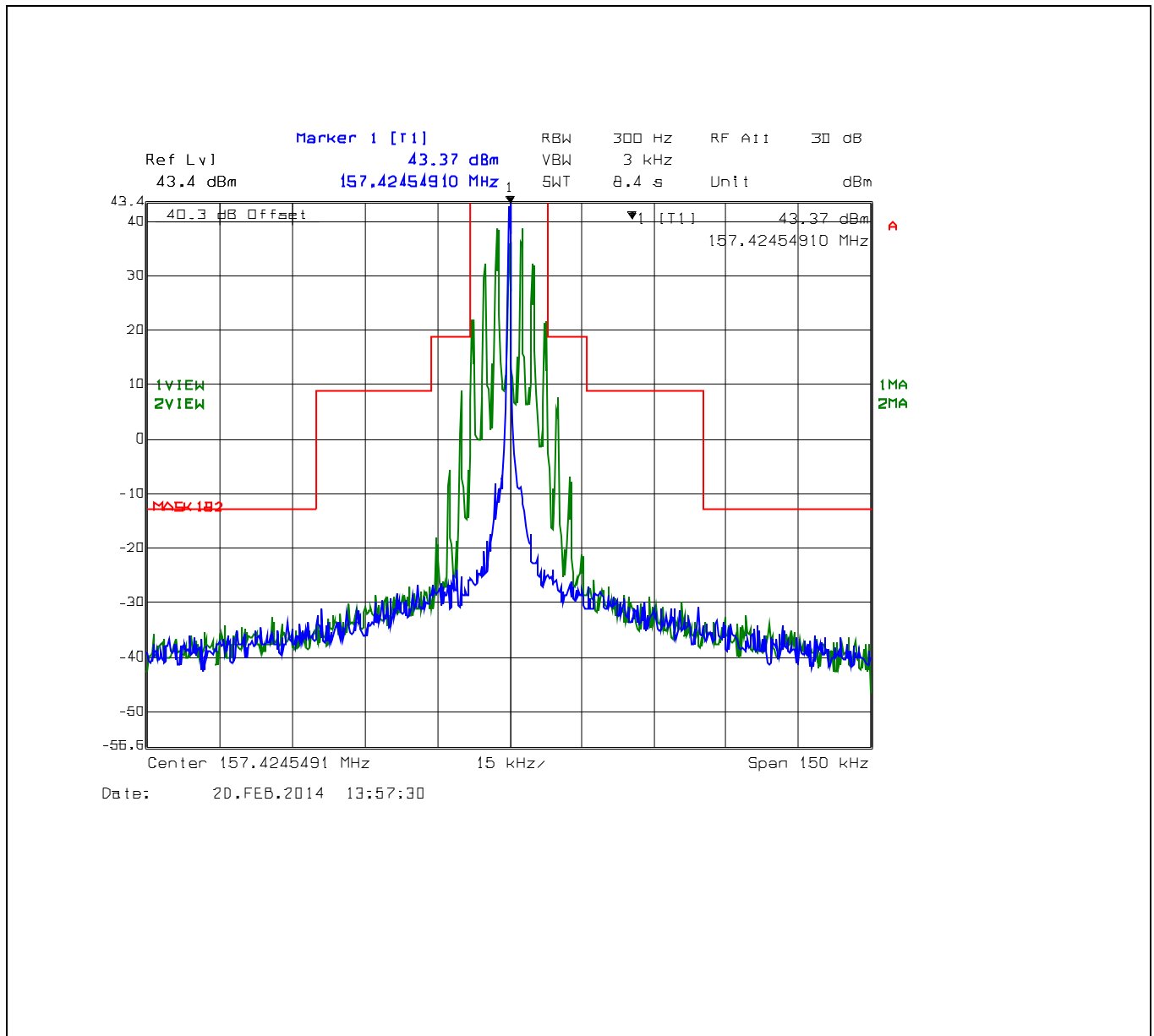
Plot 5.5.4.2.5. Emission Limitation for 157.425 MHz, 25 kHz Channel Spacing, High Power (25 W), G3E, 150 kHz Span
