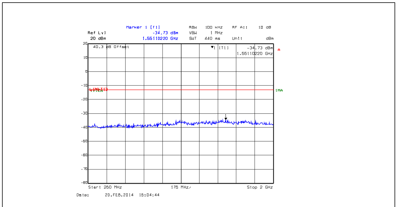
Plot 5.6.4.2. Spurious Emissions at Antenna Terminals, 156.025 MHz, 25 kHz Channel Spacing, 25 W, 250 MHz - 2 GHz
