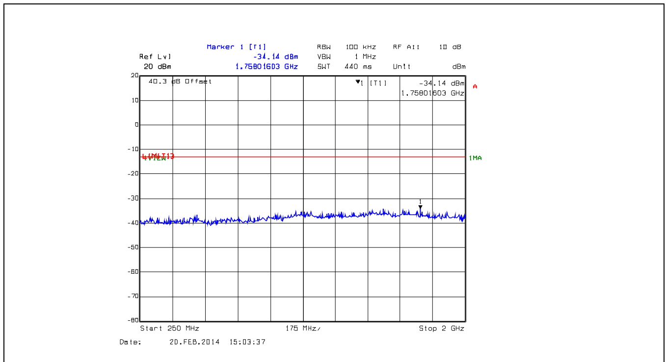
Plot 5.6.4.4. Spurious Emissions at Antenna Terminals, 156.025 MHz, 25 kHz Channel Spacing, 1 W, 250 MHz - 2 GHz
