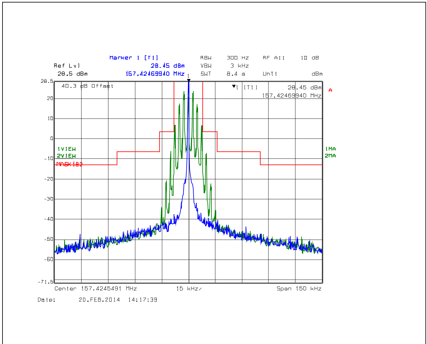
Plot 5.5.4.2.7. Emission Limitation for 157.425 MHz, 25 kHz Channel Spacing, Low Power (1 W), G3E, 150 kHz Span
