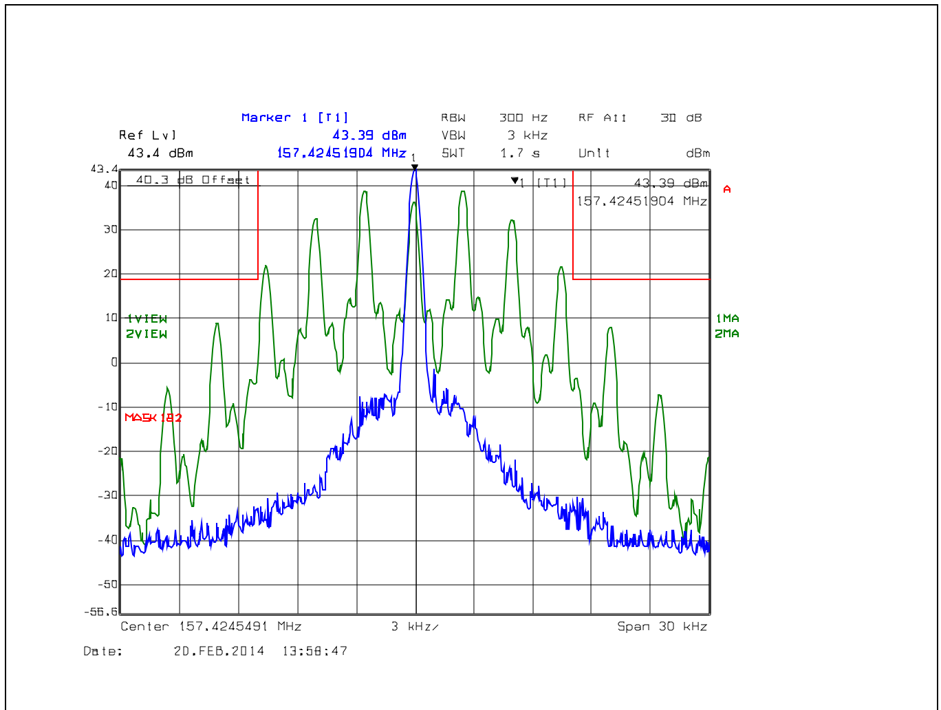
Plot 5.5.4.2.6. Emission Limitation for 157.425 MHz, 25 kHz Channel Spacing High Power (25 W), G3E, 30 kHz Span
