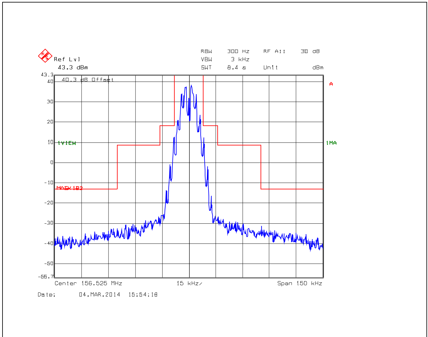
Plot 5.5.4.2.9. Emission Limitation for 156.525 MHz, 25 kHz Channel Spacing, High Power (25 W), DSC-G2B
