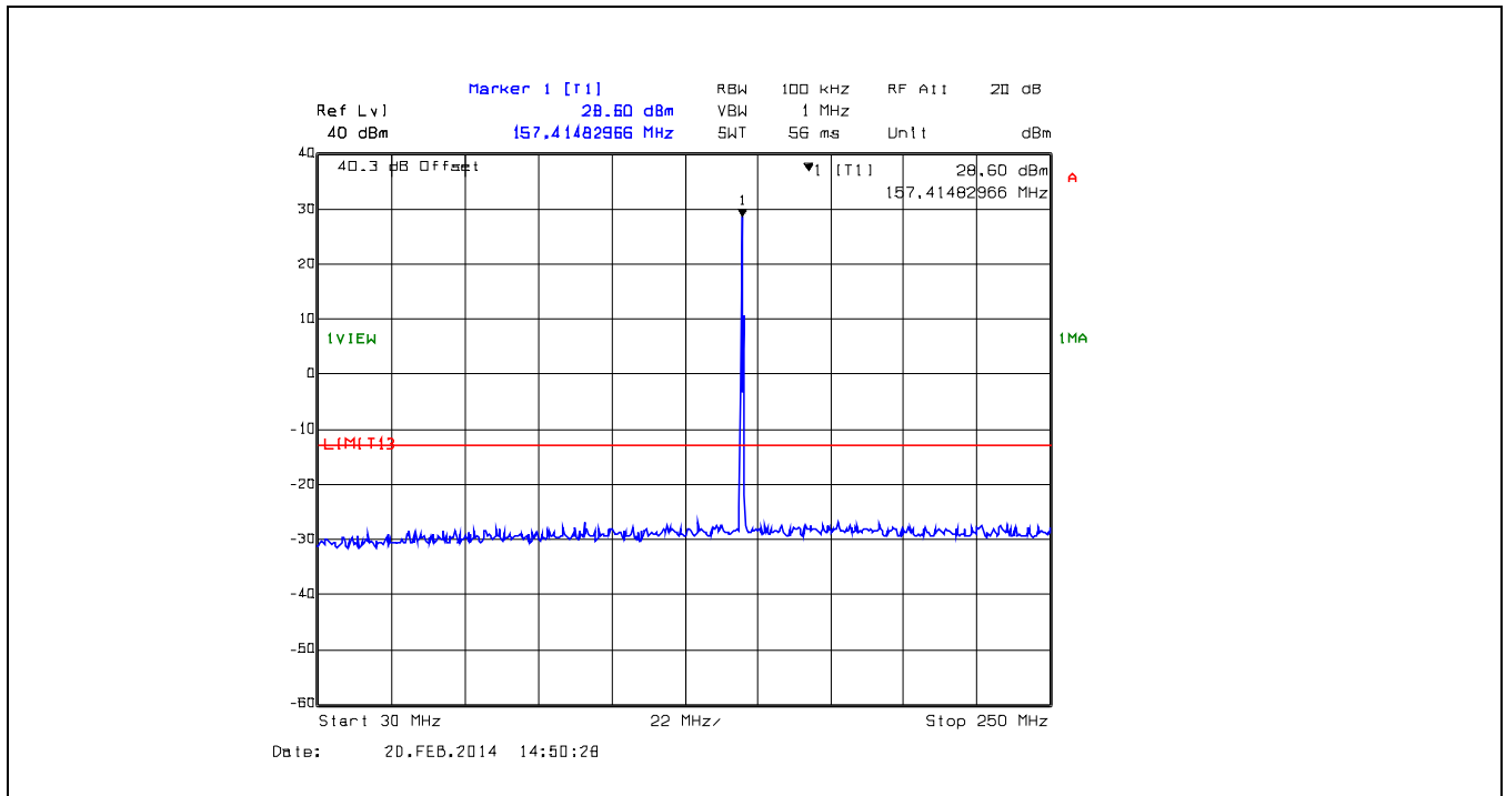
Plot 5.6.4.7. Spurious Emissions at Antenna Terminals, 157.425 MHz, 25 kHz Channel Spacing, 1 W, 30 MHz - 250 MHz
