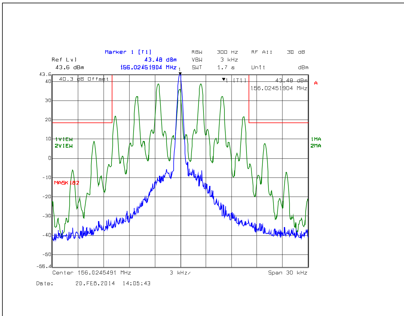
Plot 5.5.4.2.2. Emission Limitation for 156.025 MHz, 25 kHz Channel Spacing, High Power (25 W), G3E, 30 kHz Span
