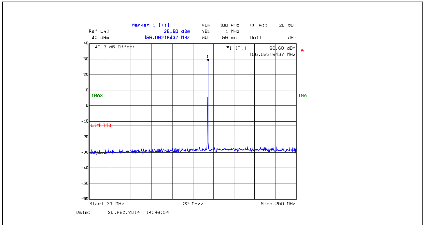
Plot 5.6.4.3. Spurious Emissions at Antenna Terminals, 156.025 MHz, 25 kHz Channel Spacing, 1 W, 30 MHz - 250 MHz
