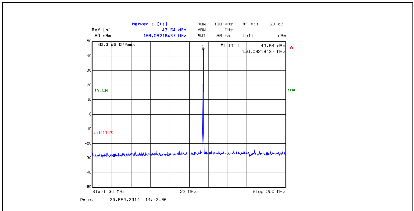
Plot 5.6.4.1. Spurious Emissions at Antenna Terminals, 156.025 MHz, 25 kHz Channel Spacing, 25 W, 30 MHz - 250 MHz
