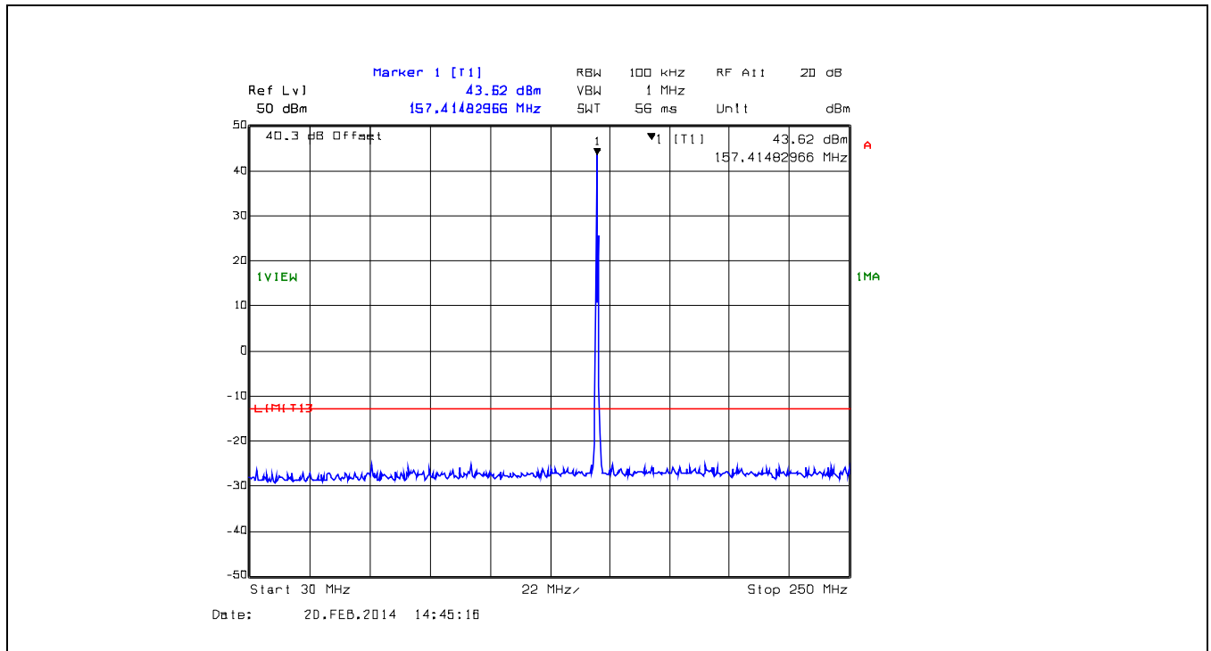
Plot 5.6.4.5. Spurious Emissions at Antenna Terminals, 157.425 MHz, 25 kHz Channel Spacing, 25 W, 30 MHz - 250 MHz
