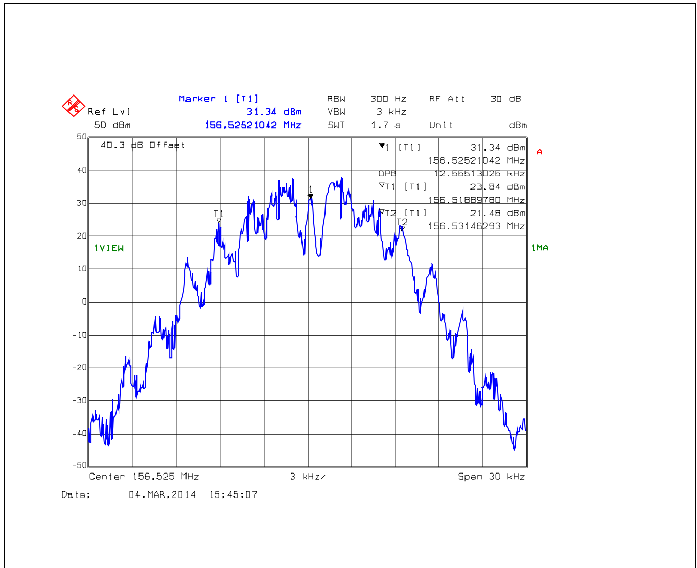
Plot 5.5.4.1.3. Occupied Bandwidth for 156.525 MHz, 25 kHz Channel Spacing, High Power (25 W), DSC-G2B
