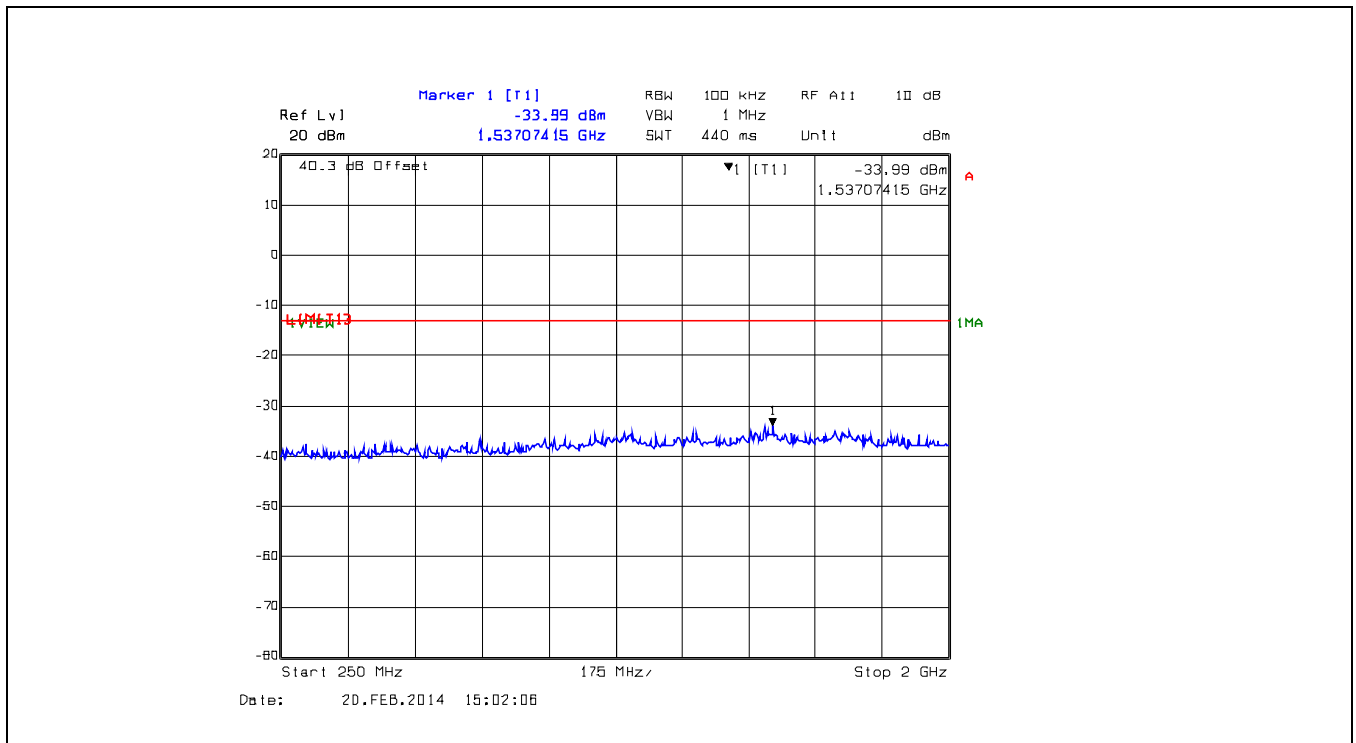
Plot 5.6.4.8. Spurious Emissions at Antenna Terminals, 157.425 MHz, 25 kHz Channel Spacing, 1 W, 250 MHz - 2 GHz
