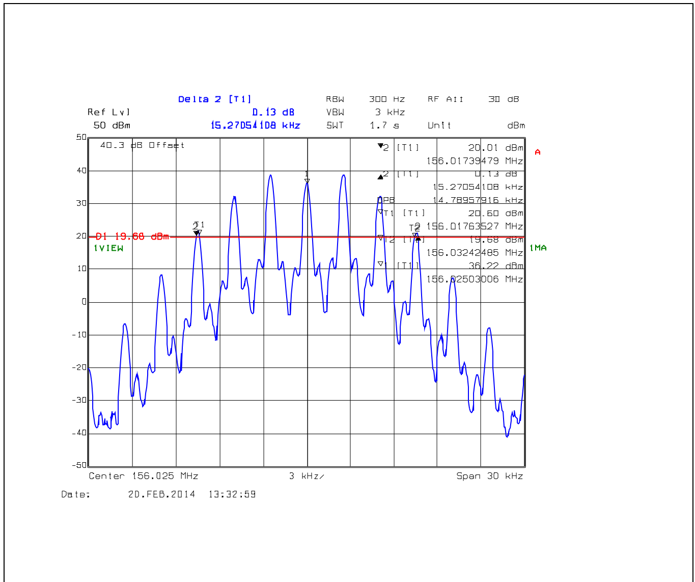
Plot 5.5.4.1.1. Occupied Bandwidth for 156.025 MHz, 25 kHz Channel Spacing, High Power (25 W), G3E
