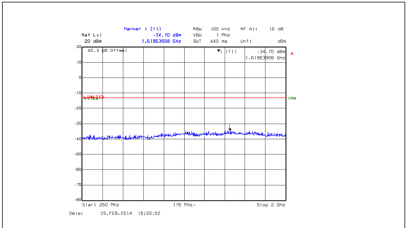
Plot 5.6.4.6. Spurious Emissions at Antenna Terminals, 157.425 MHz, 25 kHz Channel Spacing, 25 W, 250 MHz - 2 GHz
