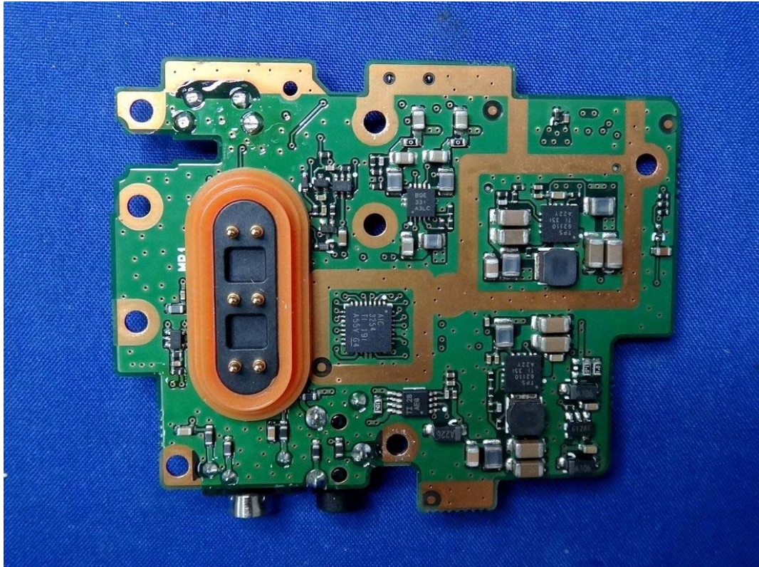
(28) EUT Photo
