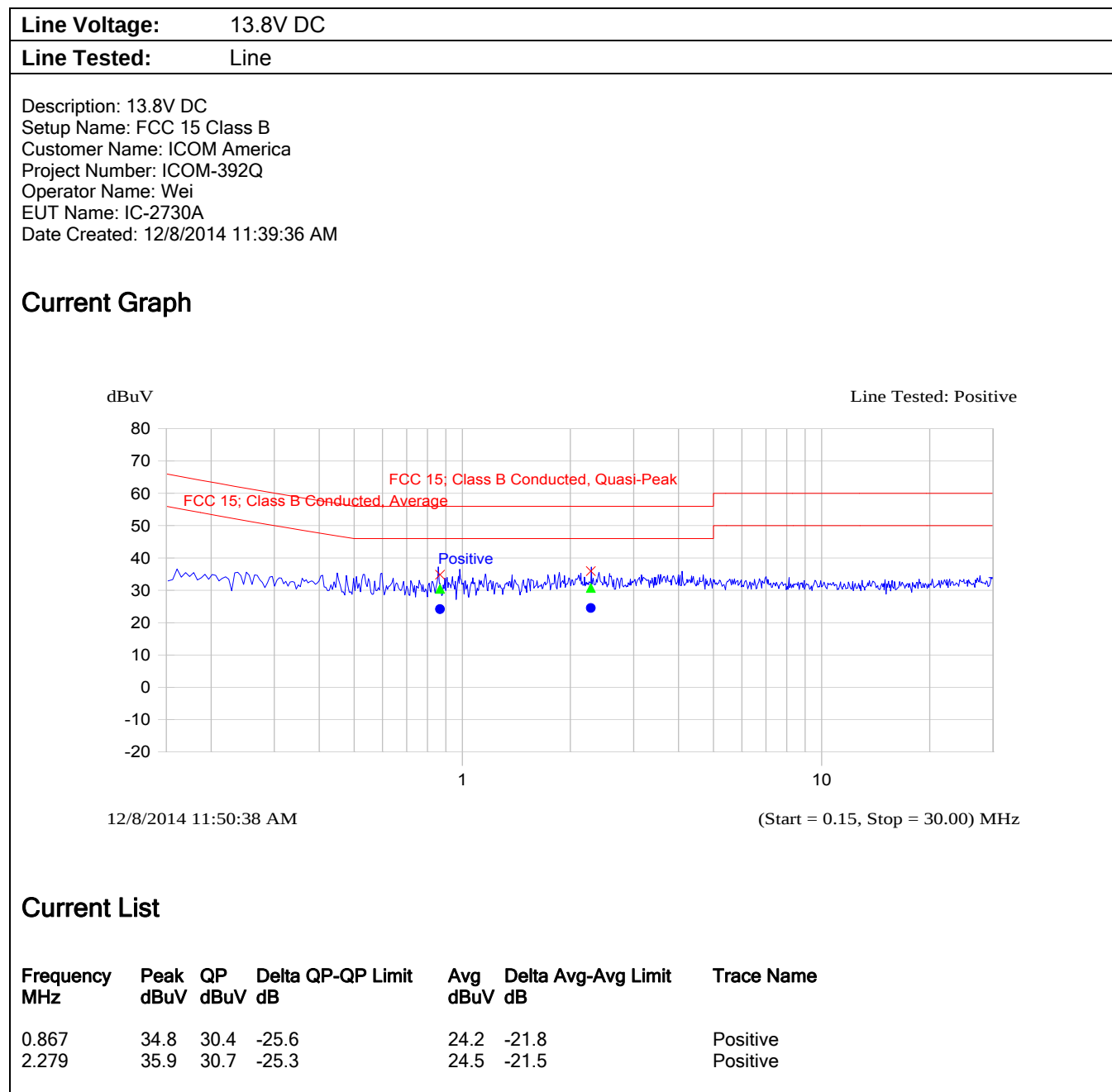
Plot 1: Power Line Conducted Emissions
