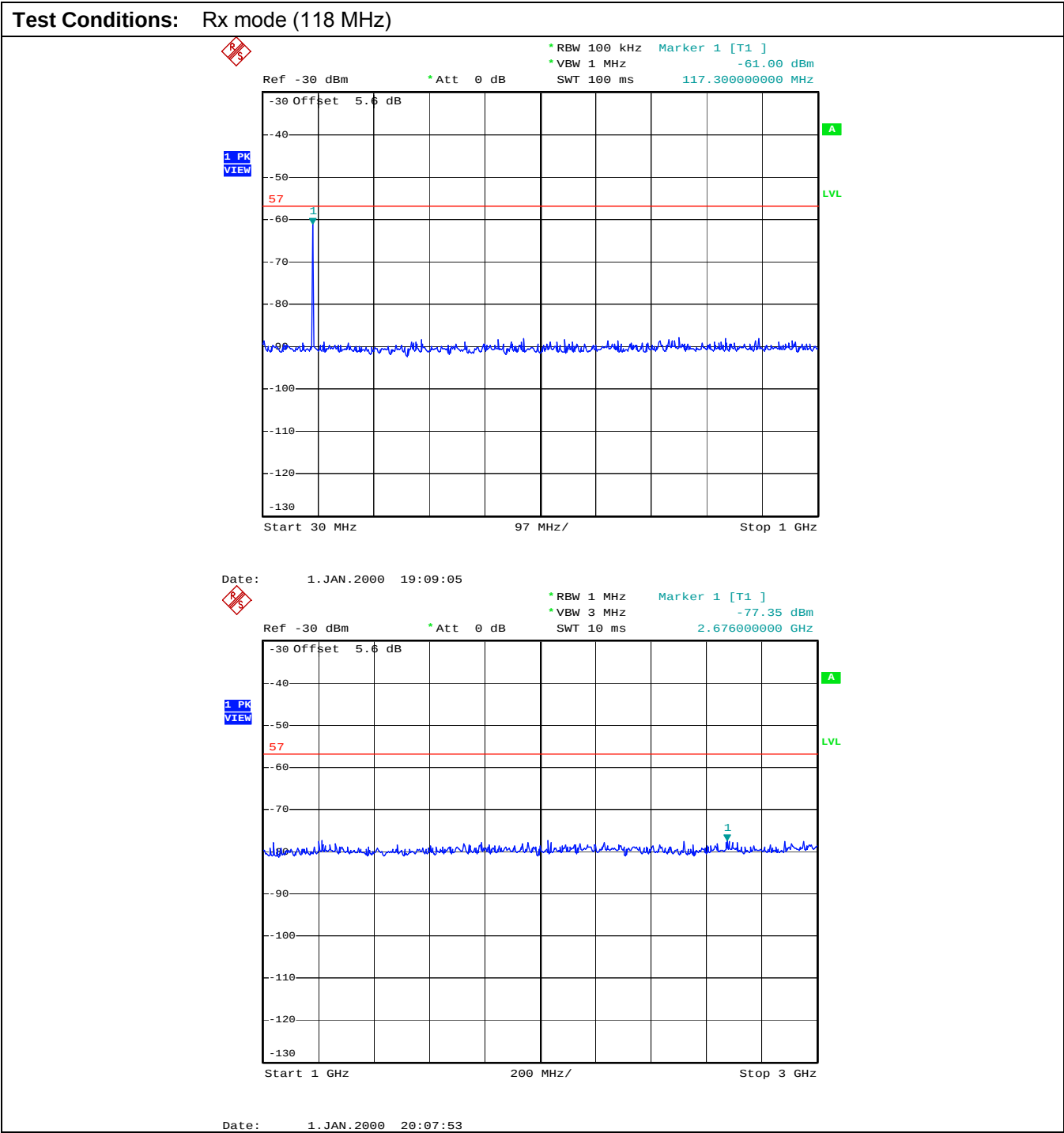
Plot 3: Conducted Receiver Spurious Emissions, 30 MHz – 3.0 GHz
