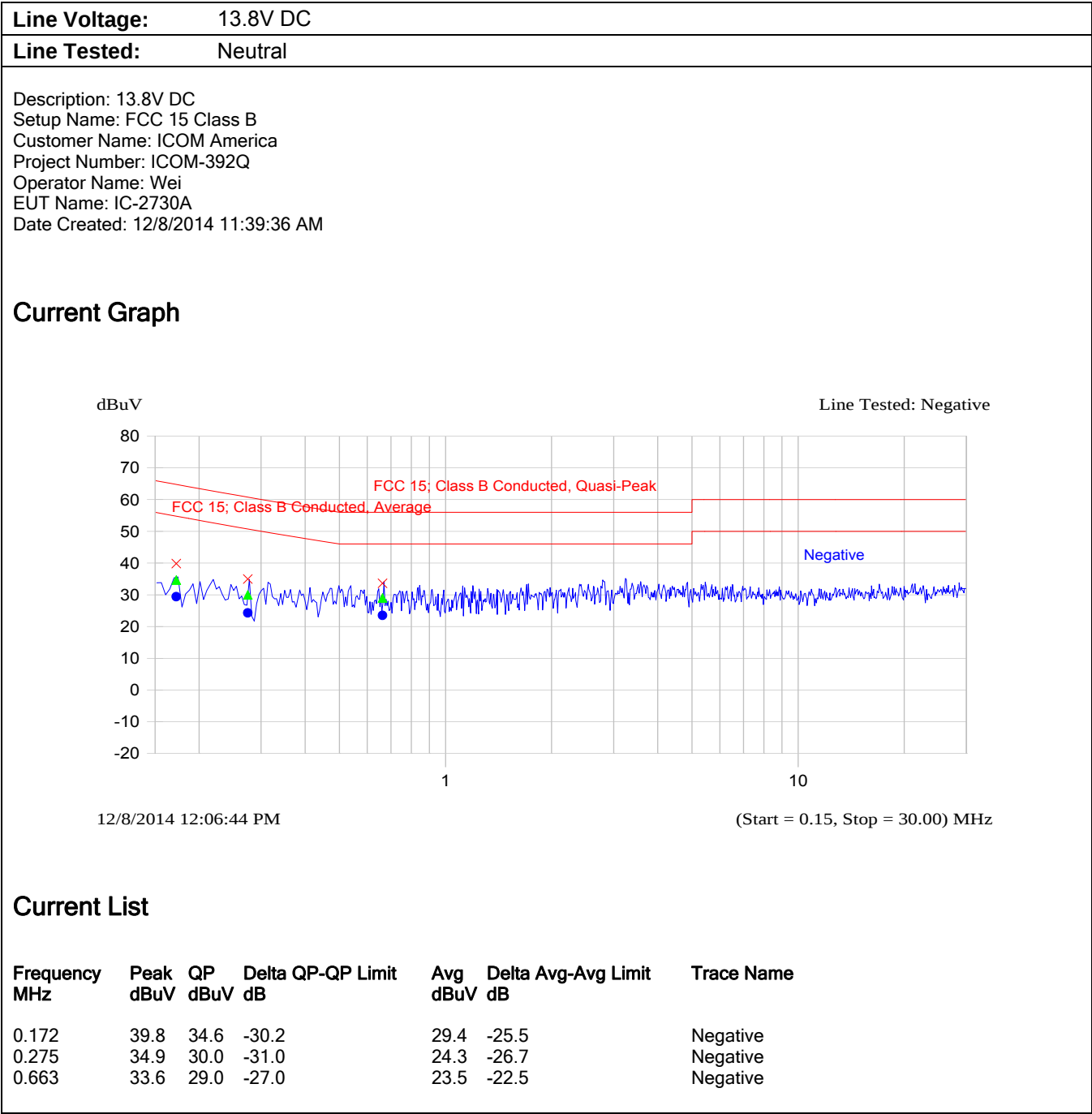
Plot 2: Power Line Conducted Emissions
