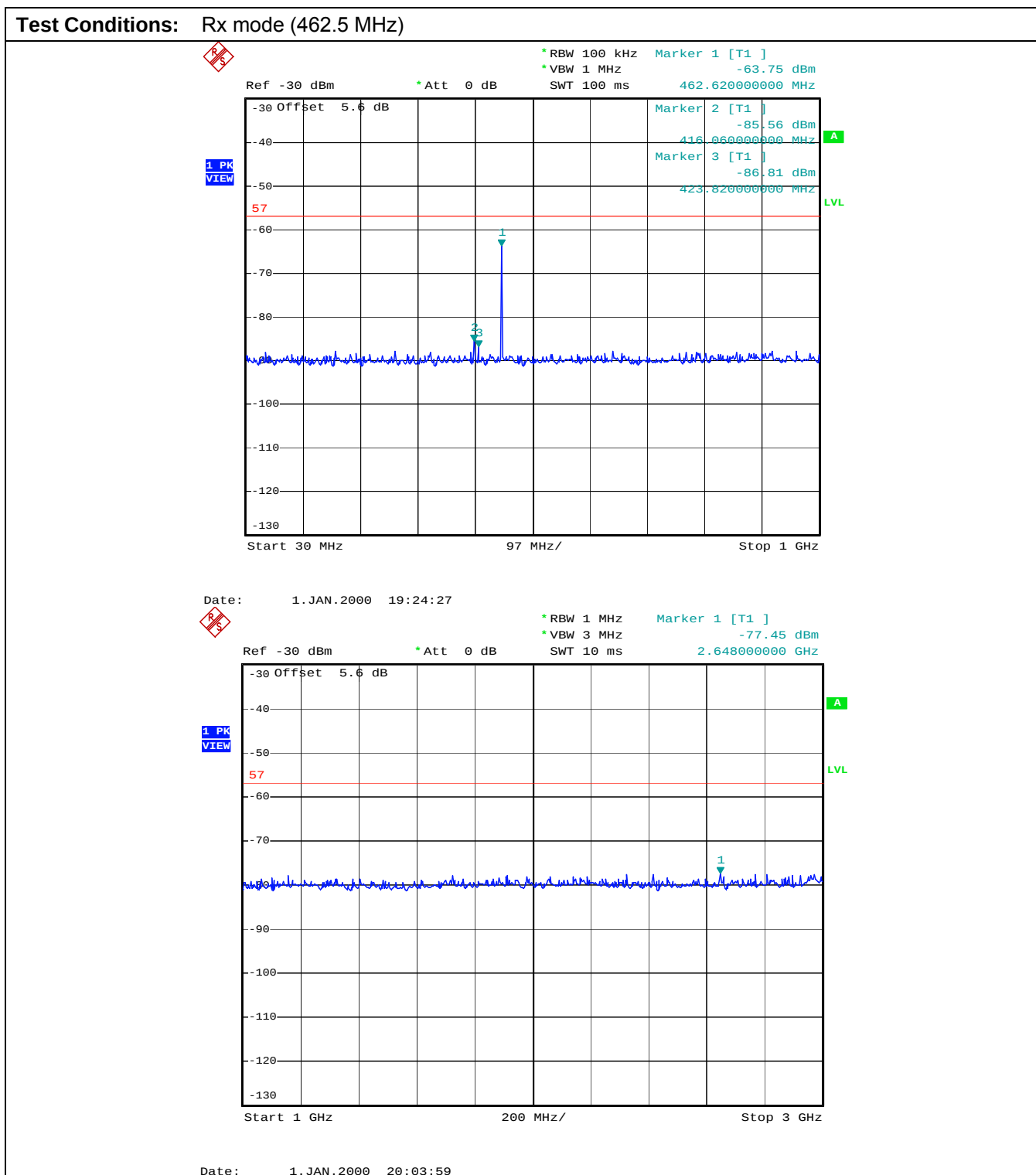
Plot 7: Conducted Receiver Spurious Emissions, 30 MHz – 3.0 GHz
