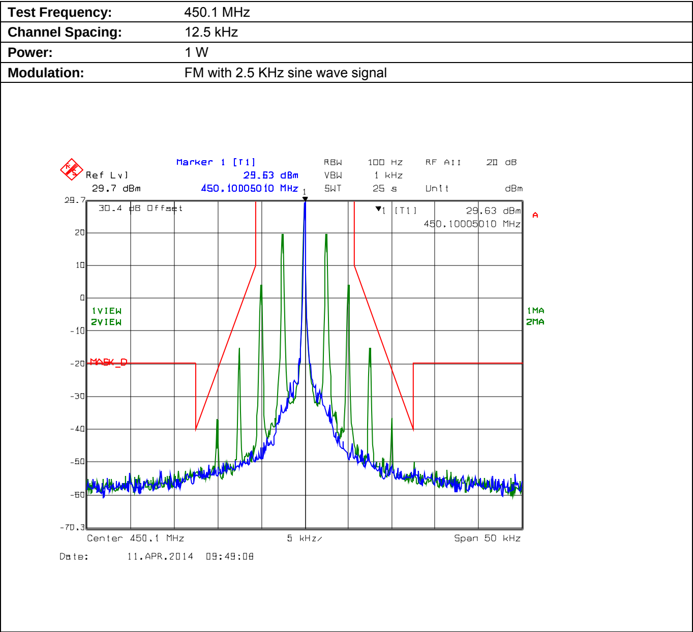
Plot 5.8.4.2.5. Emission Mask D, Low Power
