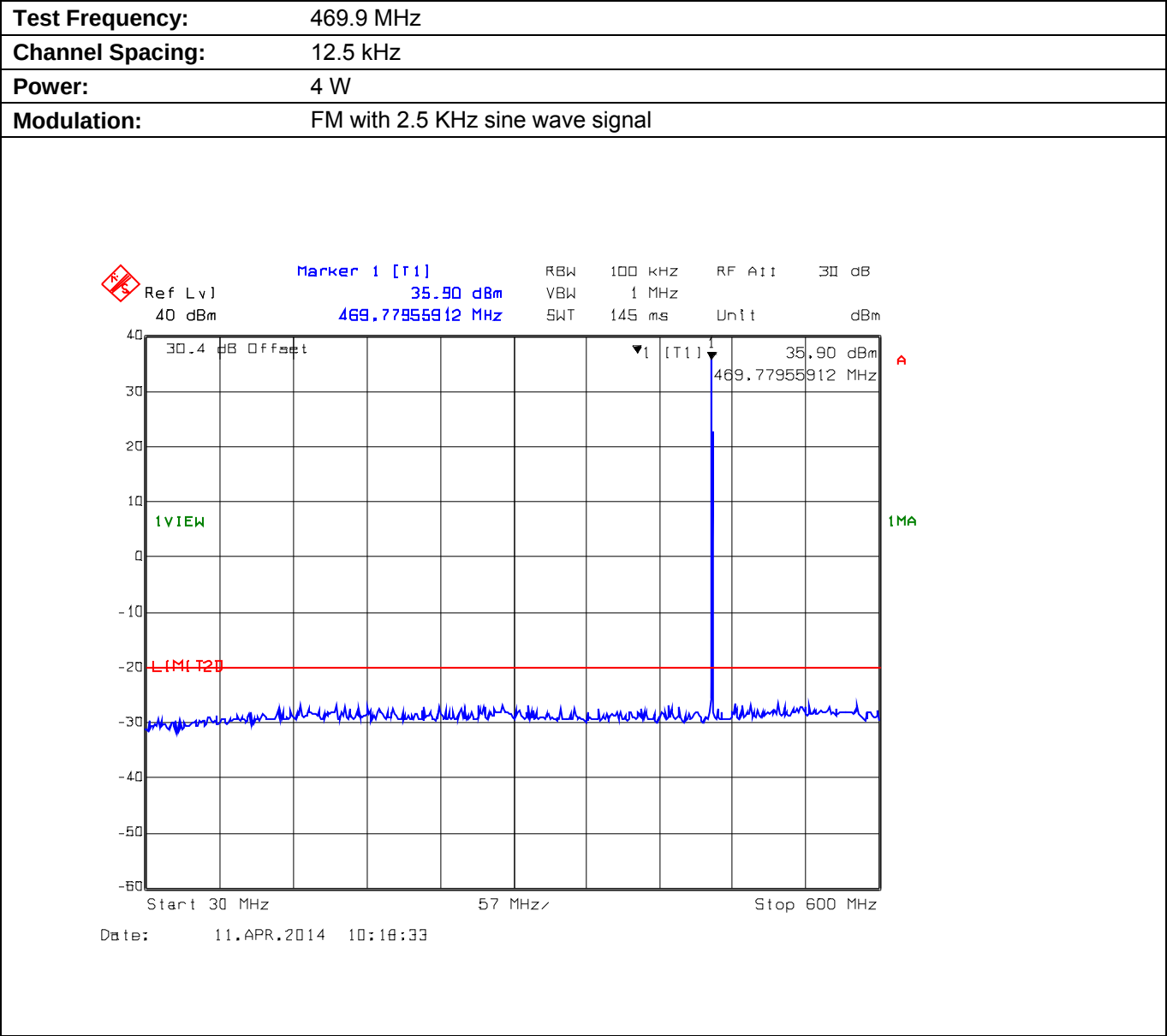
Plot 5.9.4.3.1. Conducted Transmitter Spurious Emissions for 469.9 MHz, High Power, 30 MHz - 600 MHz
