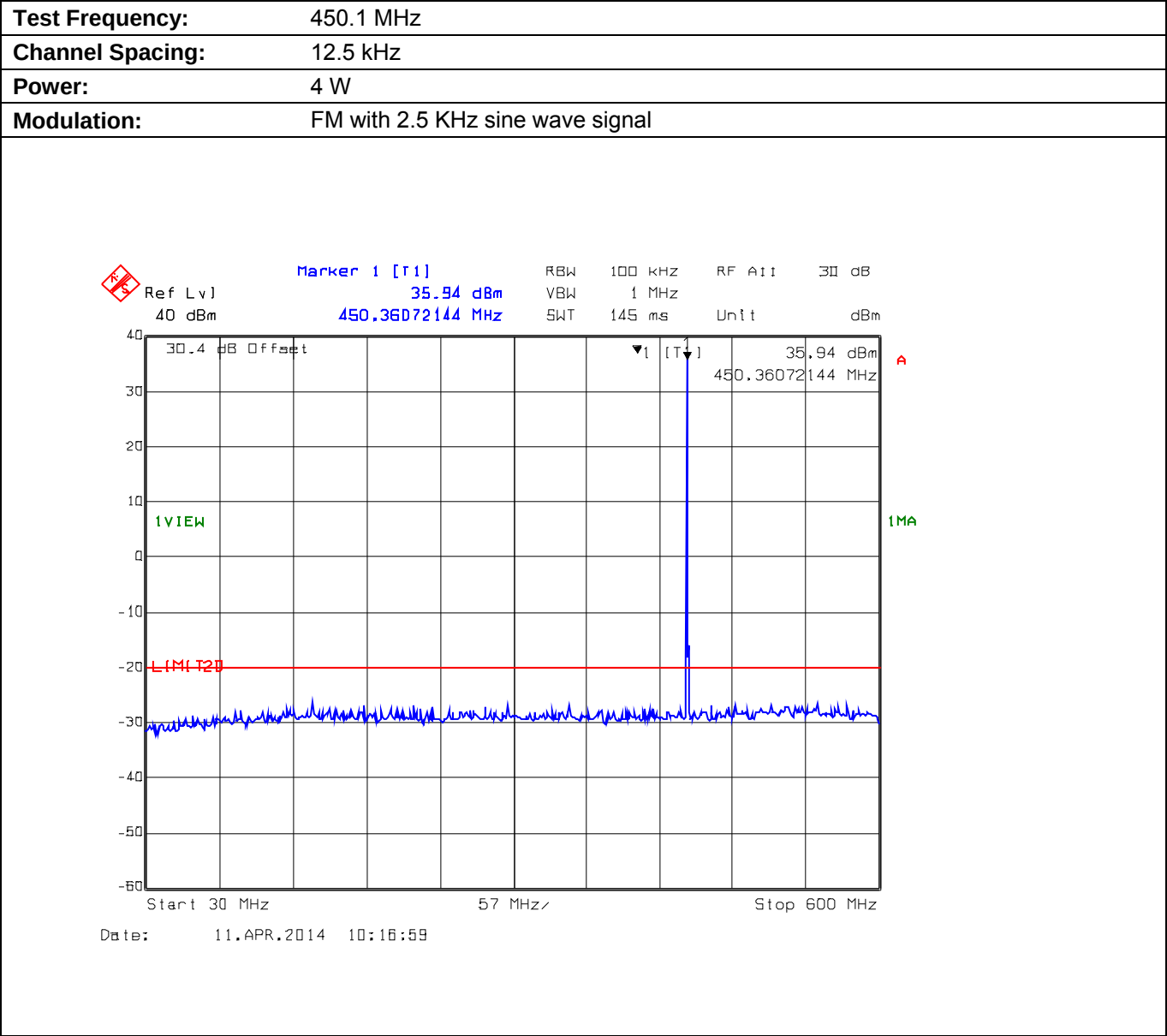
Plot 5.9.4.2.1. Conducted Transmitter Spurious Emissions for 450.1 MHz, High Power, 30 MHz - 600 MHz
