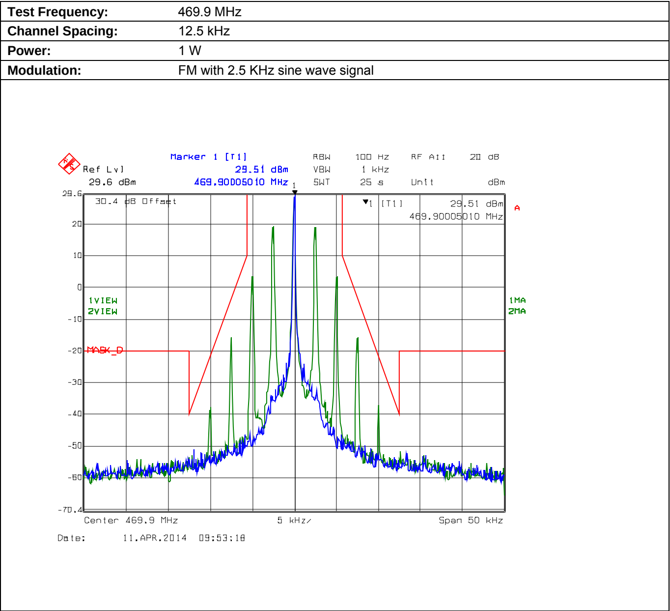
Plot 5.8.4.2.6. Emission Mask D, Low Power
