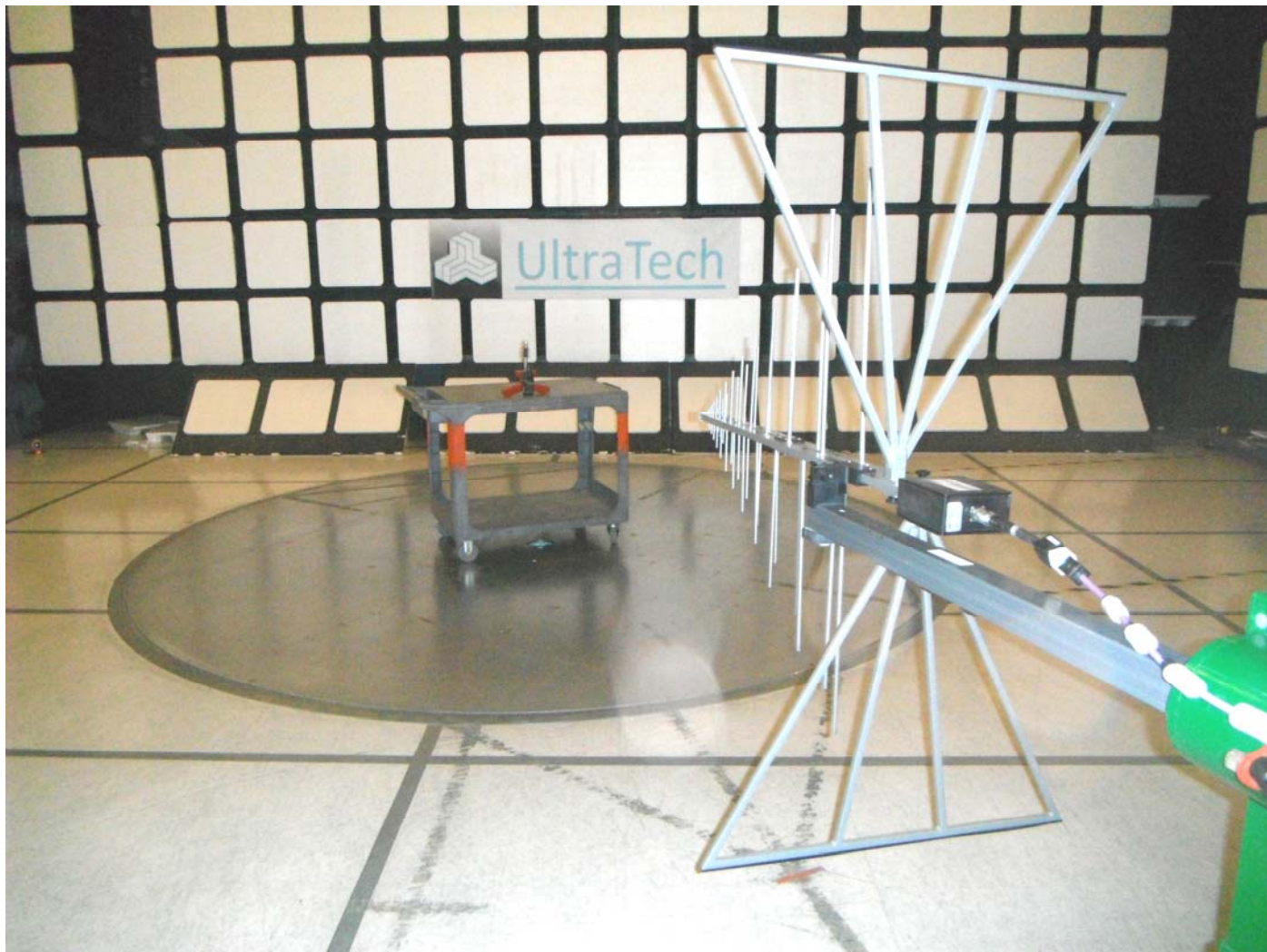
Plot #4: Tx Radiated Emission Test Setup
