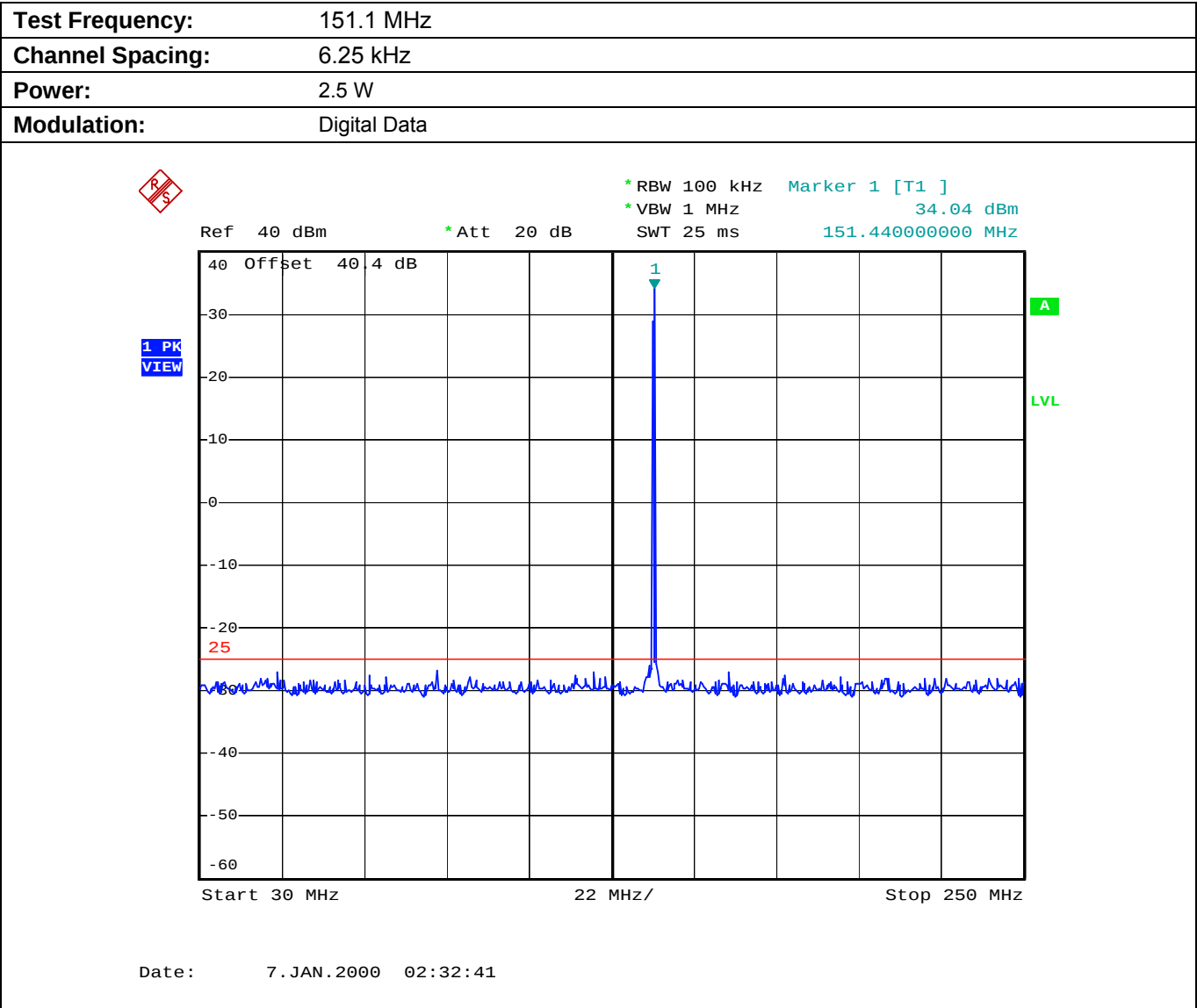
Plot 5.8.4.2.3. Conducted Transmitter Spurious Emissions for 151.1 MHz, Low Power, 30 MHz - 250 MHz
