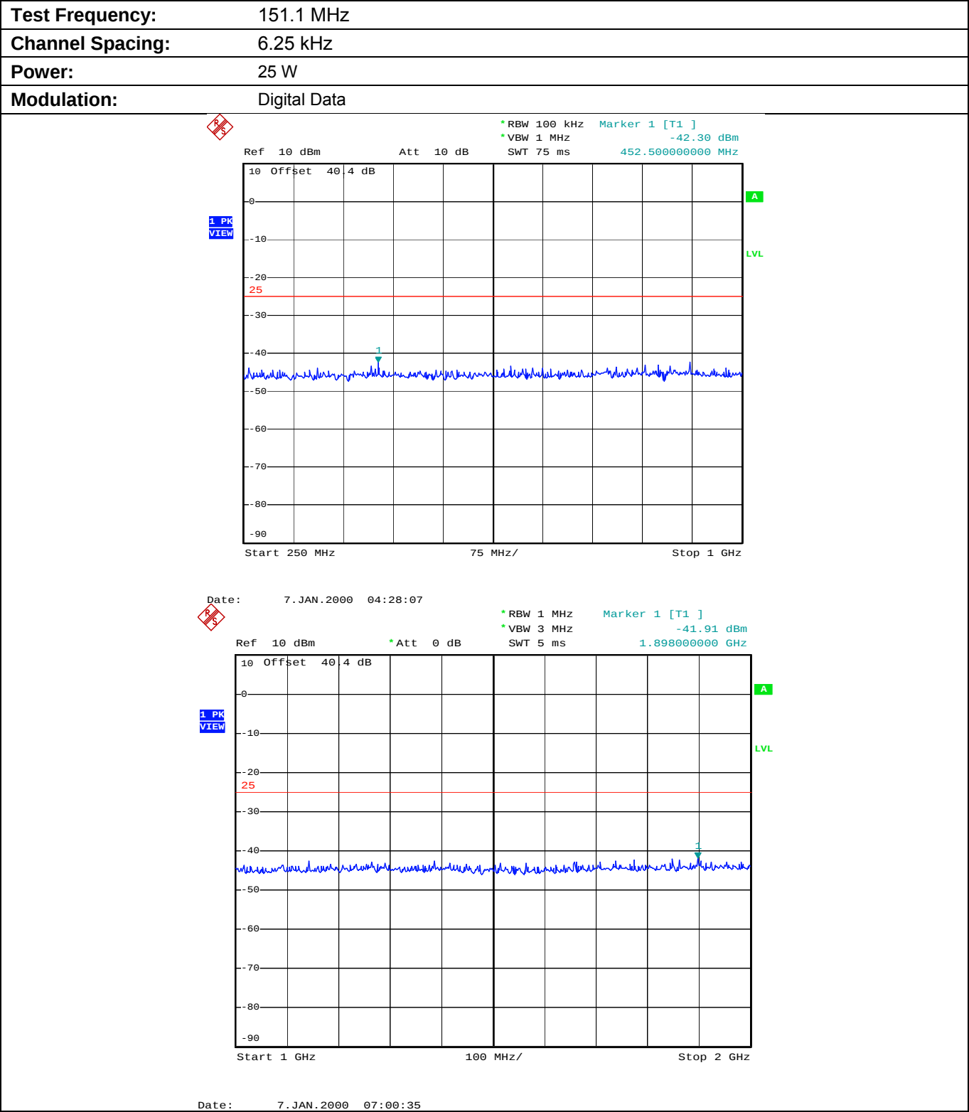
Plot 5.8.4.2.2. Conducted Transmitter Spurious Emissions for 151.1 MHz, High Power, 250 MHz - 2 GHz
