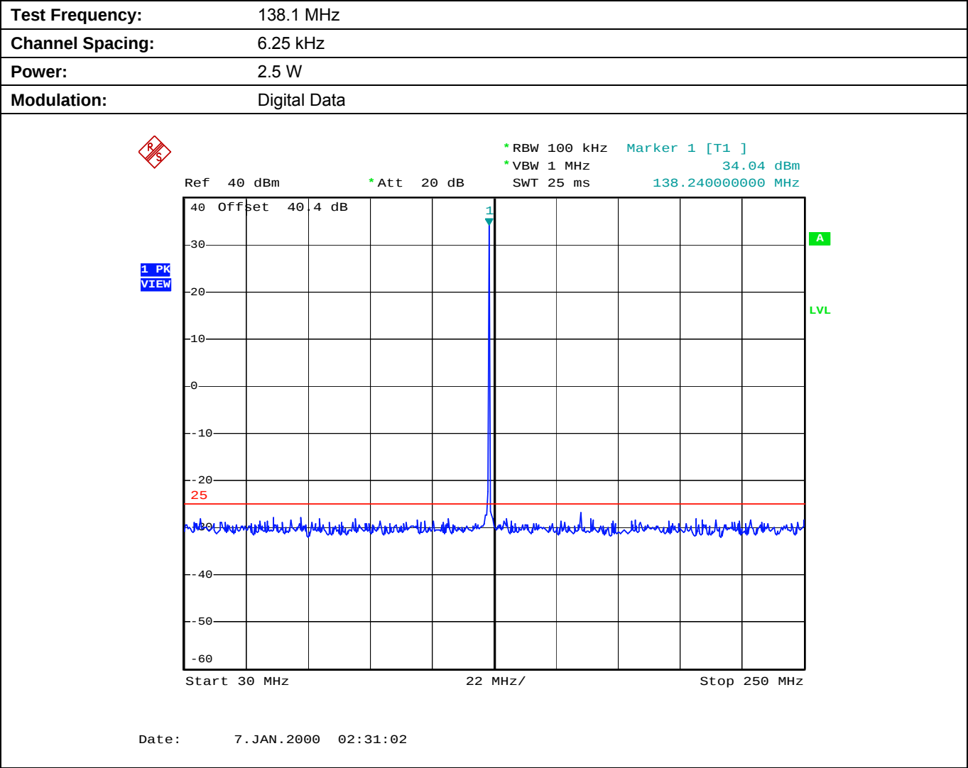
Plot 5.8.4.1.3. Conducted Transmitter Spurious Emissions for 138.1 MHz, Low Power, 30 MHz - 250 MHz
