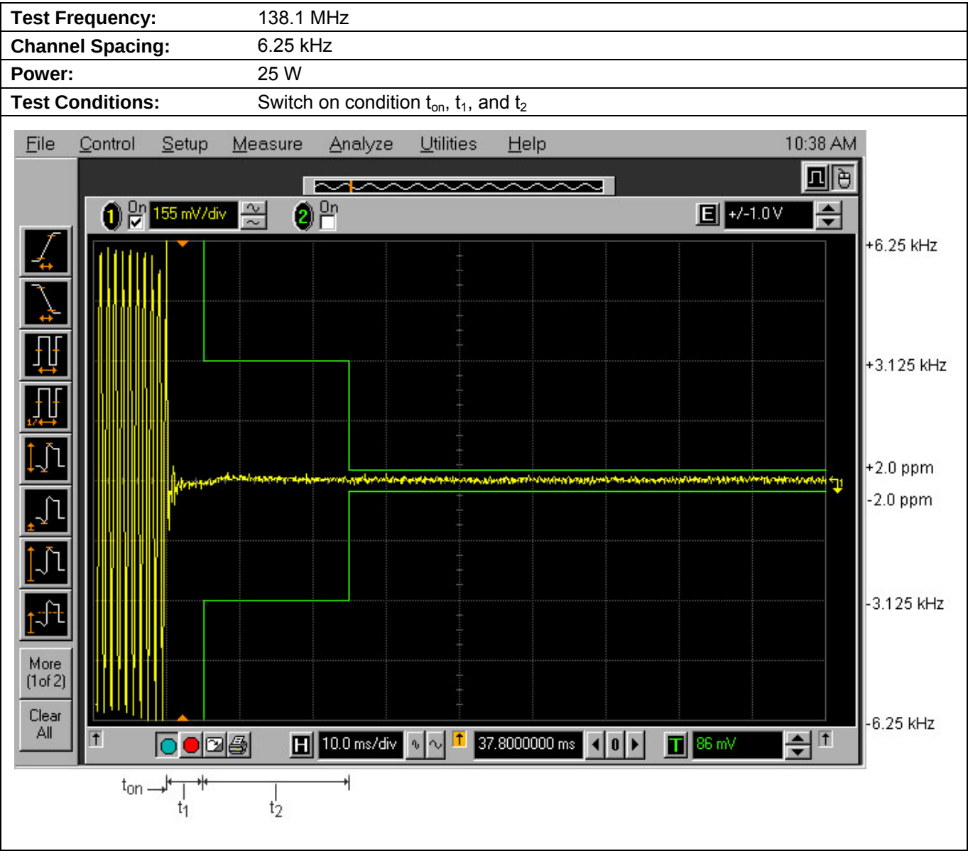
Plot 5.11.4.3. Transient Frequency Behavior for 6.25 kHz Channel Spacing
