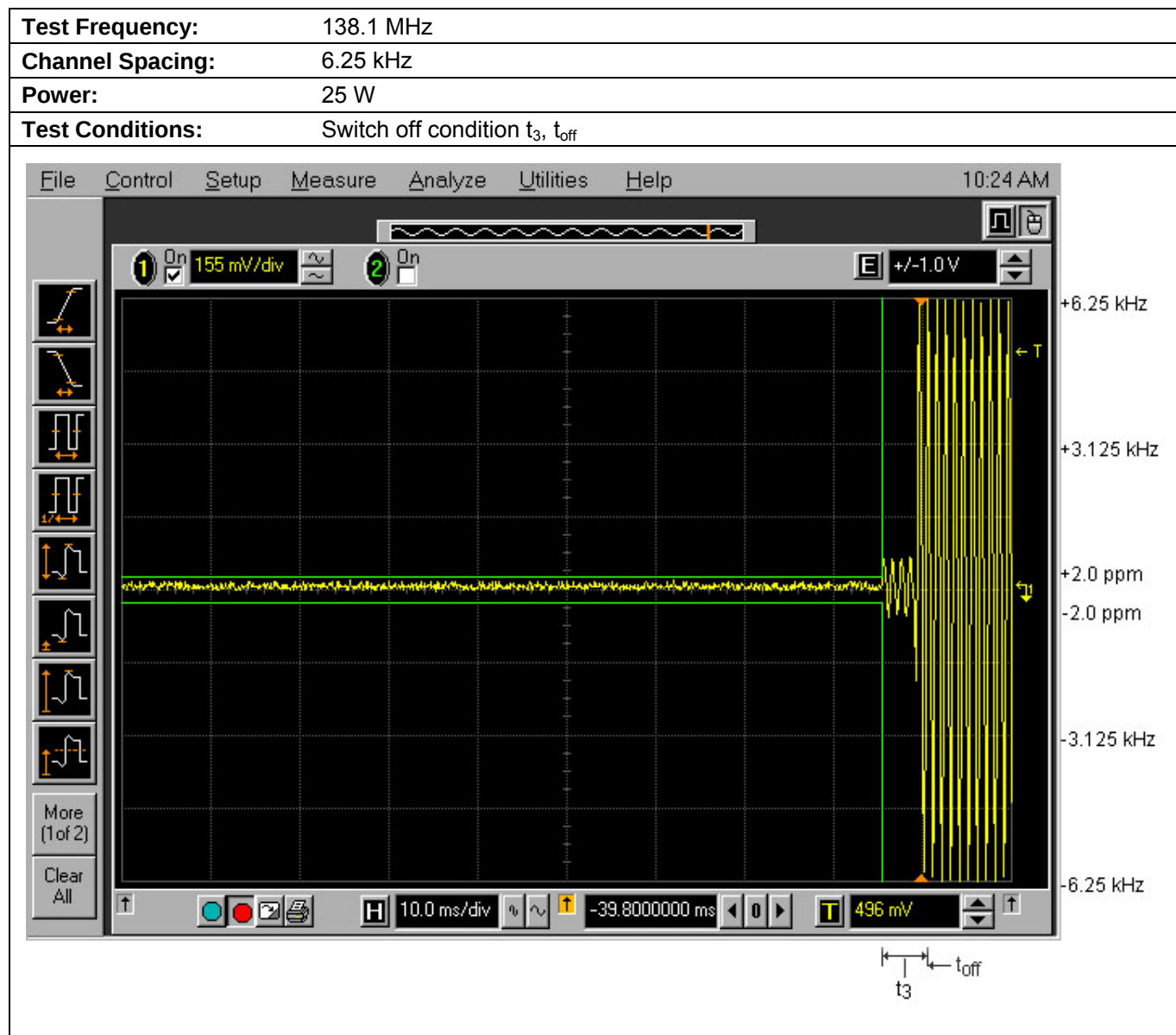
Plot 5.11.4.4. Transient Frequency Behavior for 6.25 kHz Channel Spacing
