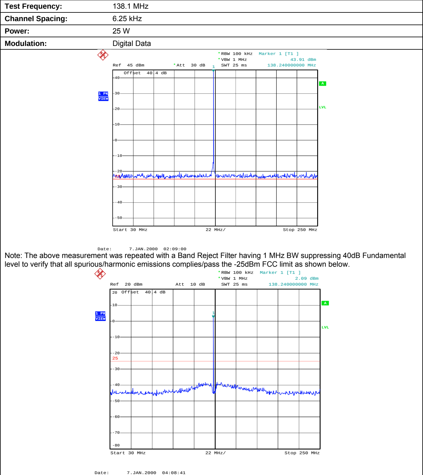
Plot 5.8.4.1.1. Conducted Transmitter Spurious Emissions for 138.1 MHz, High Power, 30 MHz - 250 MHz
