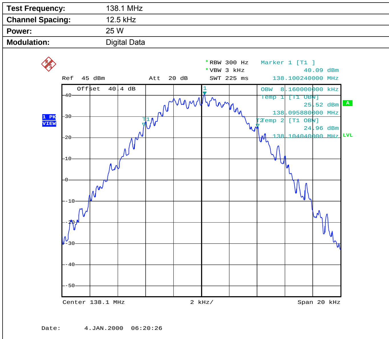
Plot 5.7.4.1.1. Occupied Bandwidth
