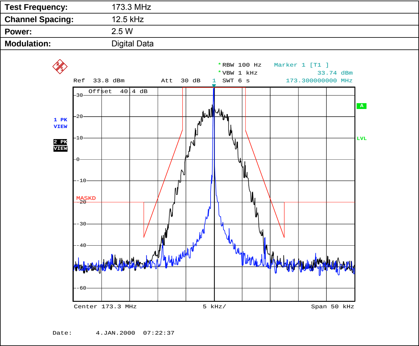
Plot 5.7.4.2.6. Emission Mask D, Low Power
