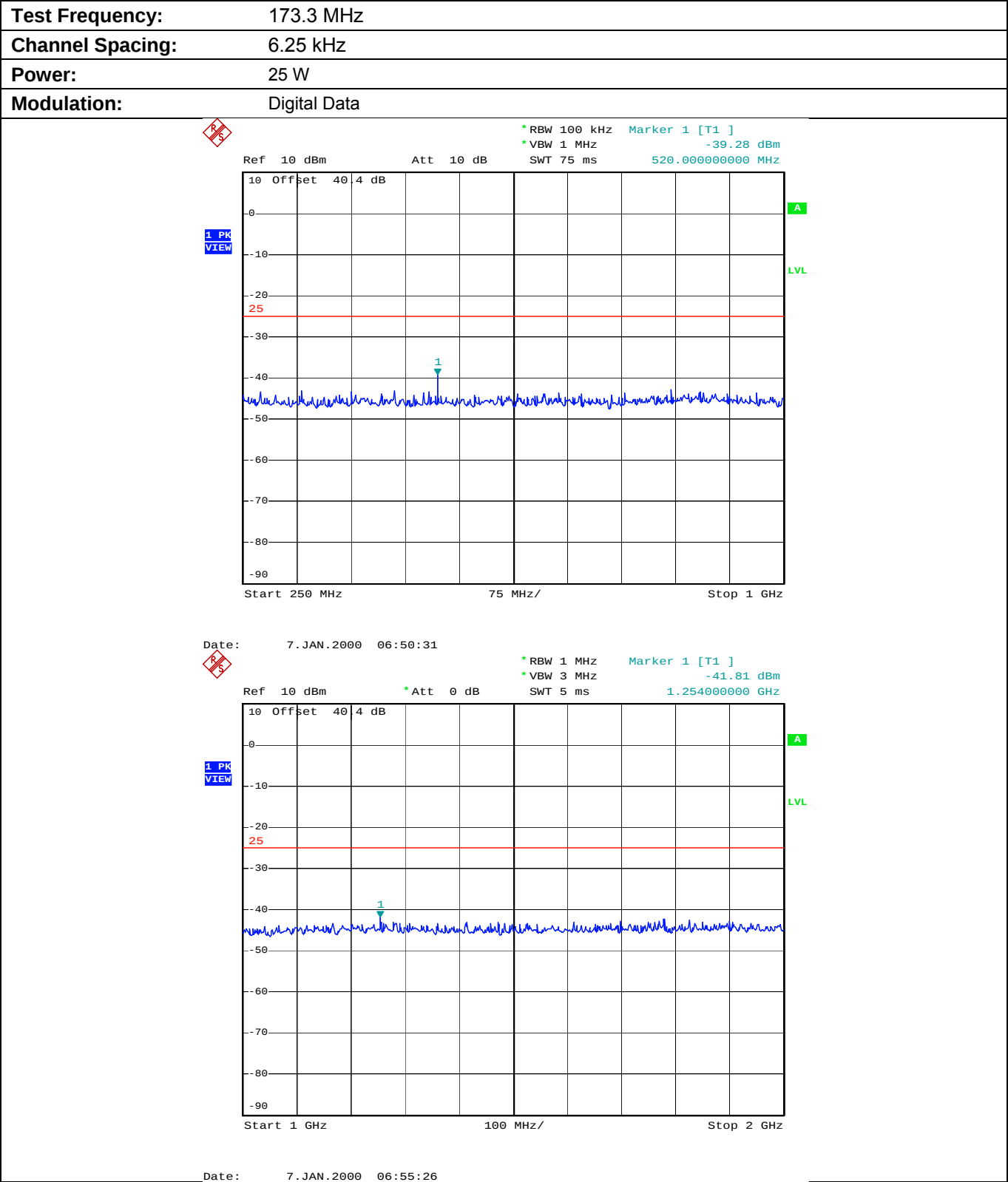
Plot 5.8.4.3.2. Conducted Transmitter Spurious Emissions for 173.3 MHz, High Power, 250 MHz - 2 GHz
