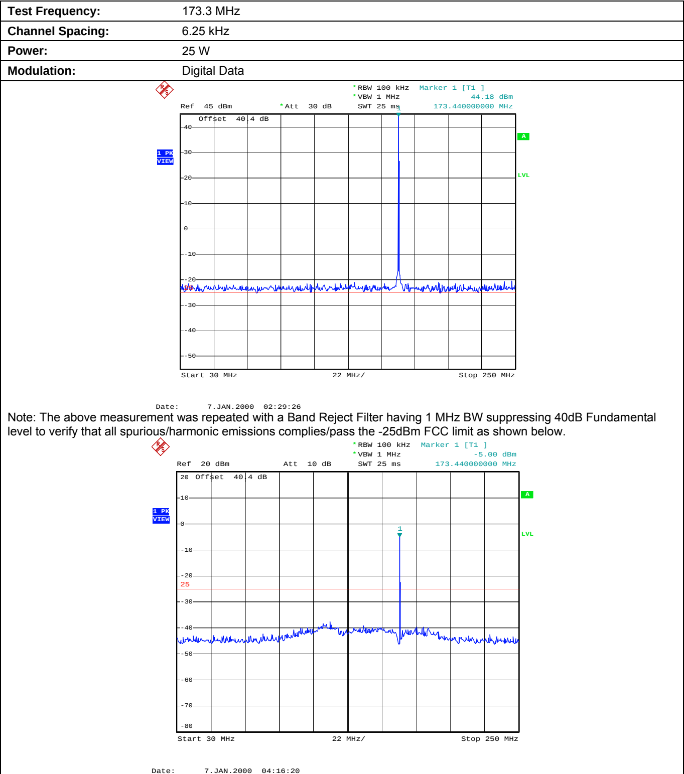
Plot 5.8.4.3.1. Conducted Transmitter Spurious Emissions for 173.3 MHz, High Power, 30 MHz - 250 MHz
