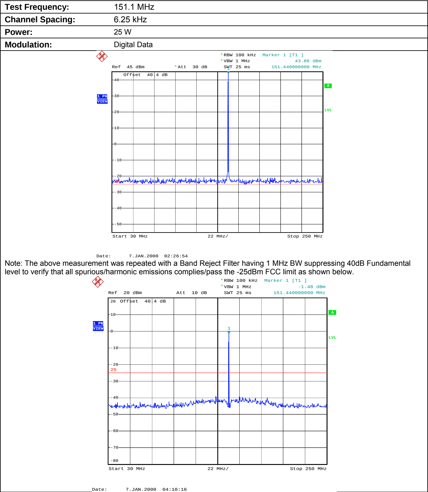
Plot 5.8.4.2.1. Conducted Transmitter Spurious Emissions for 151.1 MHz, High Power, 30 MHz - 250 MHz
