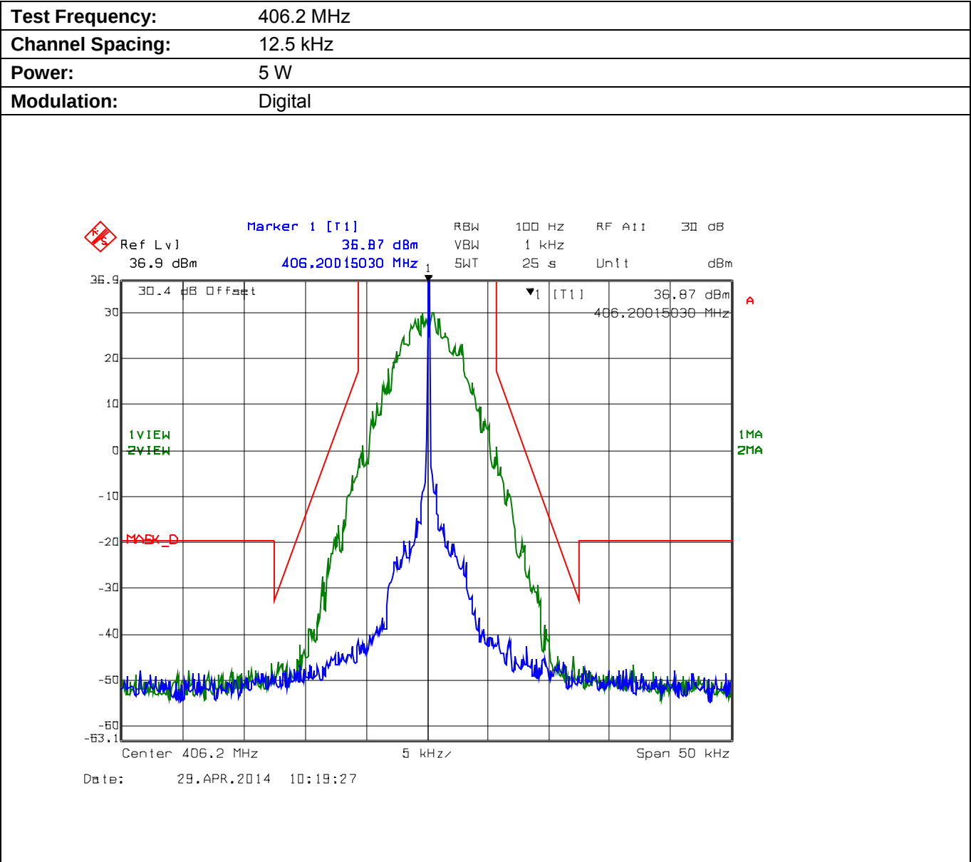
Plot 5.8.4.2.7. Emission Mask D, High Power
