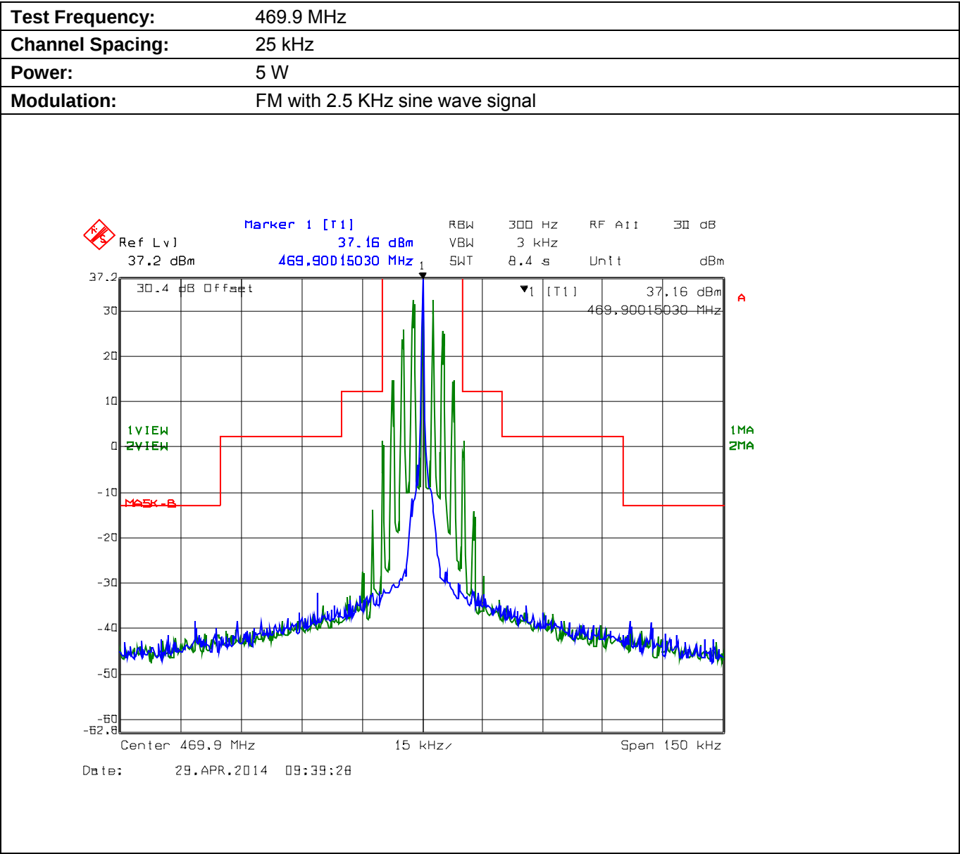
Plot 5.8.4.3.3. Emission Mask B, High Power
