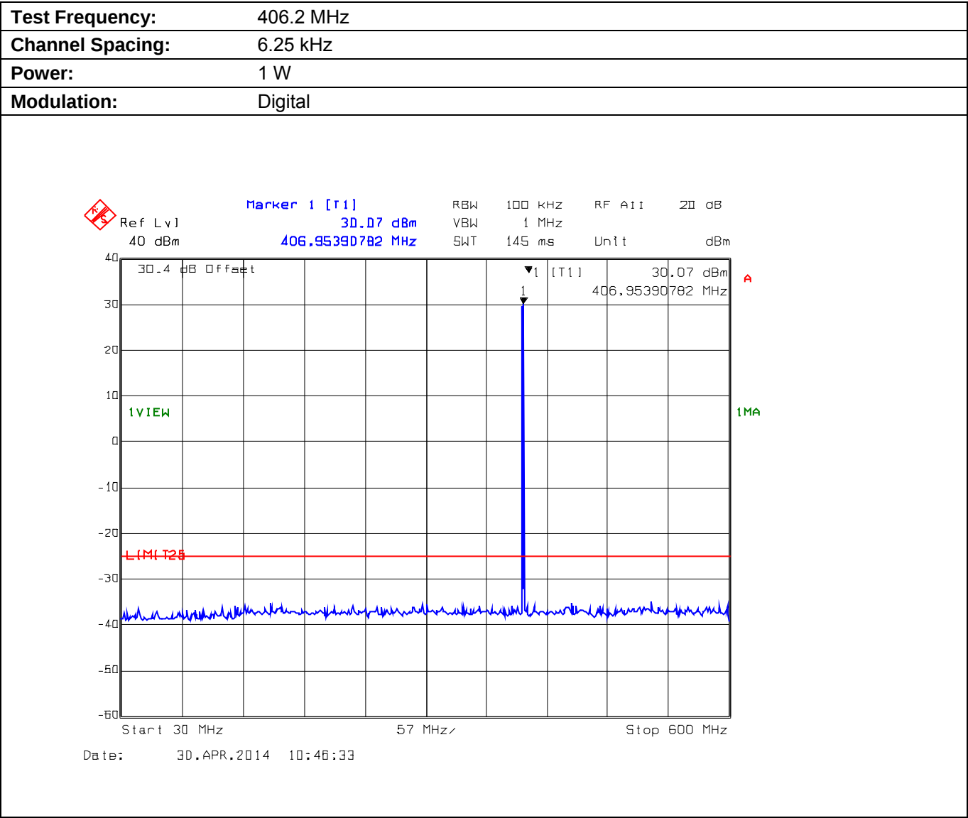
Plot 5.9.4.1.3. Conducted Transmitter Spurious Emissions for 406.2 MHz, Low Power, 30 MHz - 600 MHz
