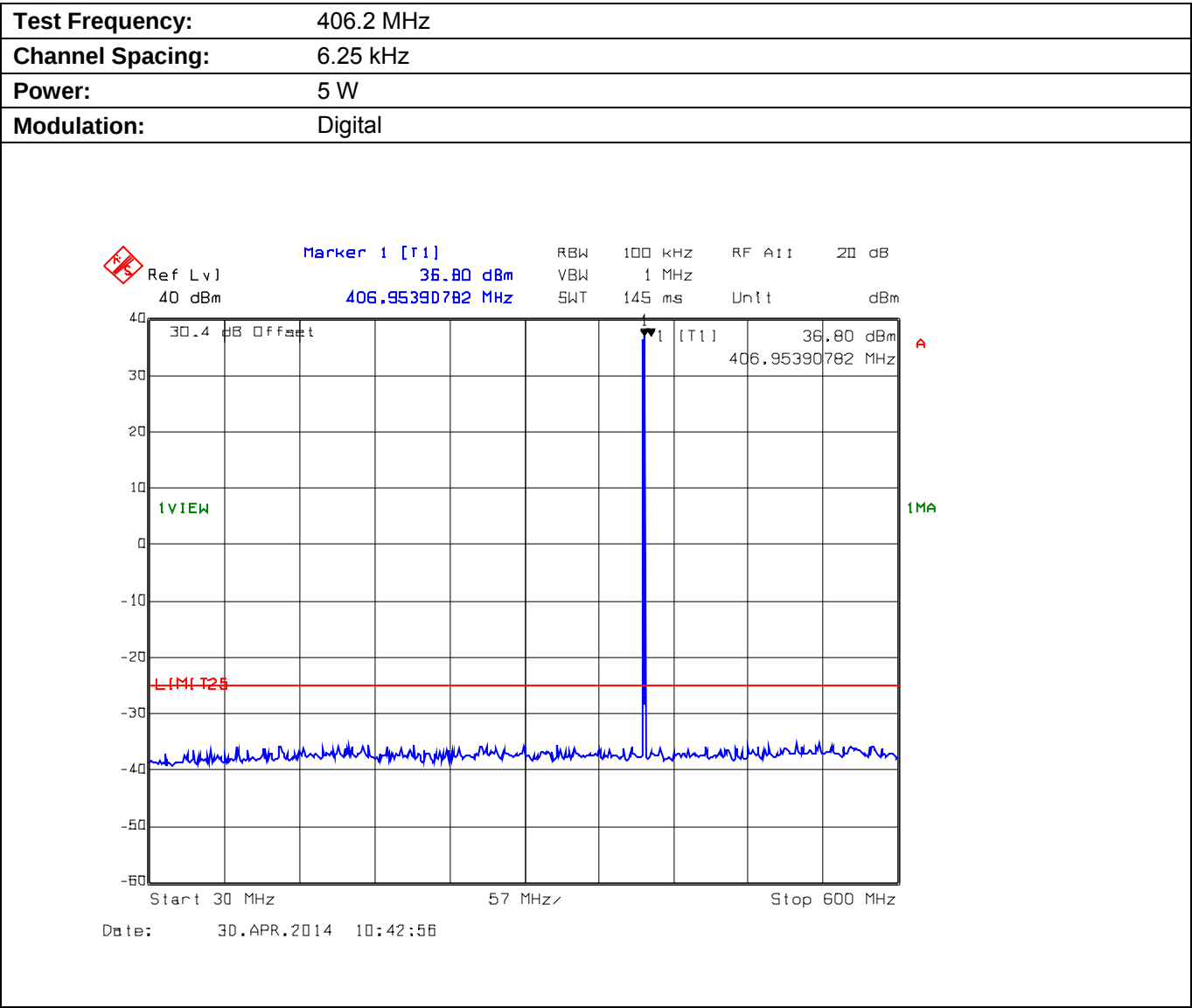
Plot 5.9.4.1.1. Conducted Transmitter Spurious Emissions for 406.2 MHz, High Power, 30 MHz - 600 MHz
