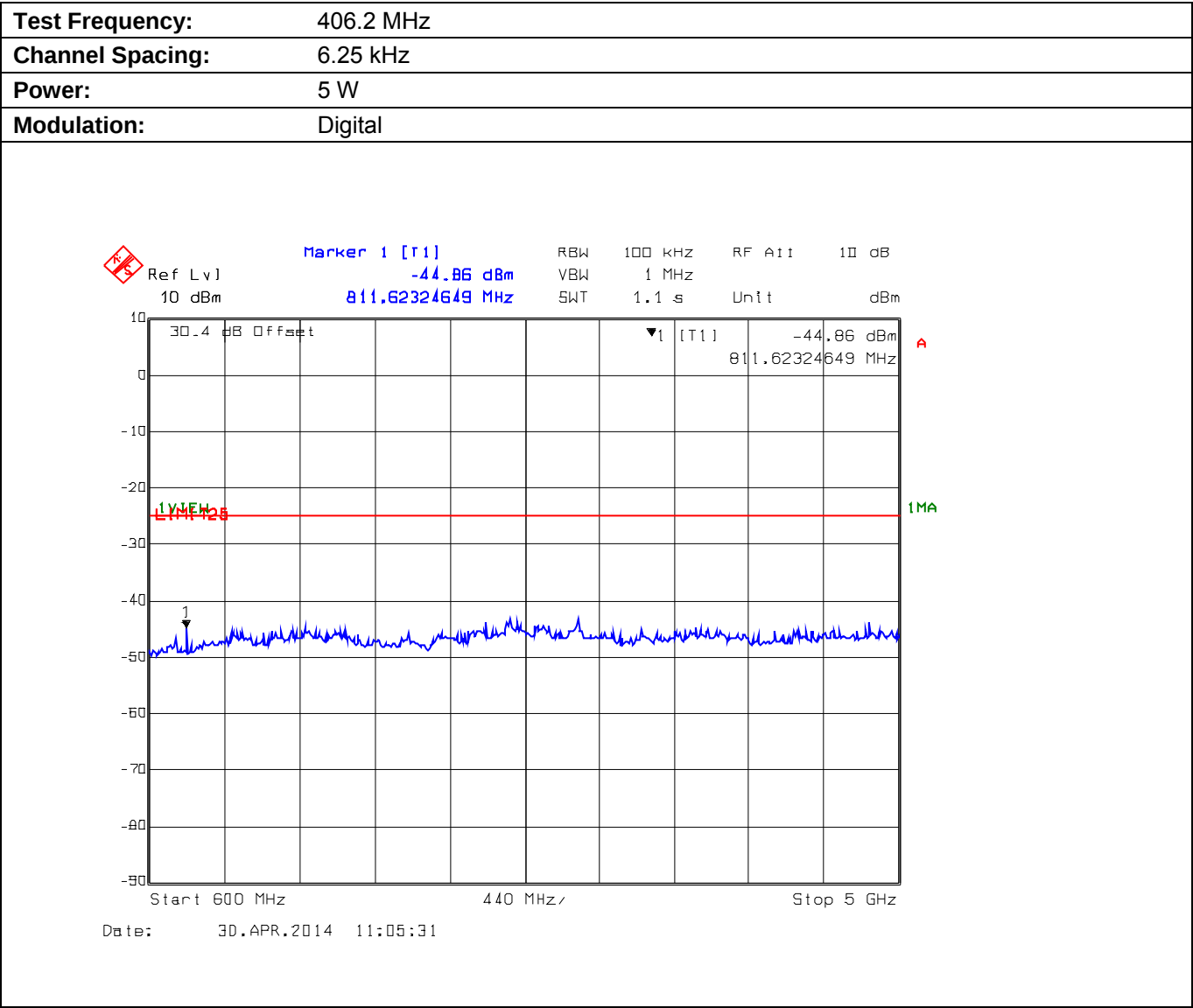
Plot 5.9.4.1.2. Conducted Transmitter Spurious Emissions for 406.2 MHz, High Power, 600 MHz - 5 GHz
