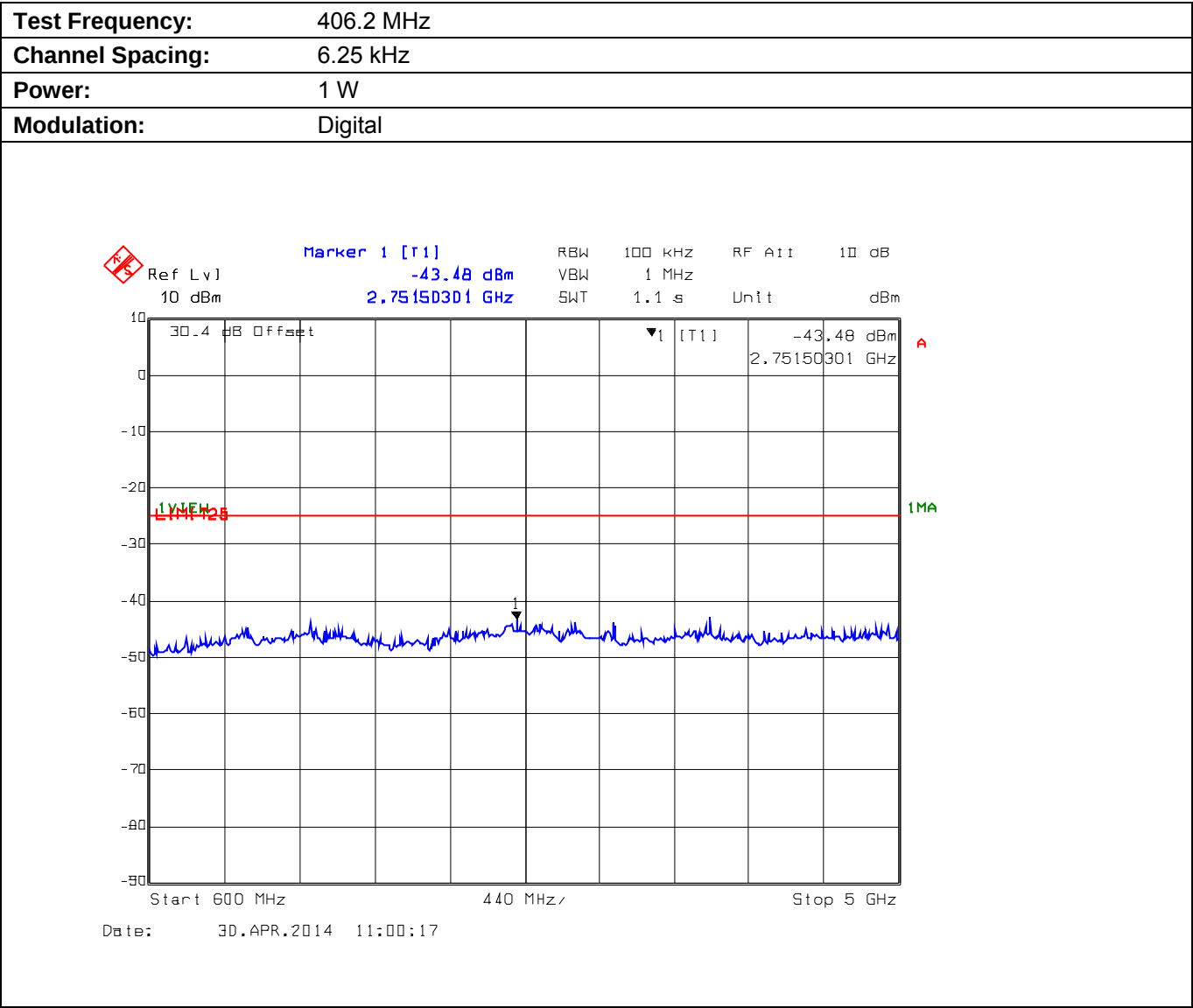
Plot 5.9.4.1.4. Conducted Transmitter Spurious Emissions for 406.2 MHz, Low Power, 600 MHz - 5 GHz
