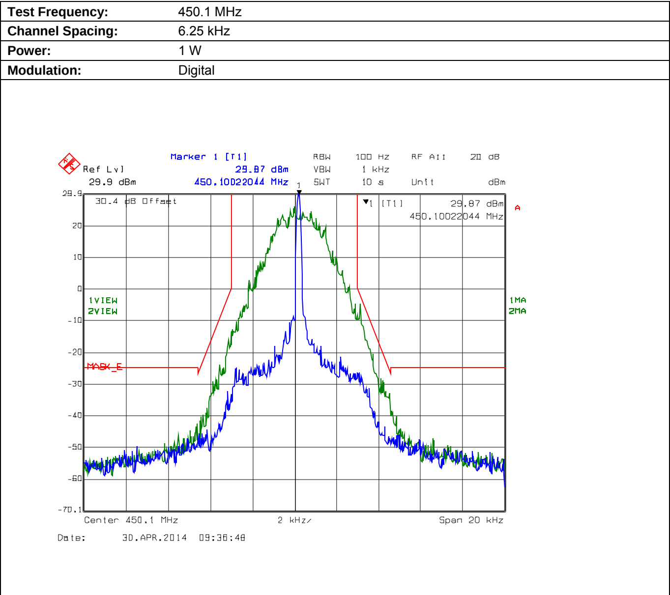
Plot 5.8.4.4.5. Emission Mask E, Low Power
