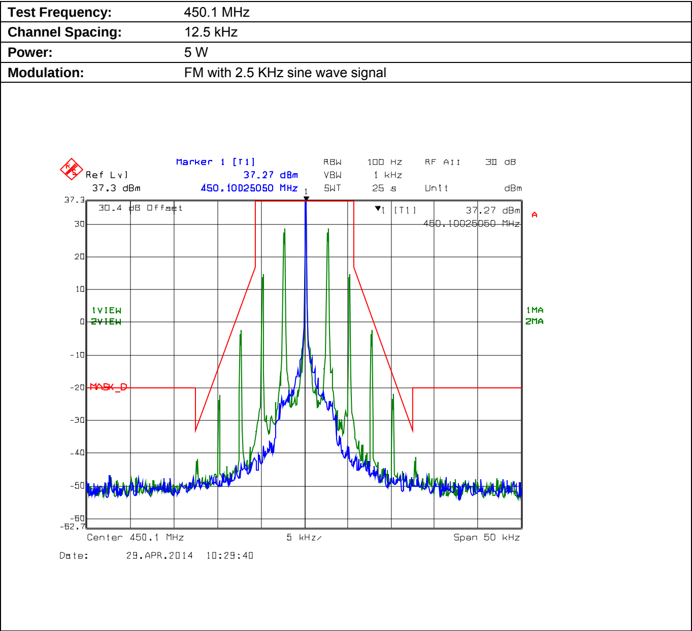
Plot 5.8.4.2.2. Emission Mask D, High Power
