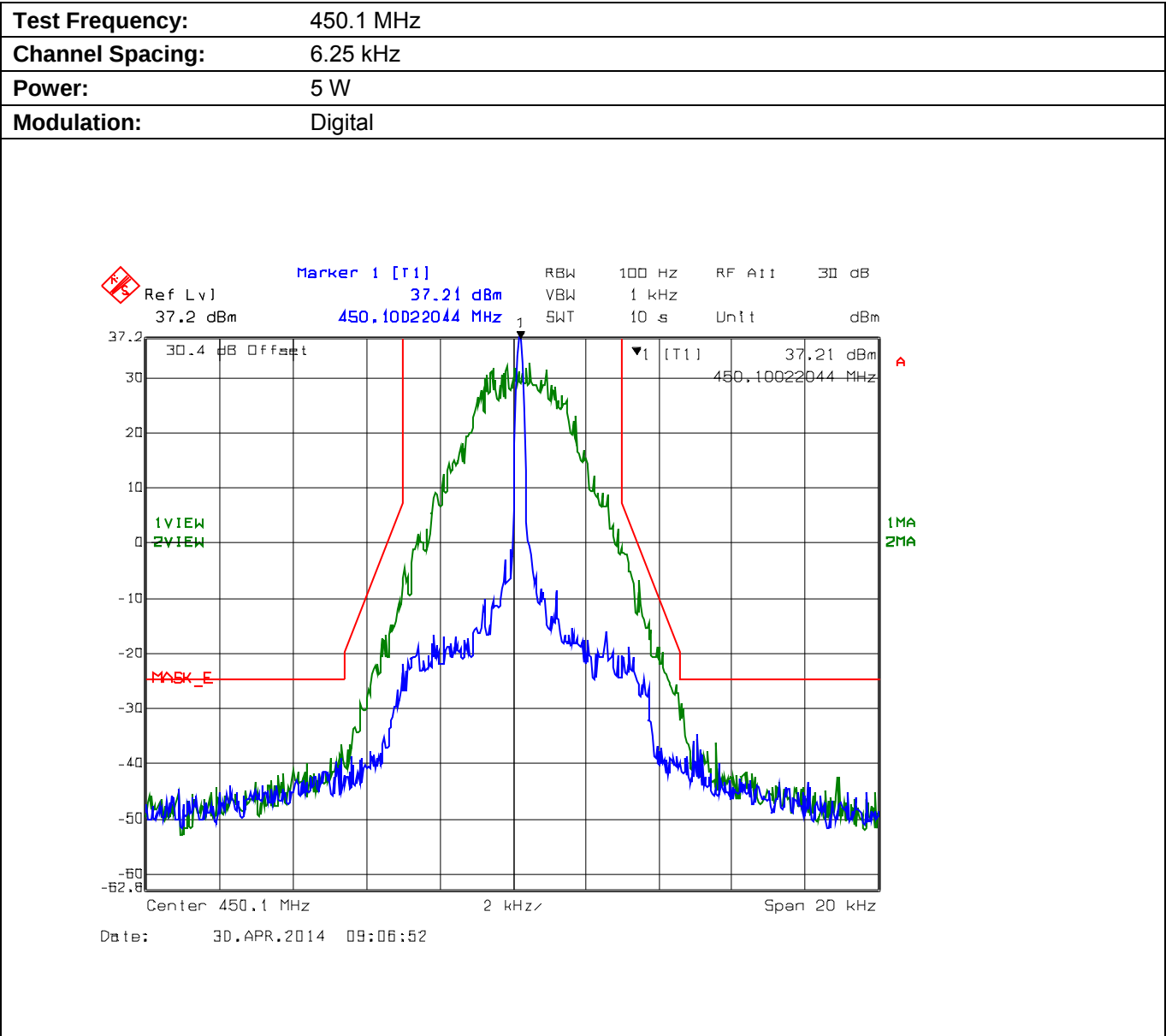
Plot 5.8.4.4.2. Emission Mask E, High Power
