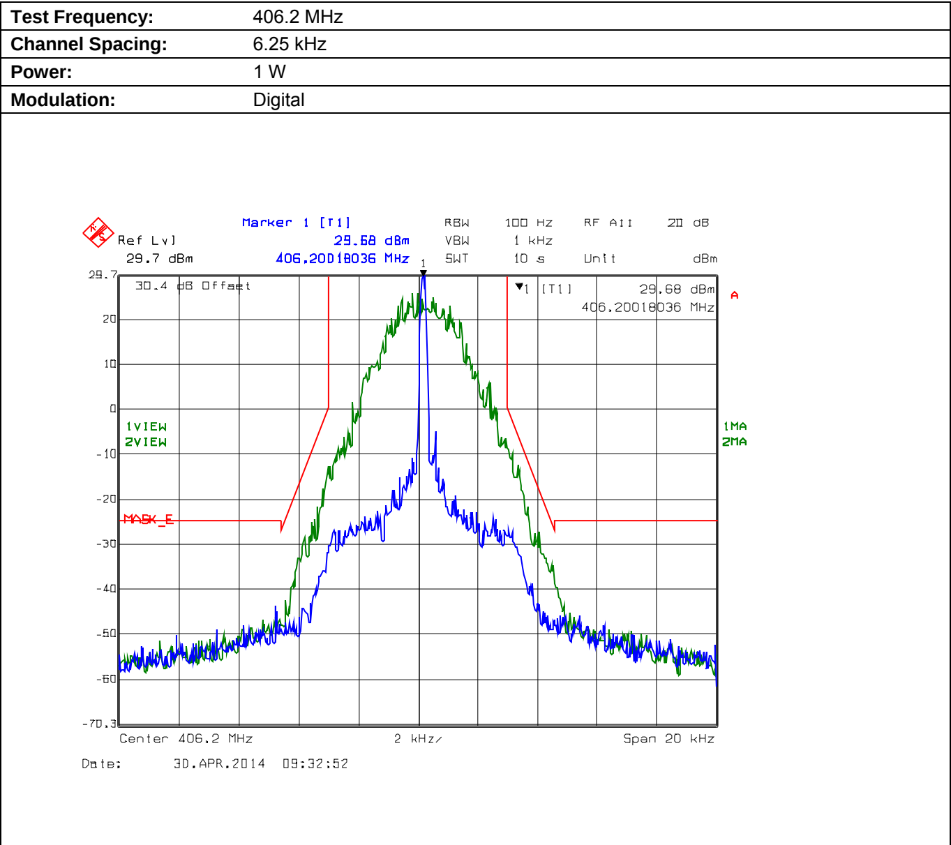
Plot 5.8.4.4.4. Emission Mask E, Low Power
