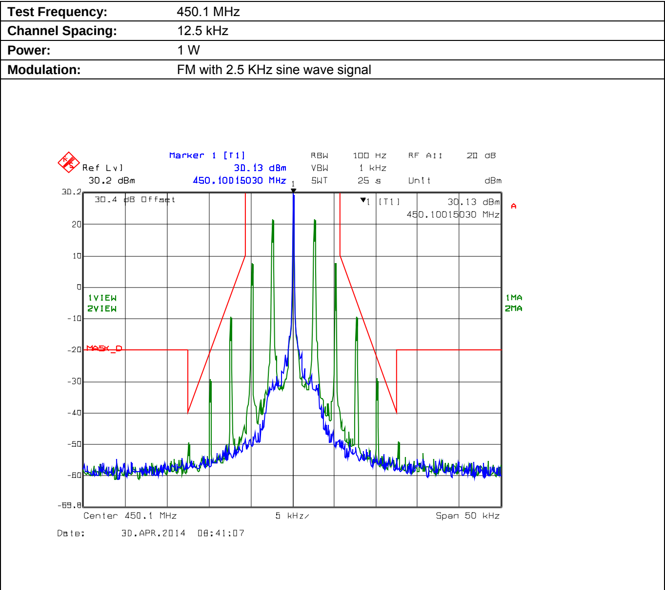
Plot 5.8.4.2.5. Emission Mask D, Low Power
