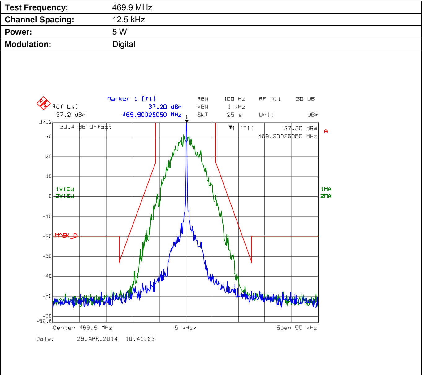
Plot 5.8.4.2.9. Emission Mask D, High Power
