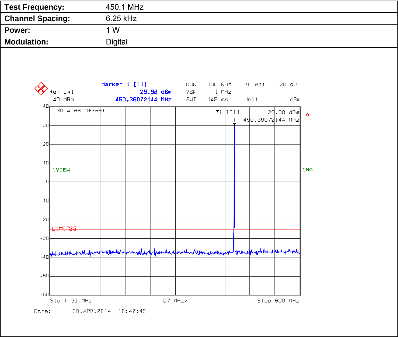
Plot 5.9.4.2.3. Conducted Transmitter Spurious Emissions for 450.1 MHz, Low Power, 30 MHz - 600 MHz
