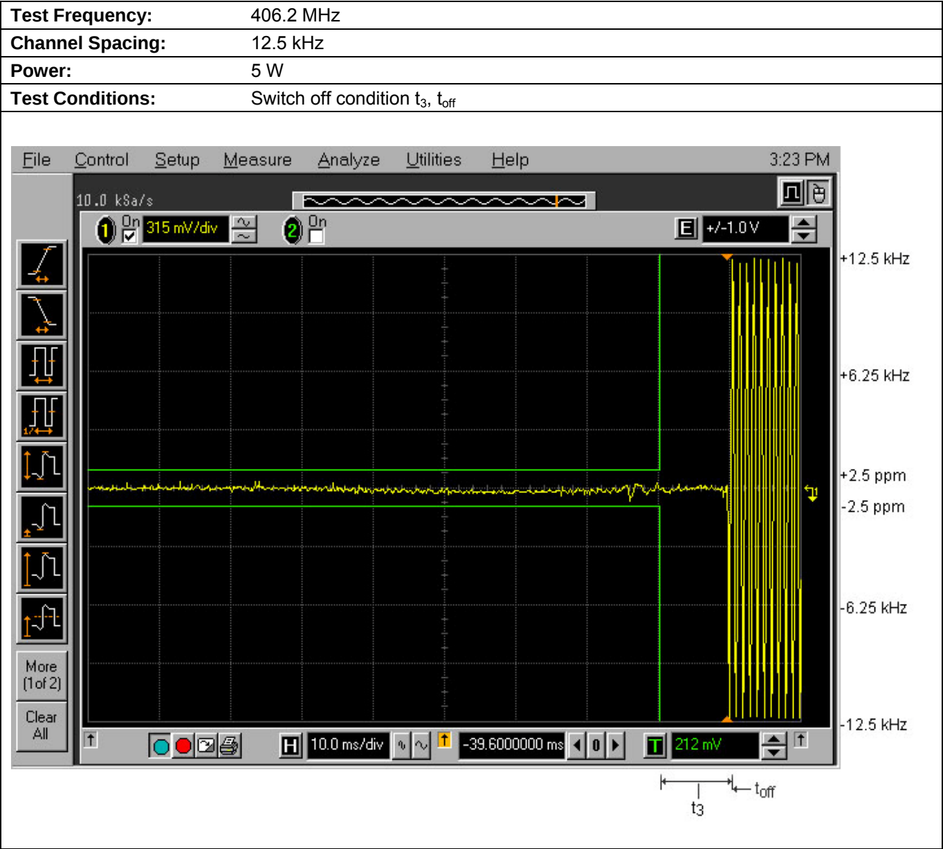
Plot 5.12.4.2. Transient Frequency Behavior for 12.5 kHz Channel Spacing
