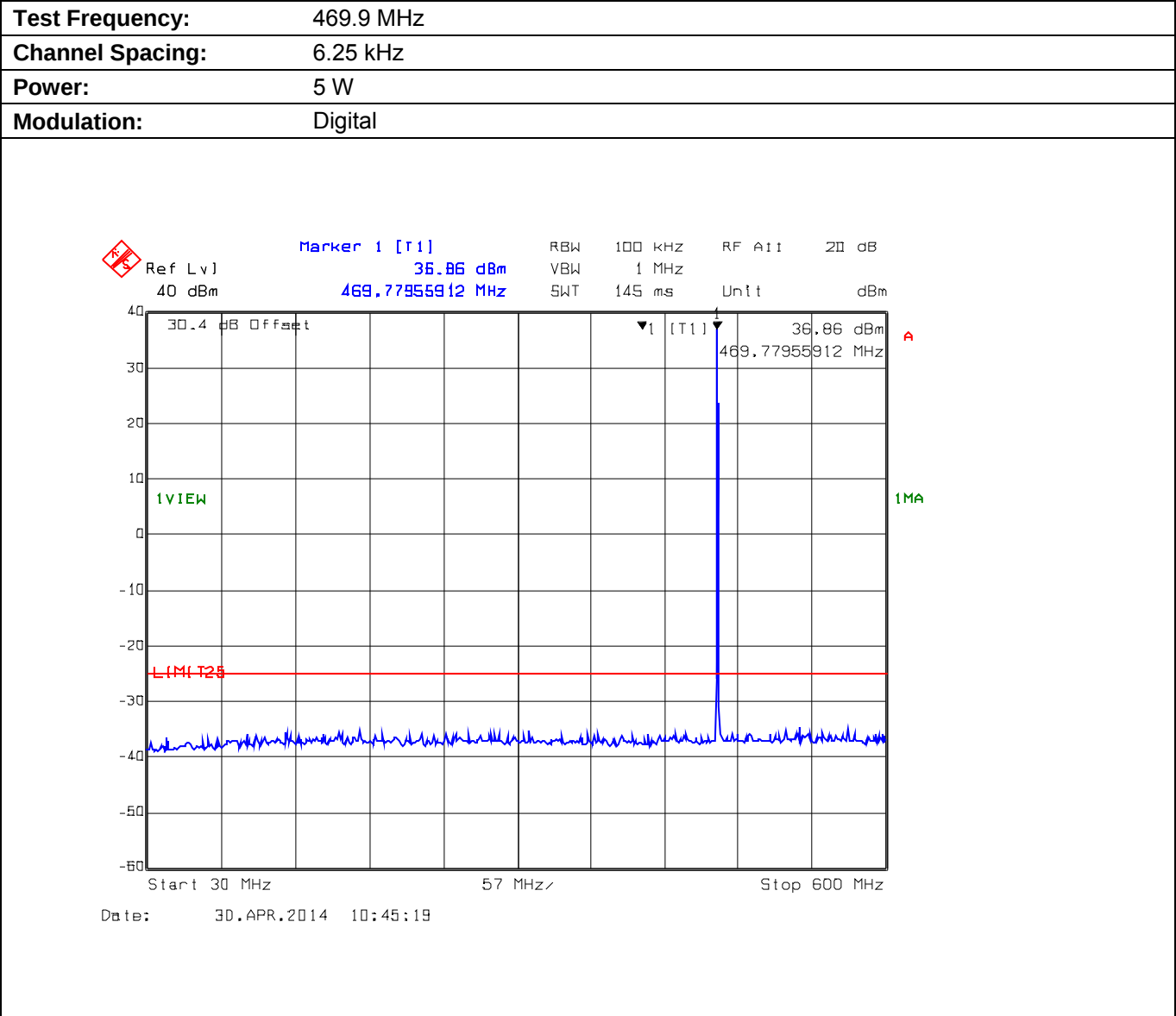
Plot 5.9.4.3.1. Conducted Transmitter Spurious Emissions for 469.9 MHz, High Power, 30 MHz - 600 MHz
