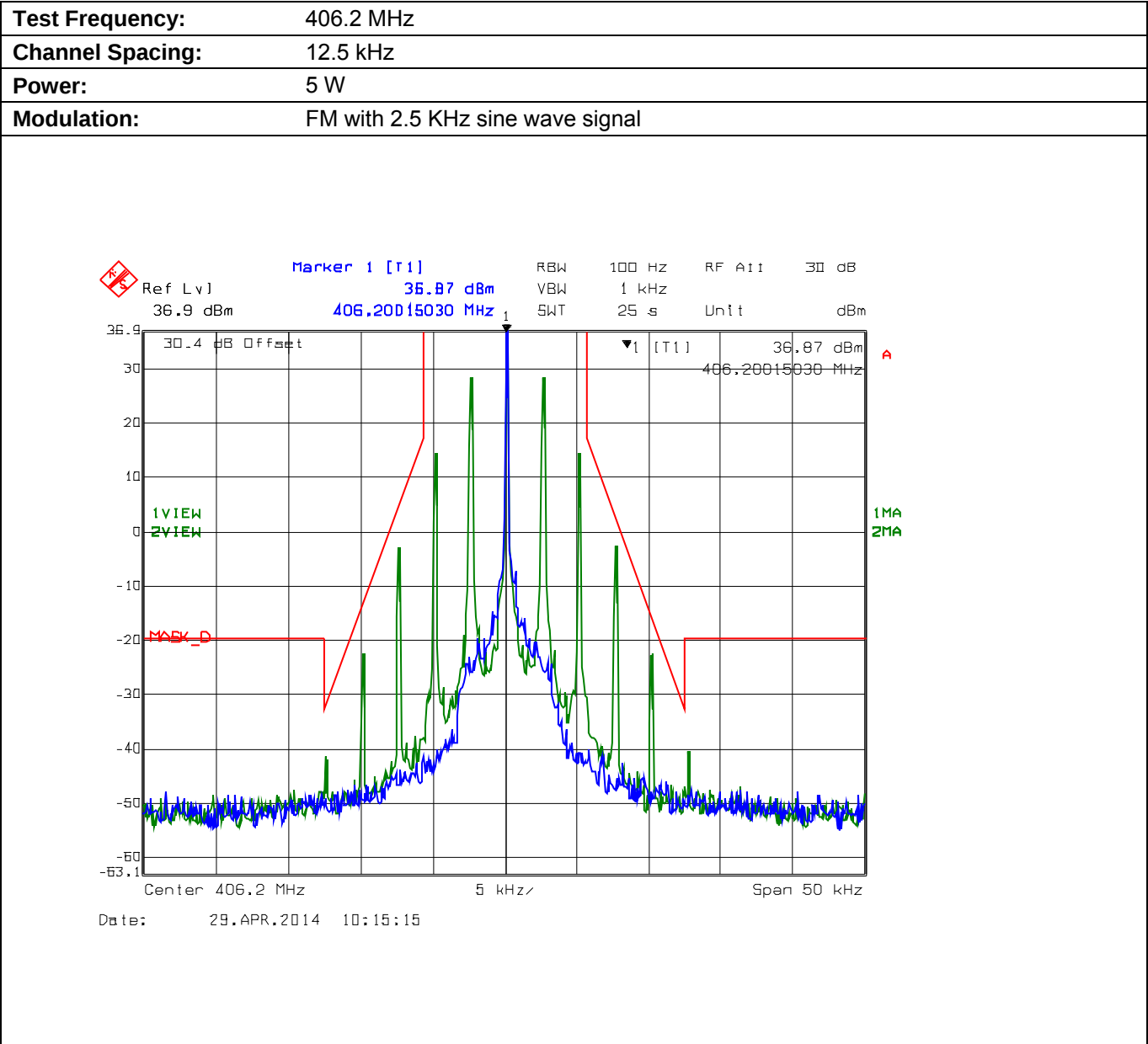
Plot 5.8.4.2.1. Emission Mask D, High Power
