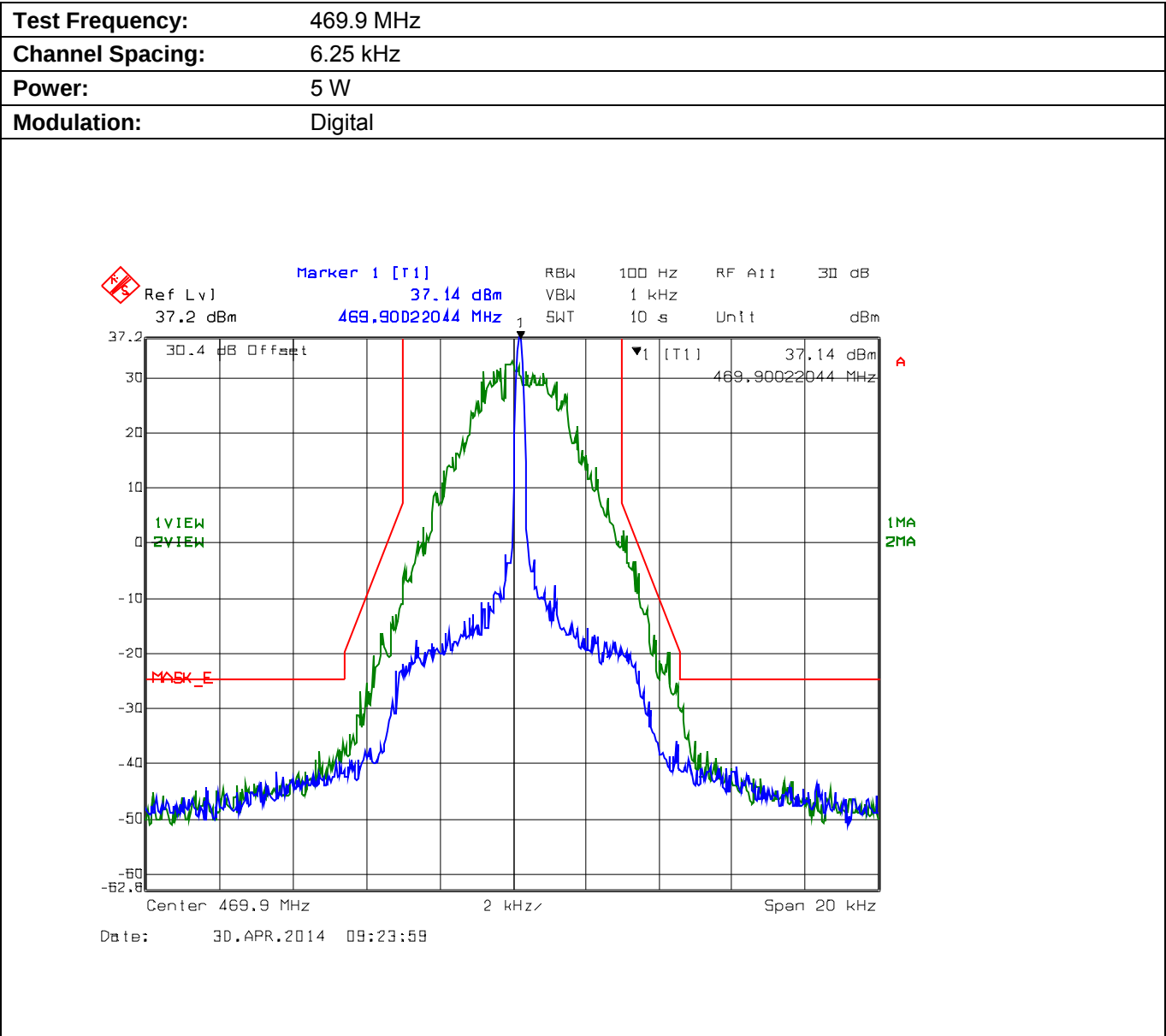
Plot 5.8.4.4.3. Emission Mask E, High Power
