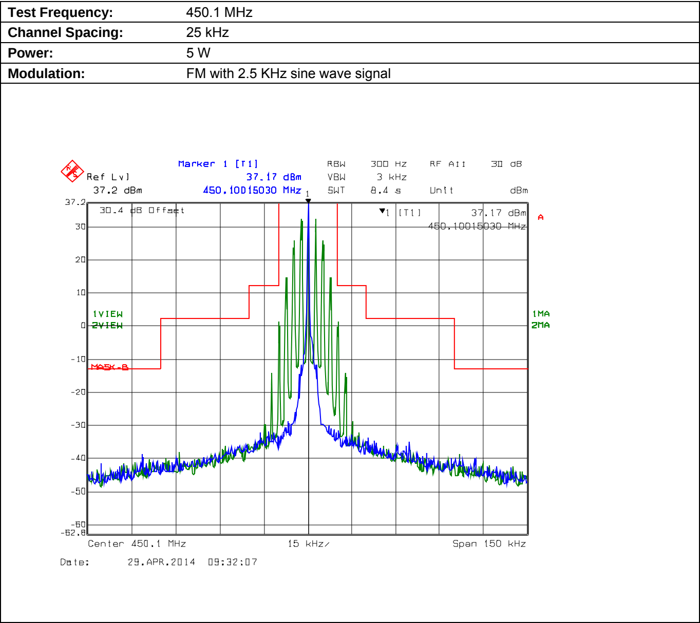
Plot 5.8.4.3.2. Emission Mask B, High Power
