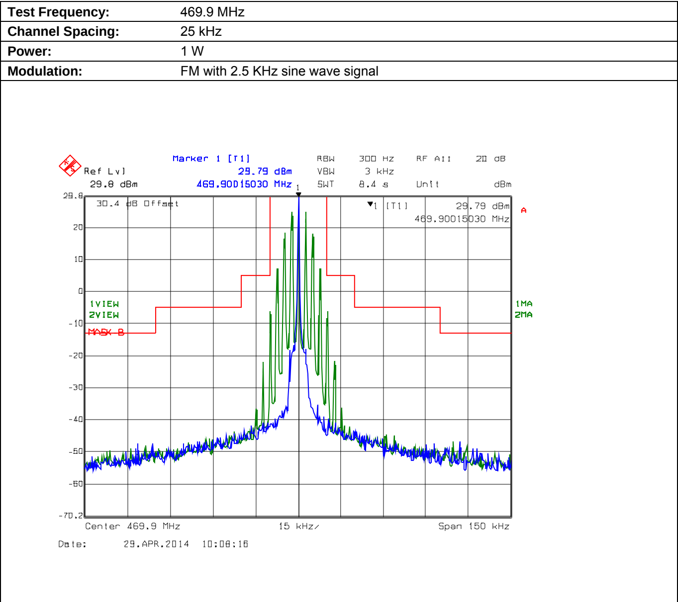
Plot 5.8.4.3.6. Emission Mask B, Low Power
