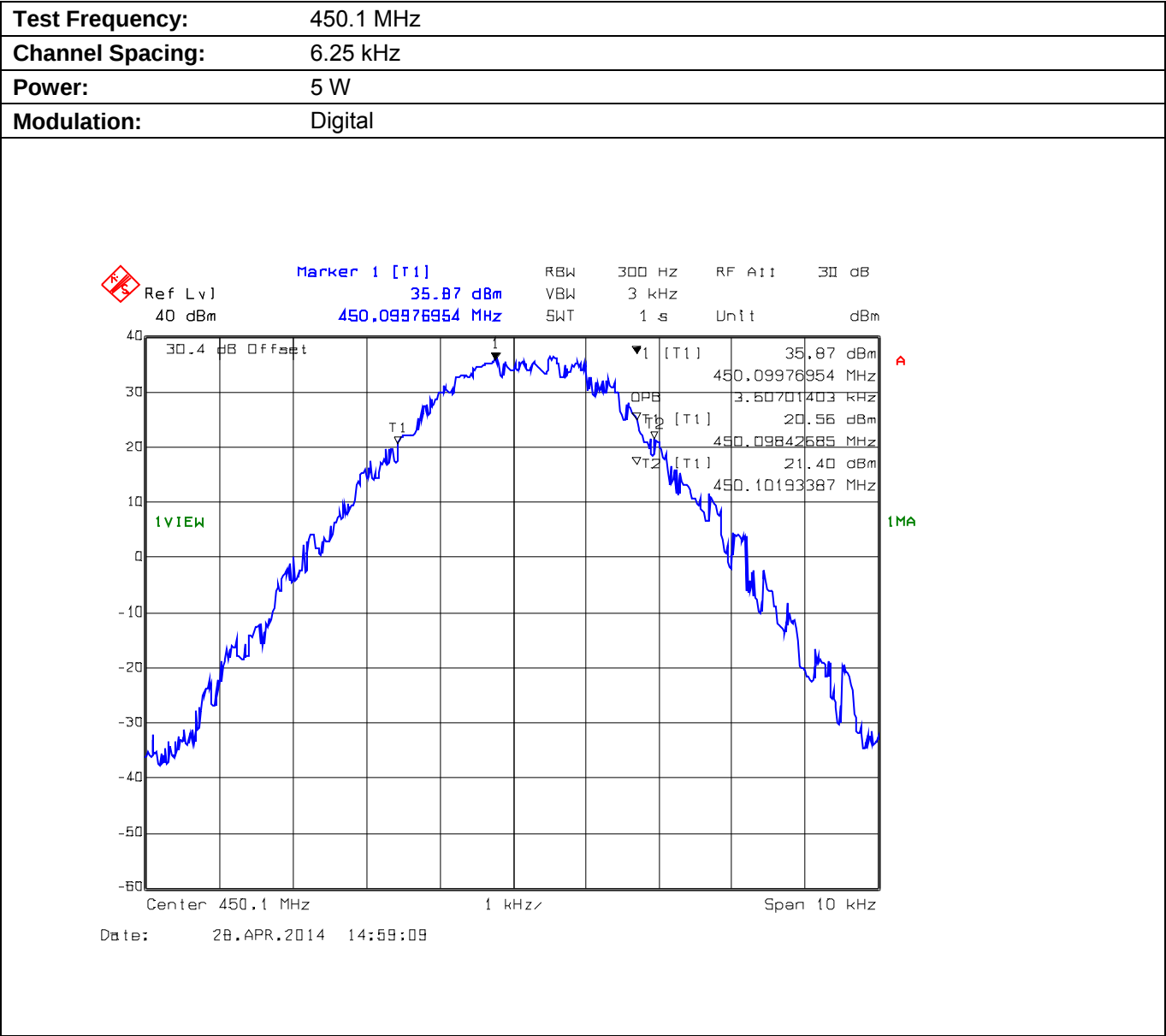
Plot 5.8.4.1.11. Occupied Bandwidth
