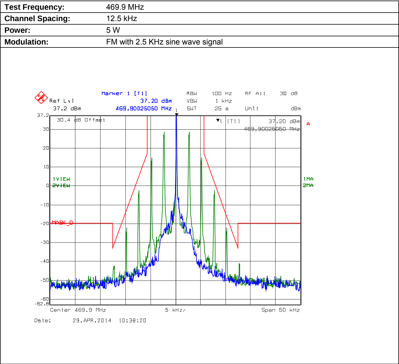
Plot 5.8.4.2.3. Emission Mask D, High Power
