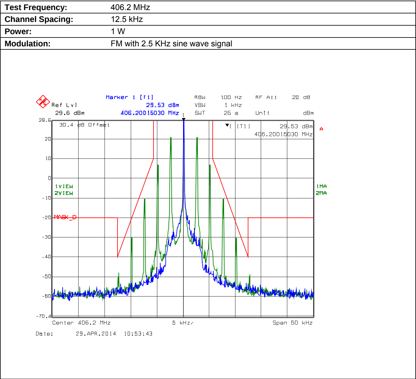
Plot 5.8.4.2.4. Emission Mask D, Low Power
