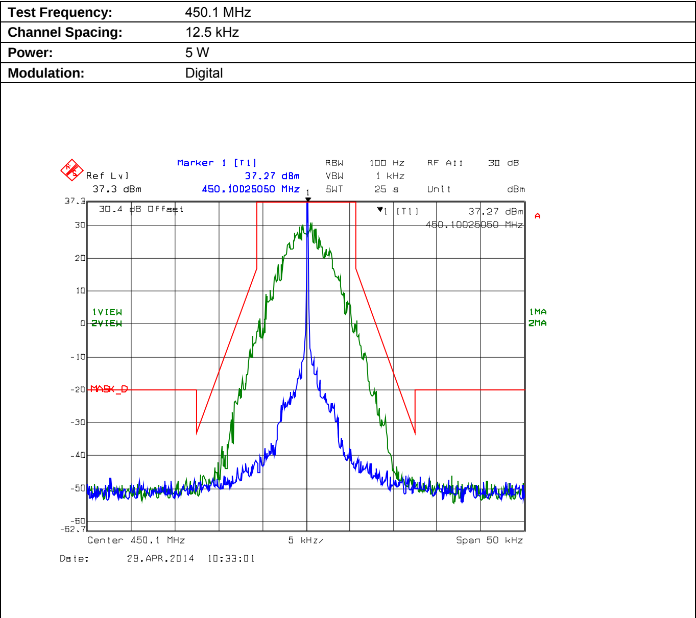
Plot 5.8.4.2.8. Emission Mask D, High Power
