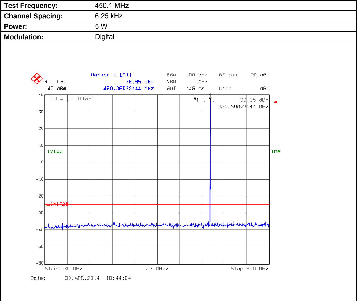
Plot 5.9.4.2.1. Conducted Transmitter Spurious Emissions for 450.1 MHz, High Power, 30 MHz - 600 MHz
