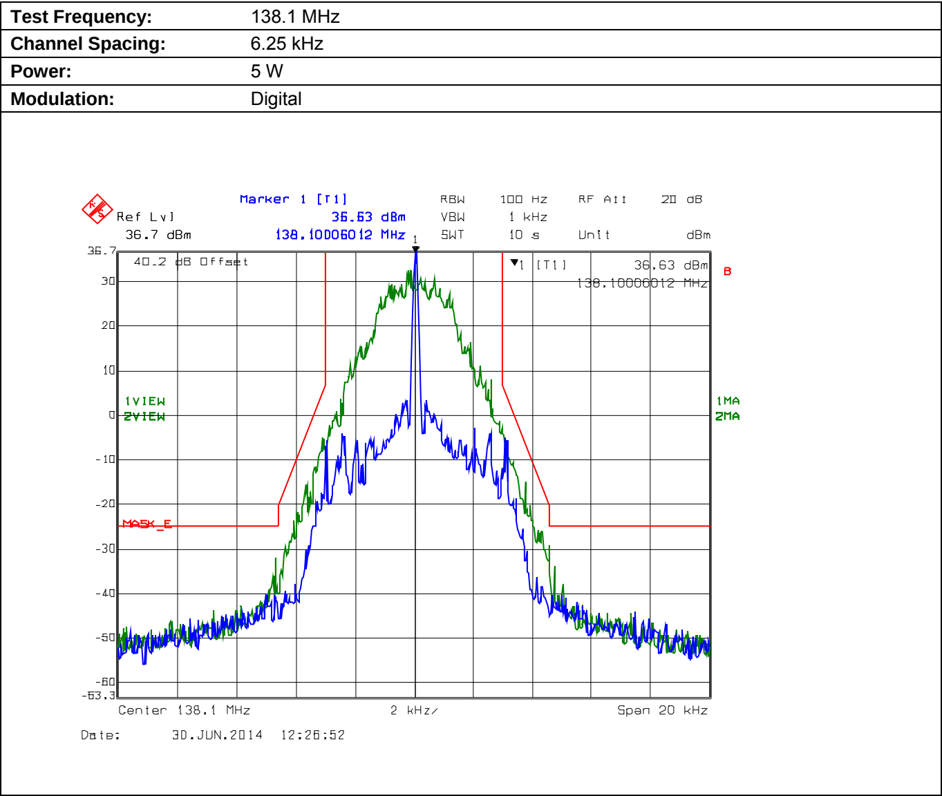
Plot 5.8.4.4. Emission Mask E, Low Power
