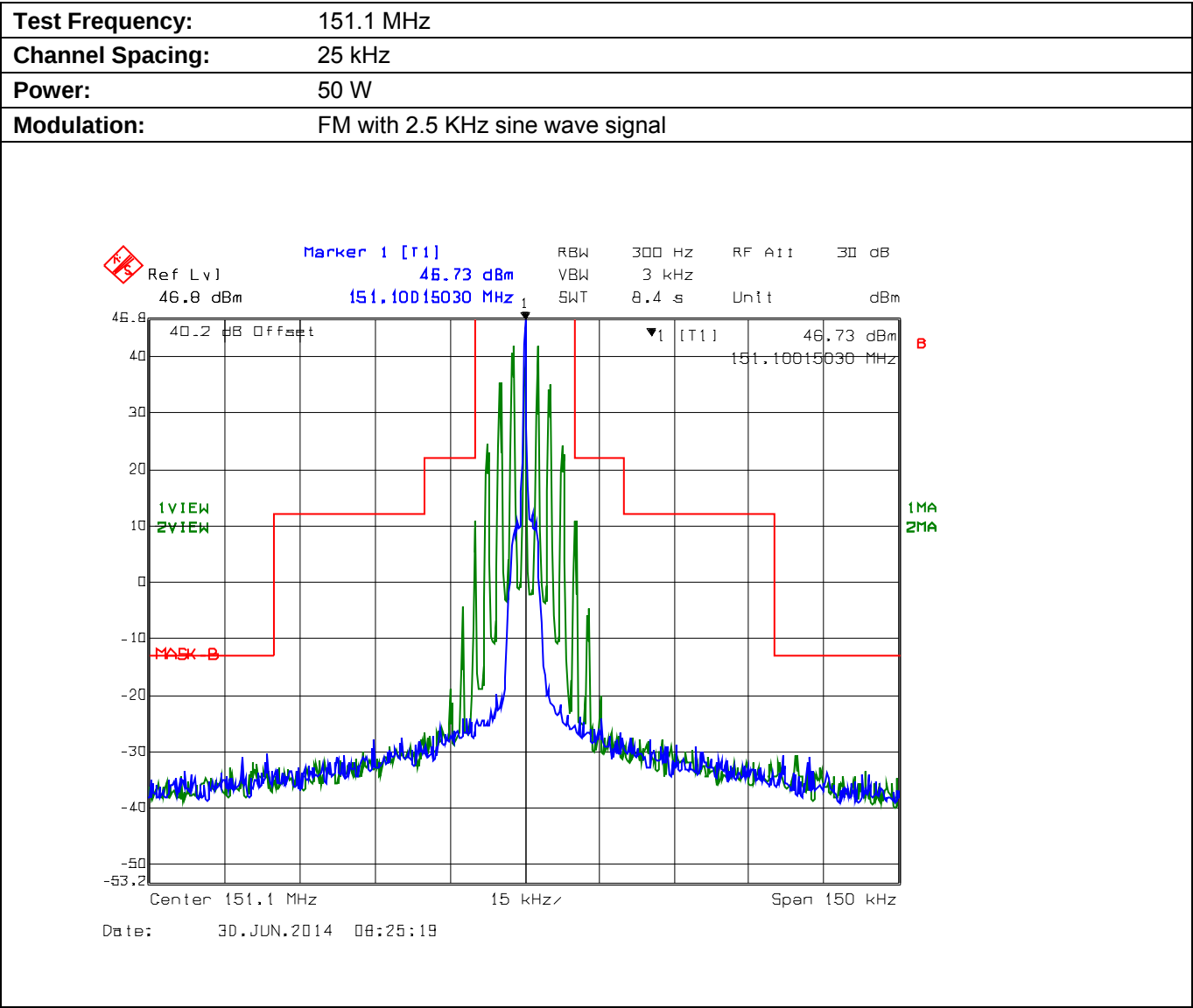
Plot 5.8.4.3.2. Emission Mask B, High Power
