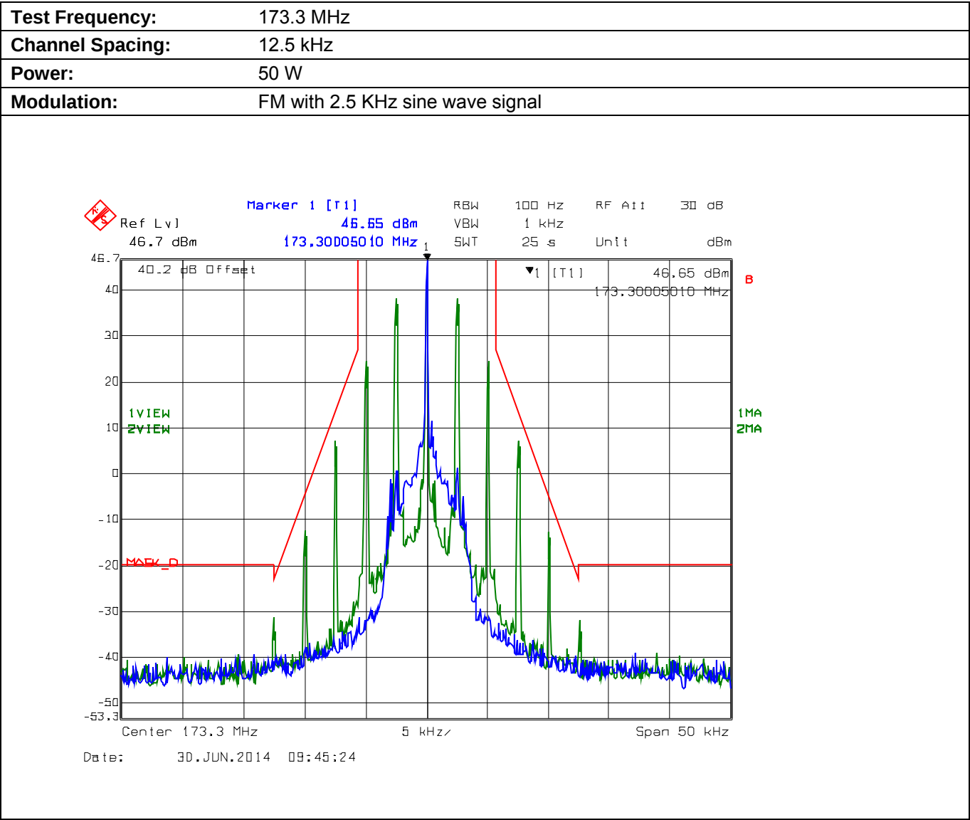
Plot 5.8.4.2.3. Emission Mask D, High Power
