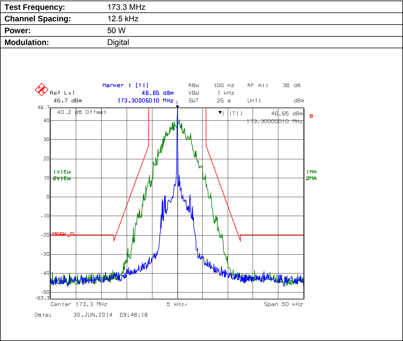
Plot 5.8.4.2.9. Emission Mask D, High Power
