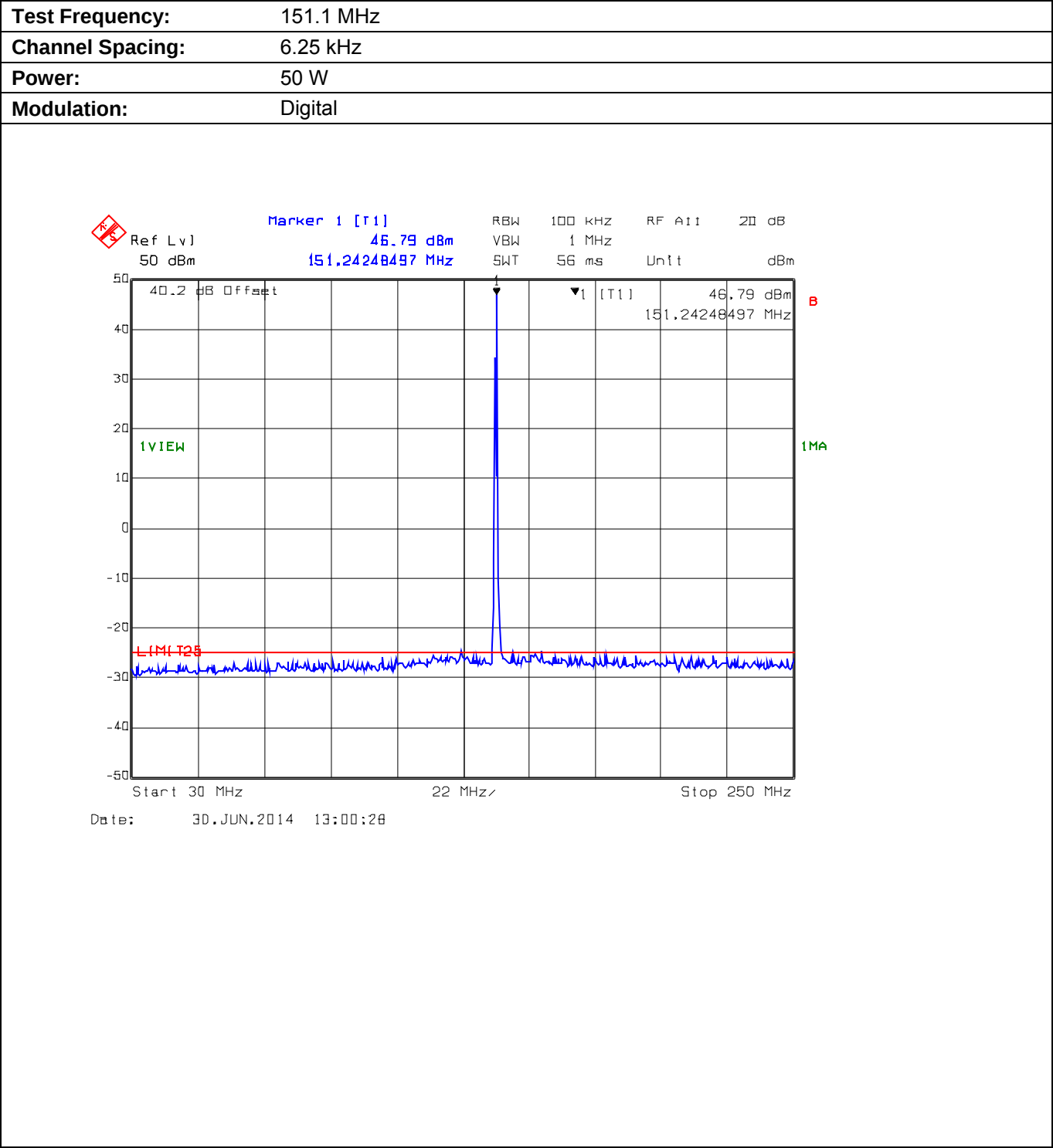
Plot 5.9.4.2.1. Conducted Transmitter Spurious Emissions for 151.1 MHz, High Power, 30 MHz - 250 MHz
