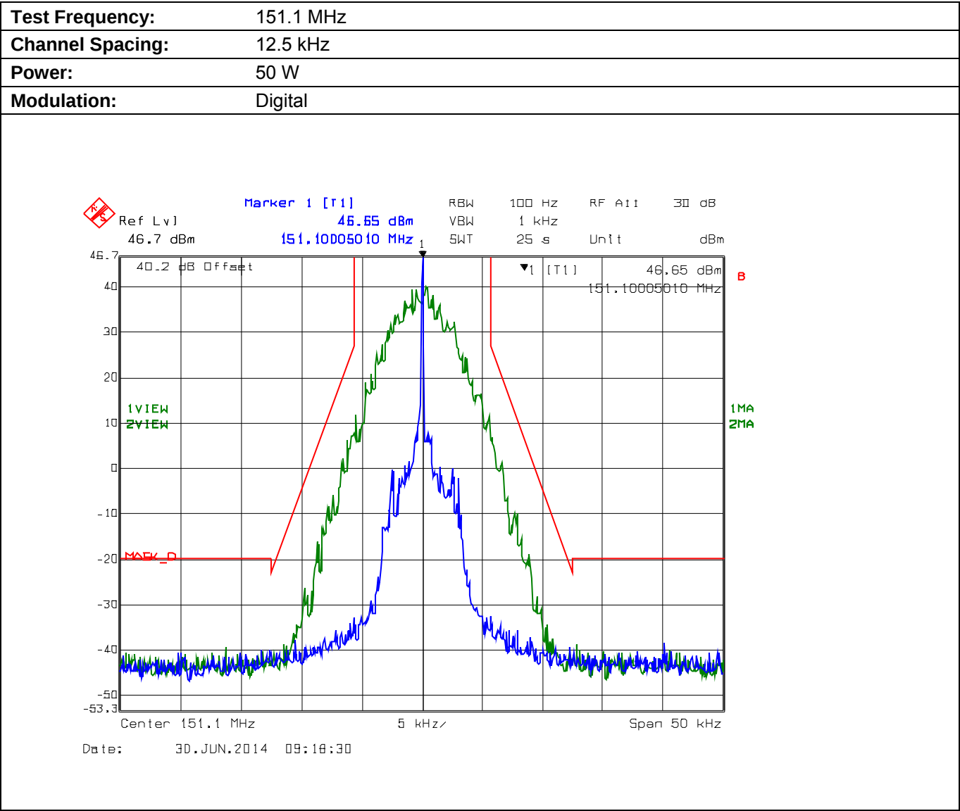
Plot 5.8.4.2.8. Emission Mask D, High Power
