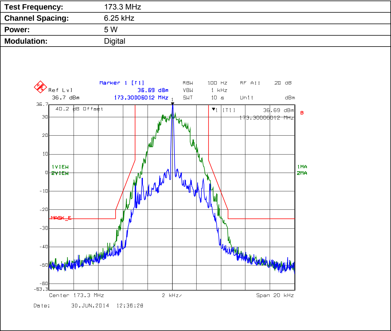
Plot 5.8.4.4.6. Emission Mask E, Low Power
