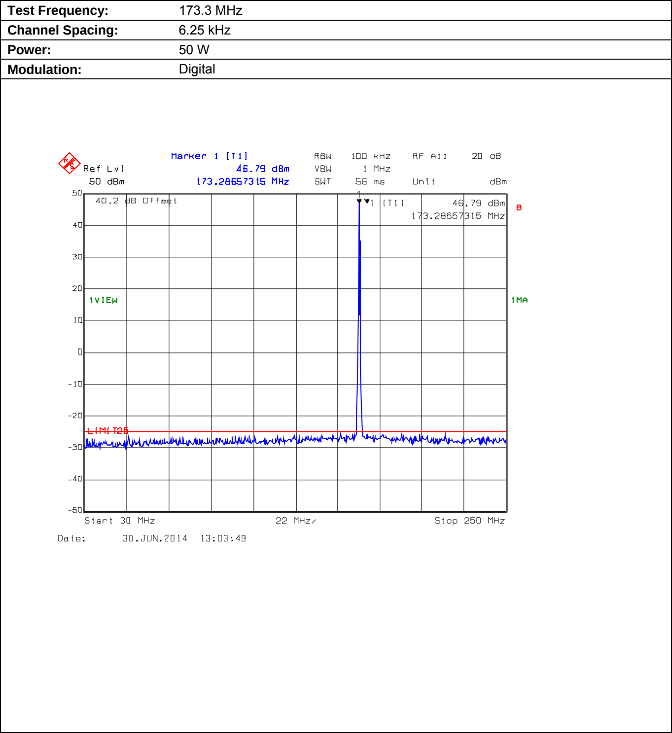
Plot 5.9.4.3.1. Conducted Transmitter Spurious Emissions for 173.3 MHz, High Power, 30 MHz - 250 MHz
