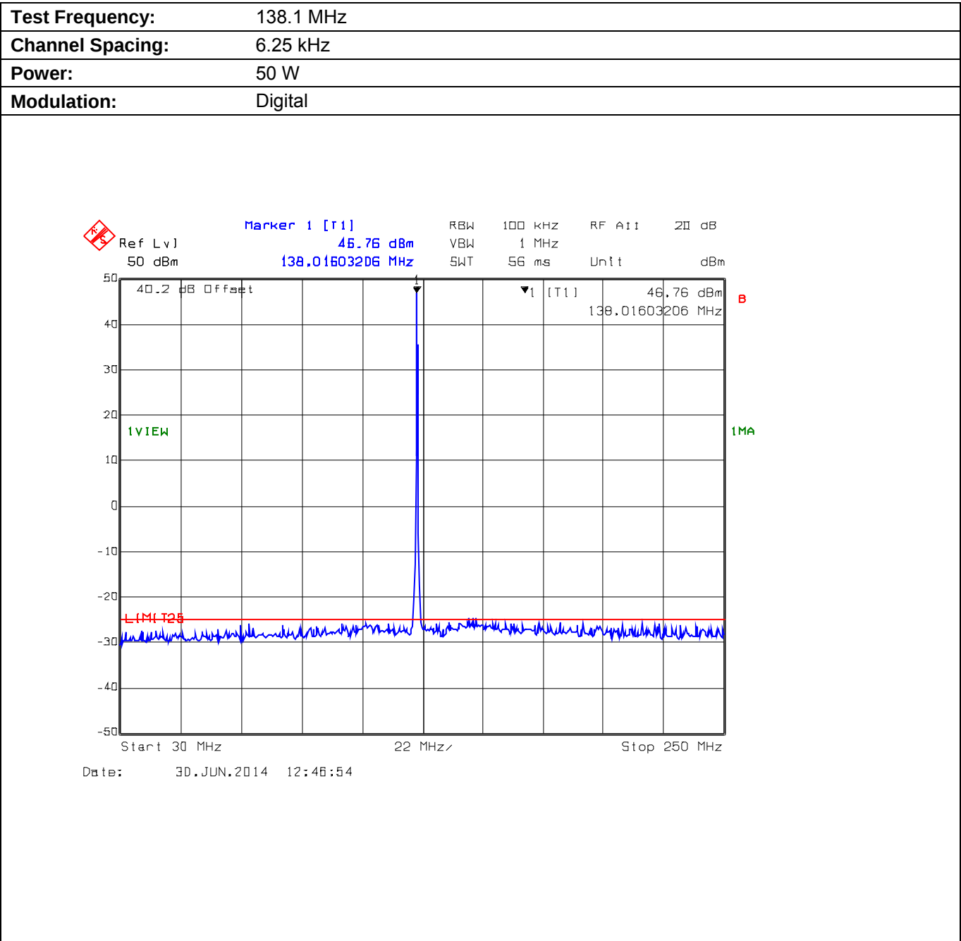
Plot 5.9.4.1.1. Conducted Transmitter Spurious Emissions for 138.1 MHz, High Power, 30 MHz - 250 MHz
