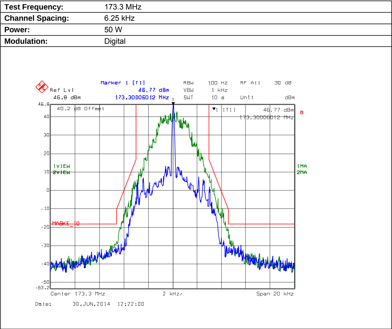
Plot 5.8.4.4.3. Emission Mask E, High Power
