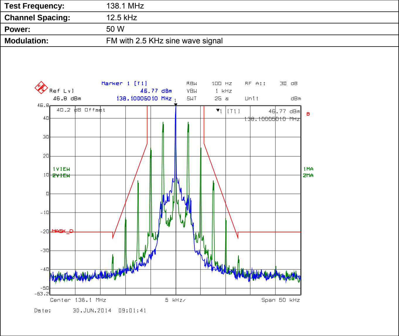
Plot 5.8.4.2.1. Emission Mask D, High Power
