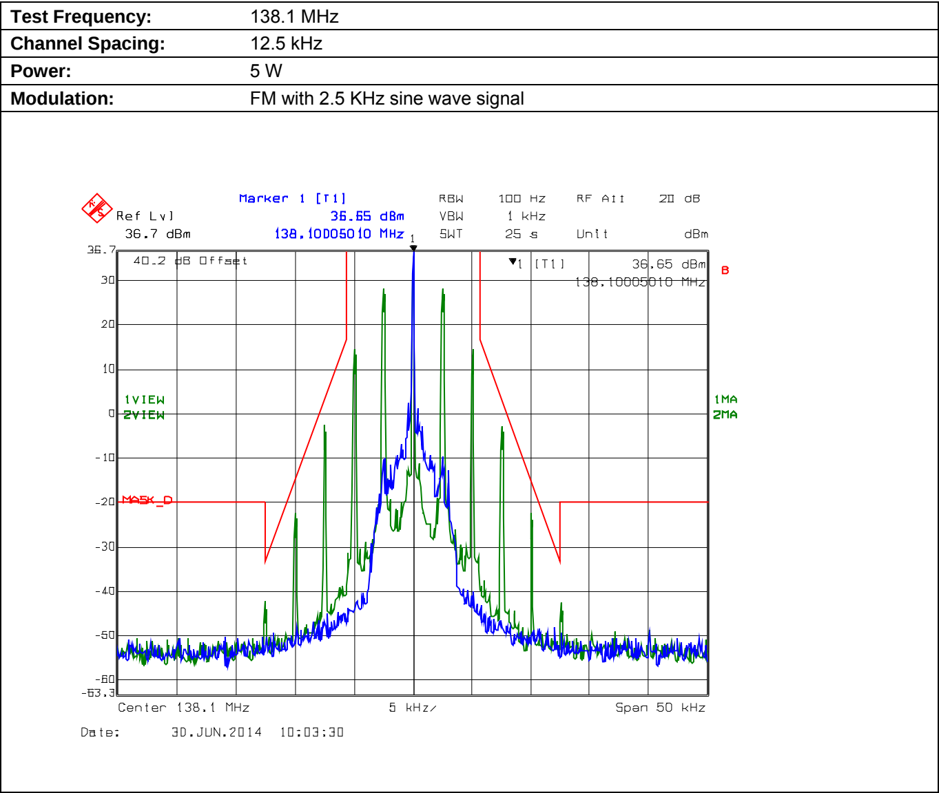
Plot 5.8.4.2.4. Emission Mask D, Low Power
