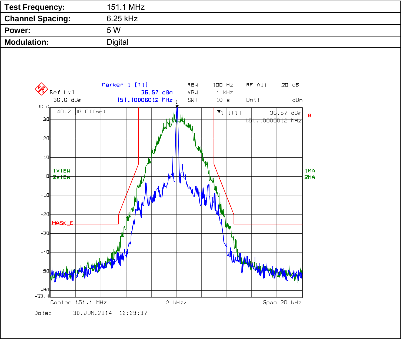
Plot 5.8.4.4.5. Emission Mask E, Low Power
