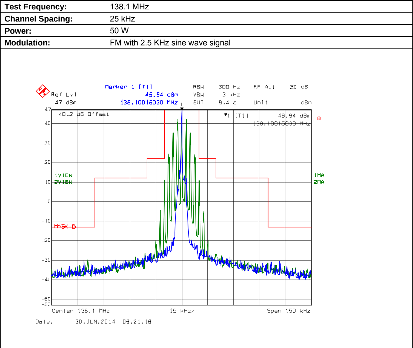
Plot 5.8.4.3.1. Emission Mask B, High Power
