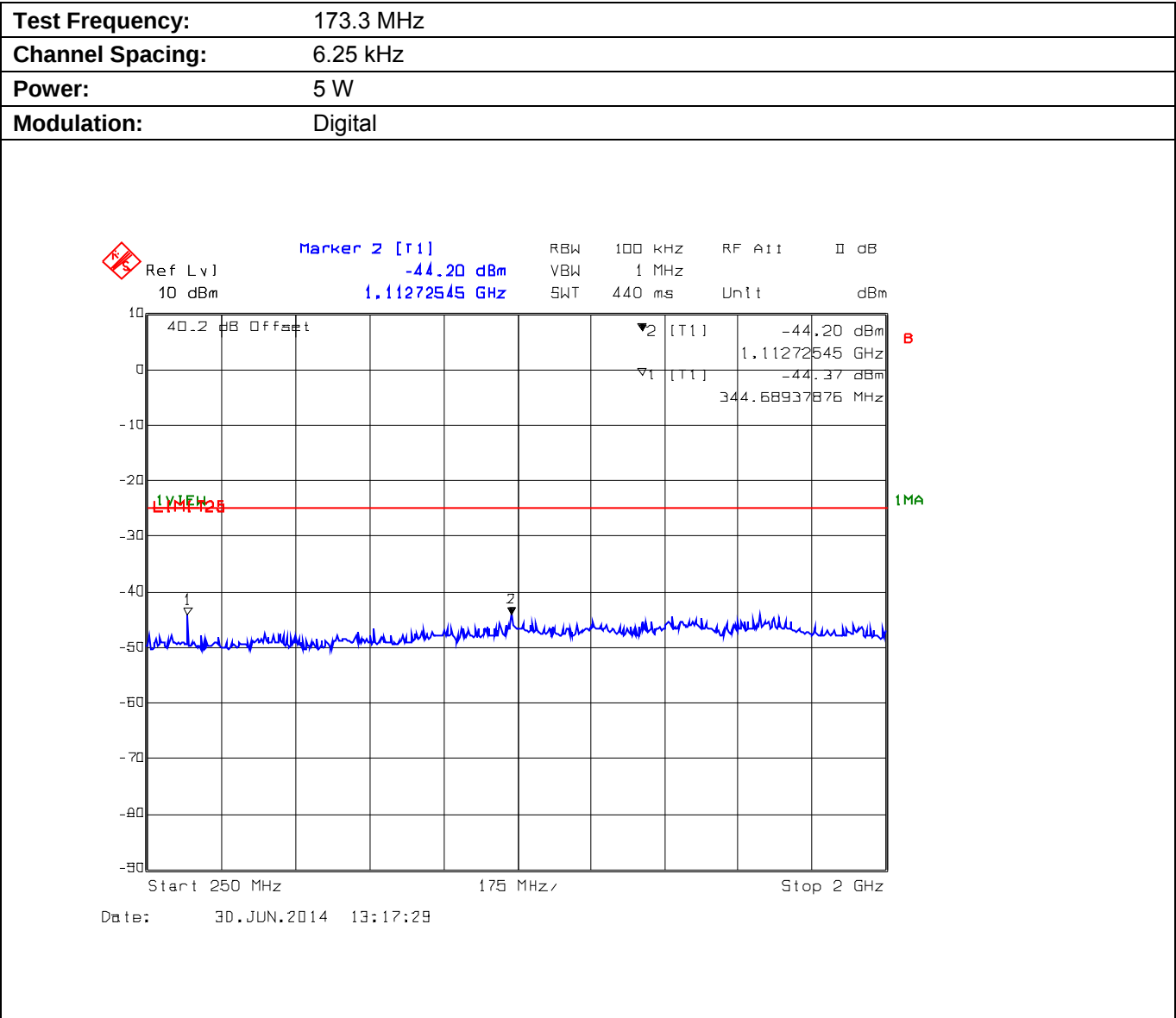
Plot 5.9.4.3.4. Conducted Transmitter Spurious Emissions for 173.3 MHz, Low Power, 250 MHz - 2 GHz
