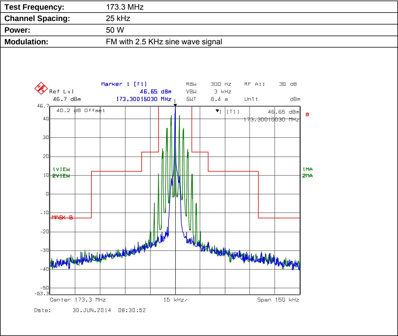
Plot 5.8.4.3.3. Emission Mask B, High Power
