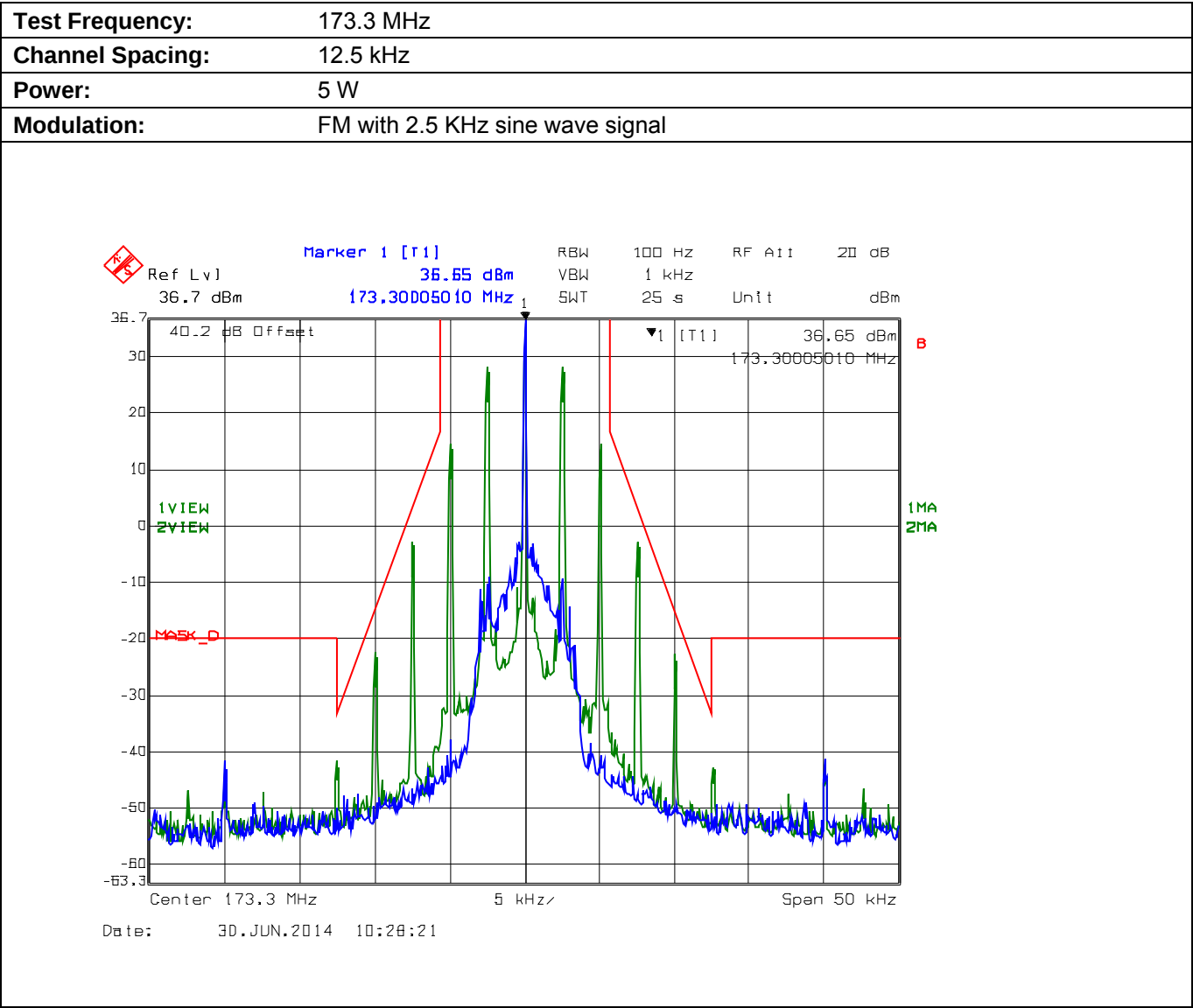
Plot 5.8.4.2.6. Emission Mask D, Low Power
