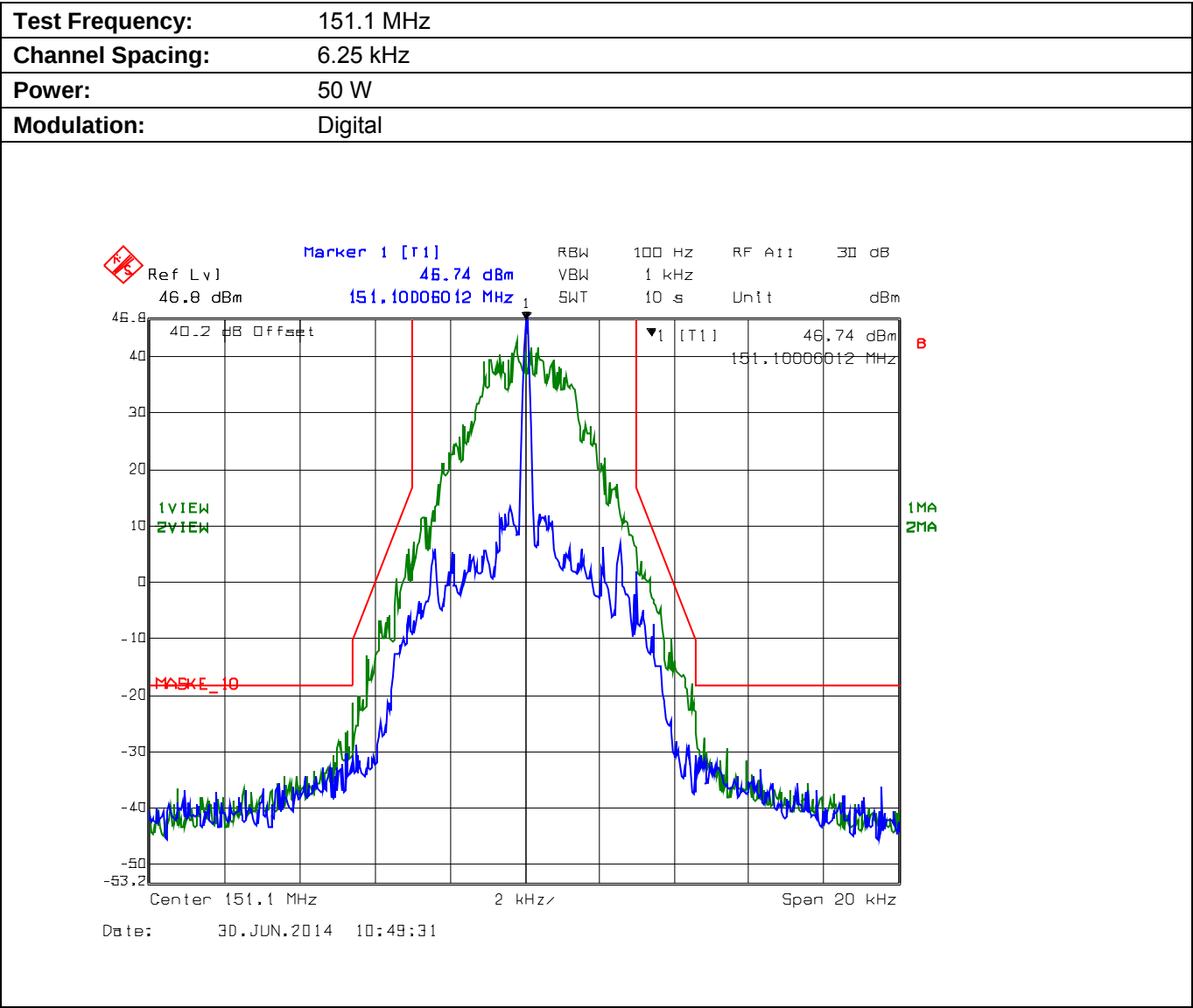
Plot 5.8.4.4.2. Emission Mask E, High Power
