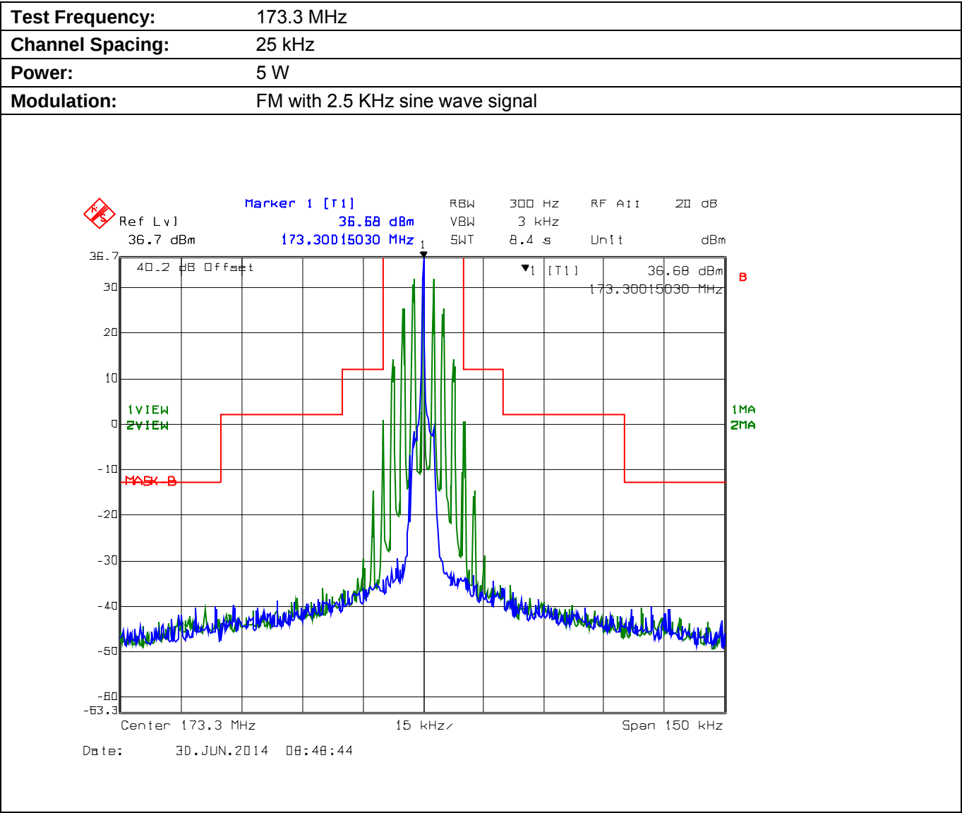
Plot 5.8.4.3.6. Emission Mask B, Low Power
