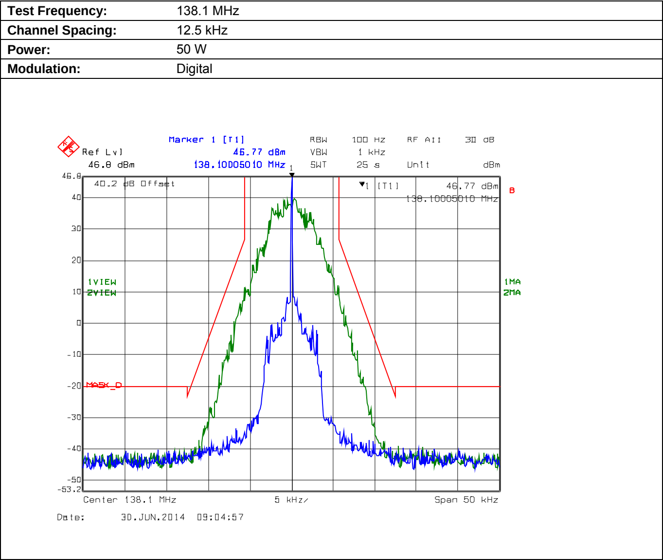
Plot 5.8.4.2.7. Emission Mask D, High Power
