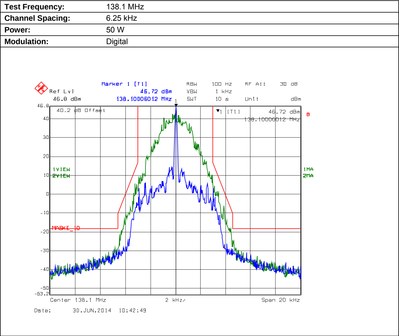
Plot 5.8.4.4.1. Emission Mask E, High Power
