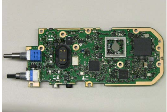
Main Board - Back -
