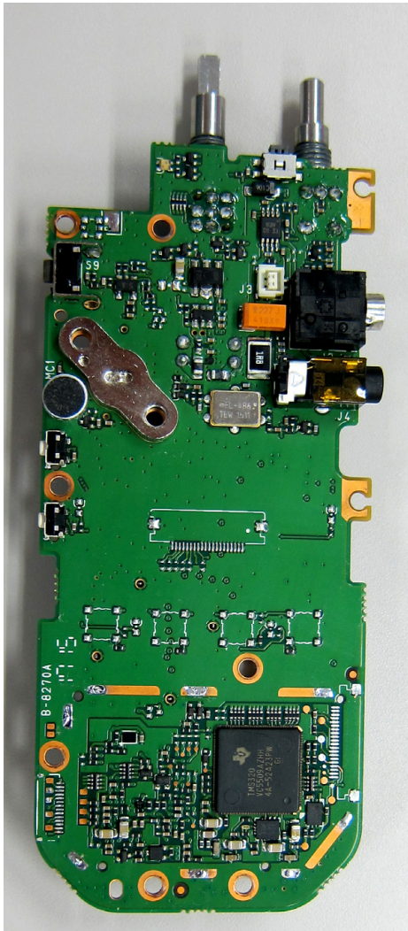
Main Board - Front -
