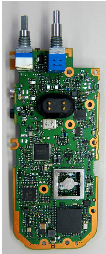
Main Board - Back -
