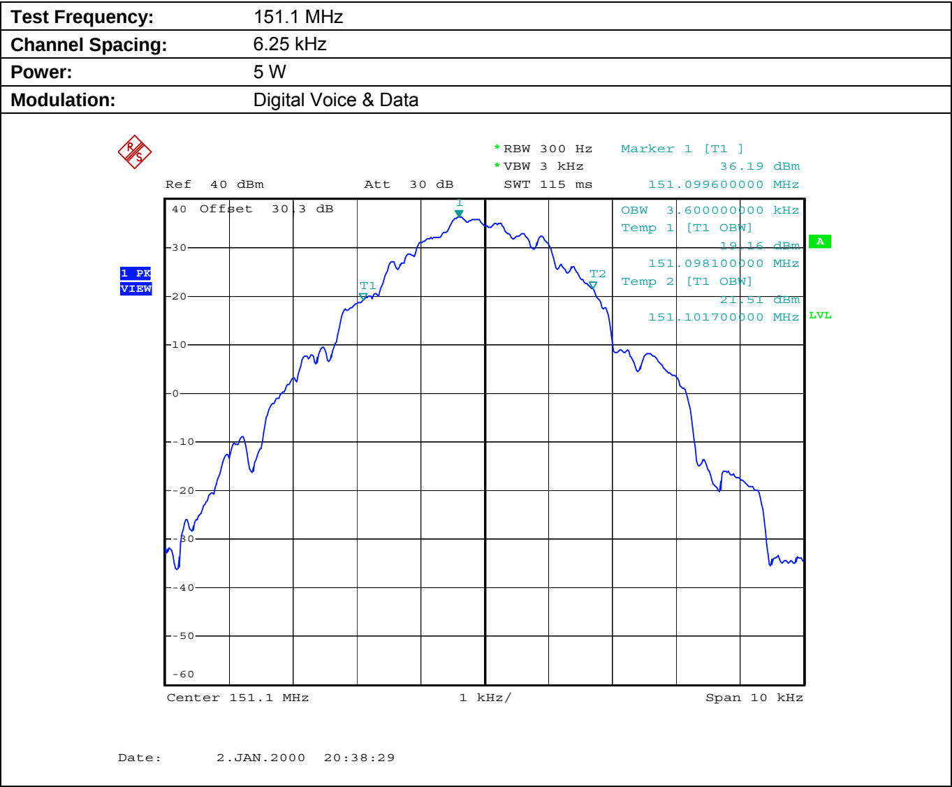
Plot 5.8.4.1.8. Occupied Bandwidth
