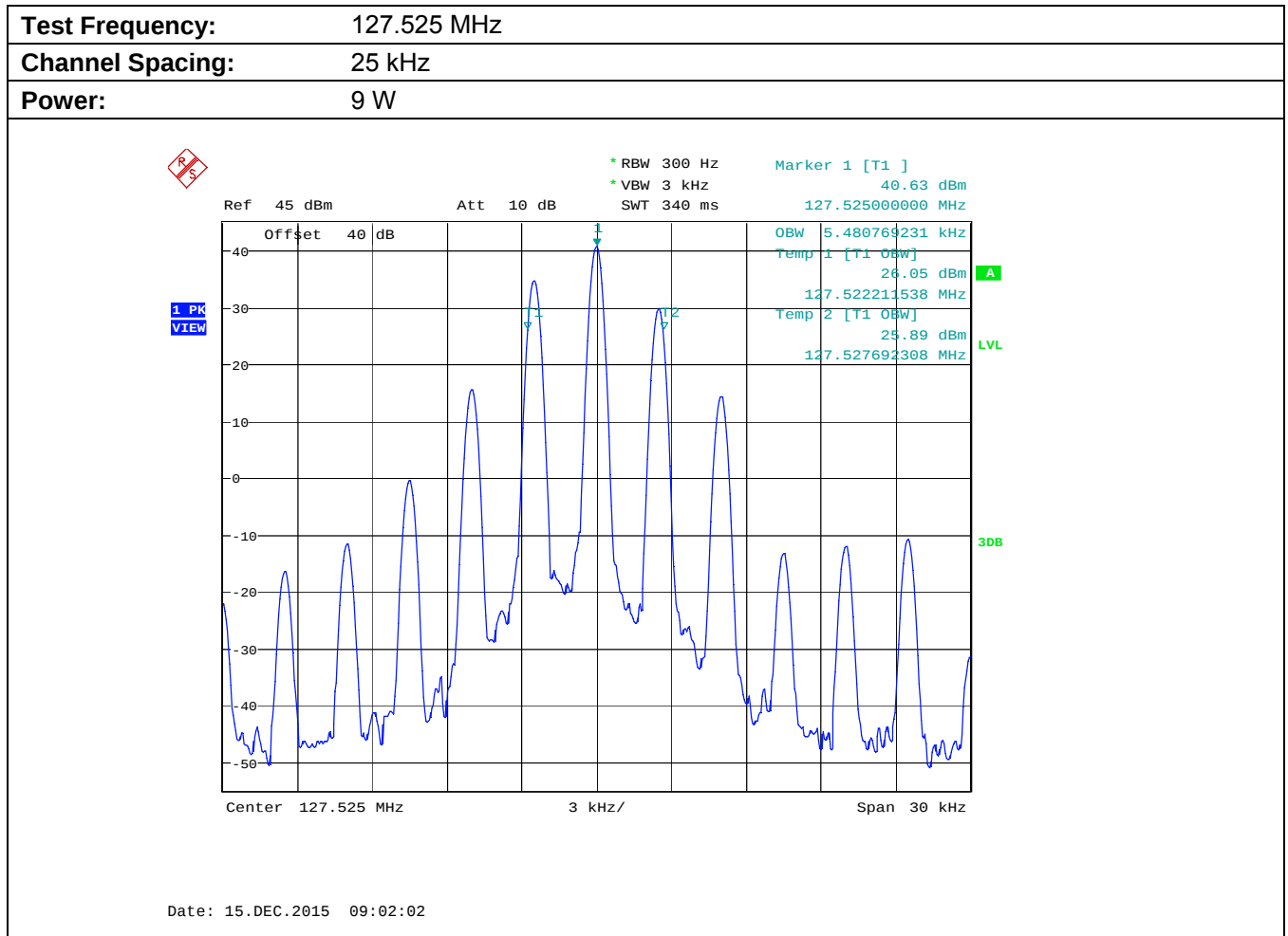
Plot 5.6.4.1.5. 99% Occupied Bandwidth
