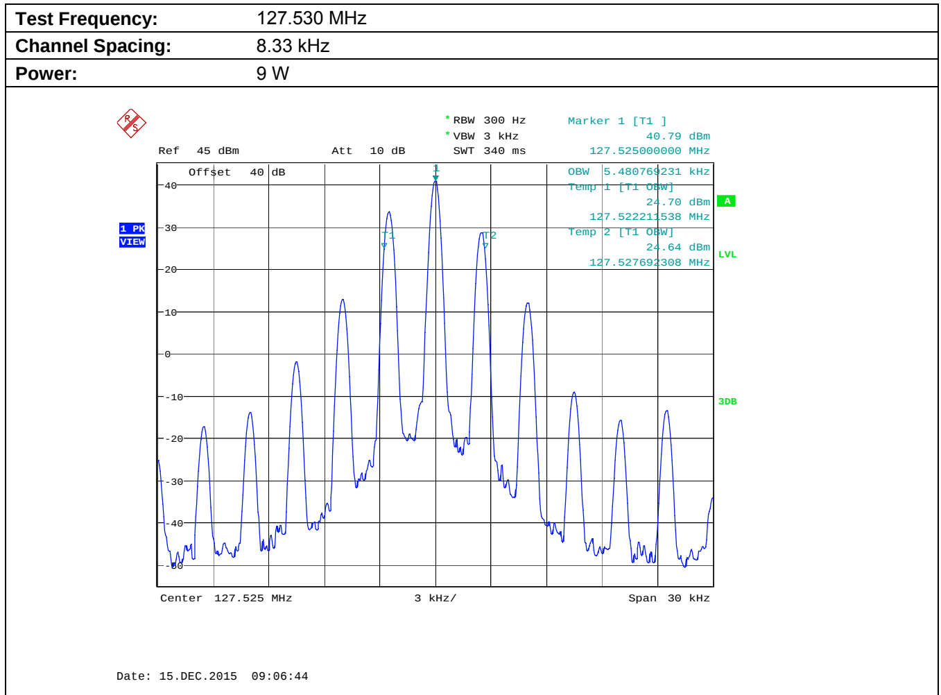
Plot 5.6.4.1.2. 99% Occupied Bandwidth
