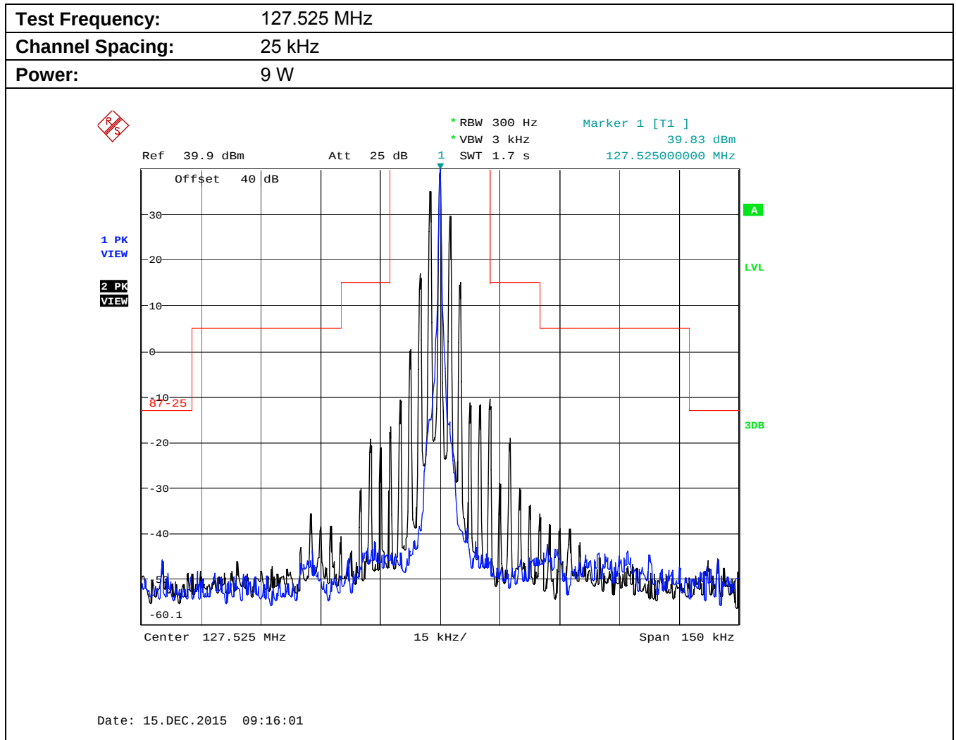
Plot 5.6.4.2.5. Emissions Limitation
