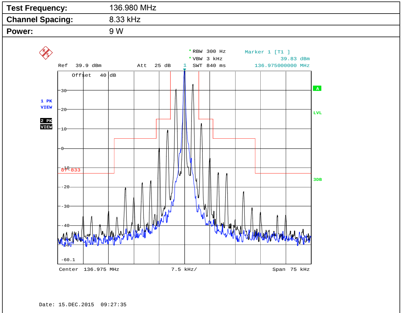
Plot 5.6.4.2.3. Emissions Limitation
