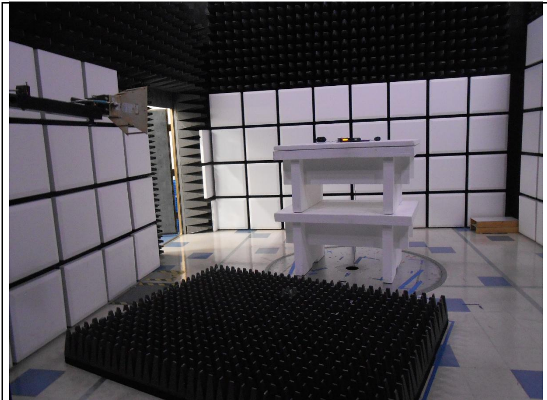
Radiated Emissions: 1 – 1.5 GHz
