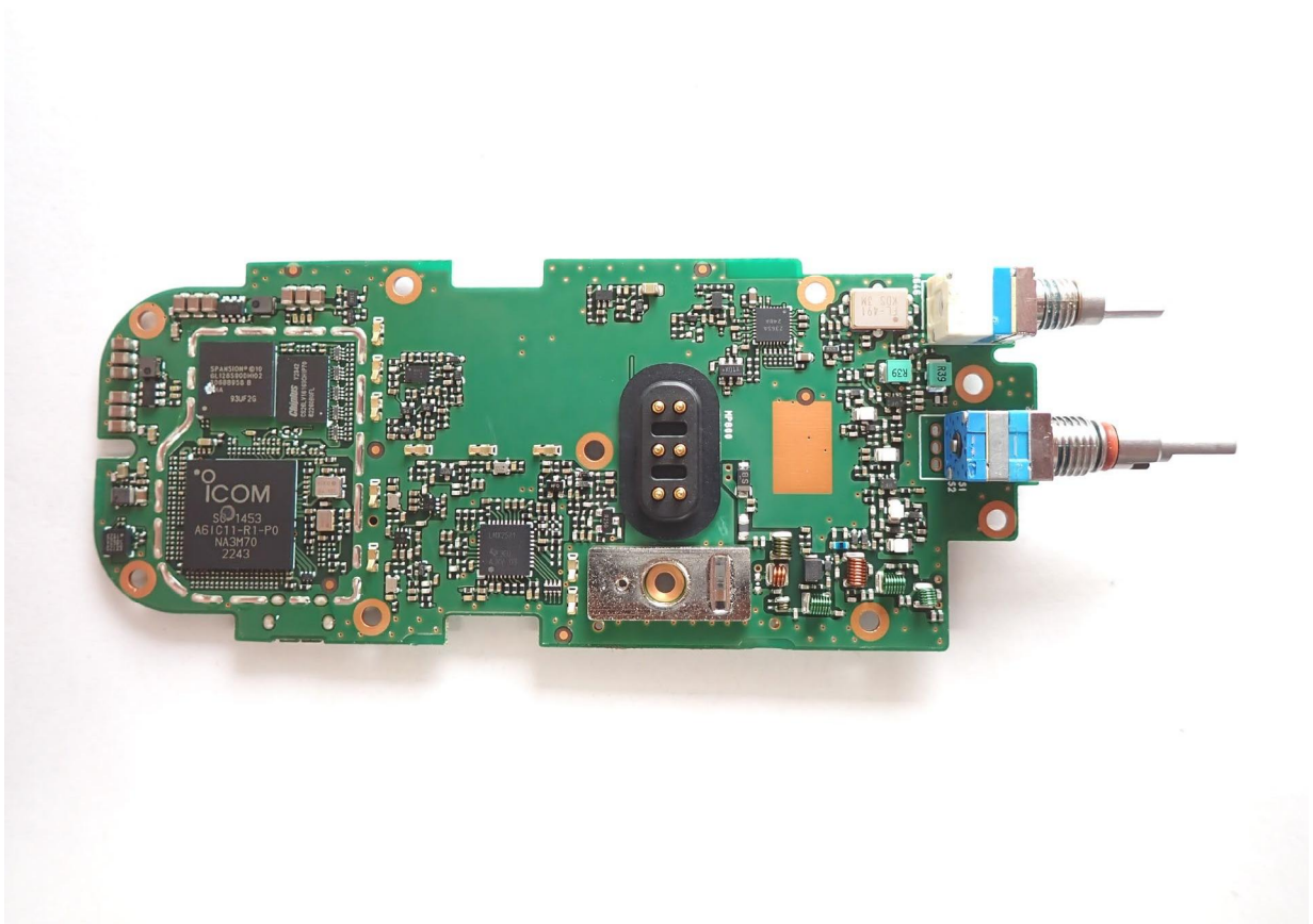
IC-F3400DT/DS MAIN SIDE B
