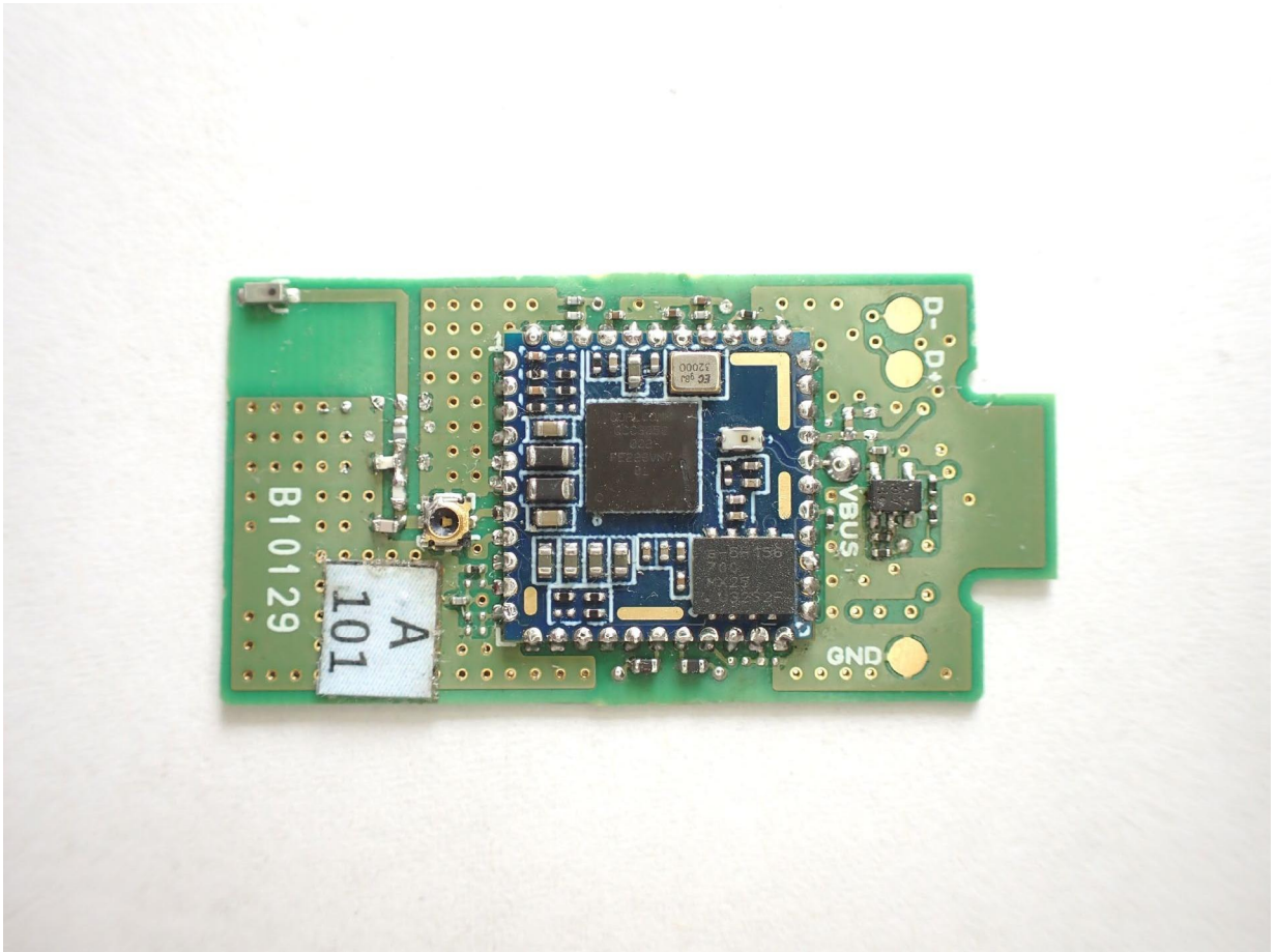
Bluetooth Unit(UT-136B) SIDE A
