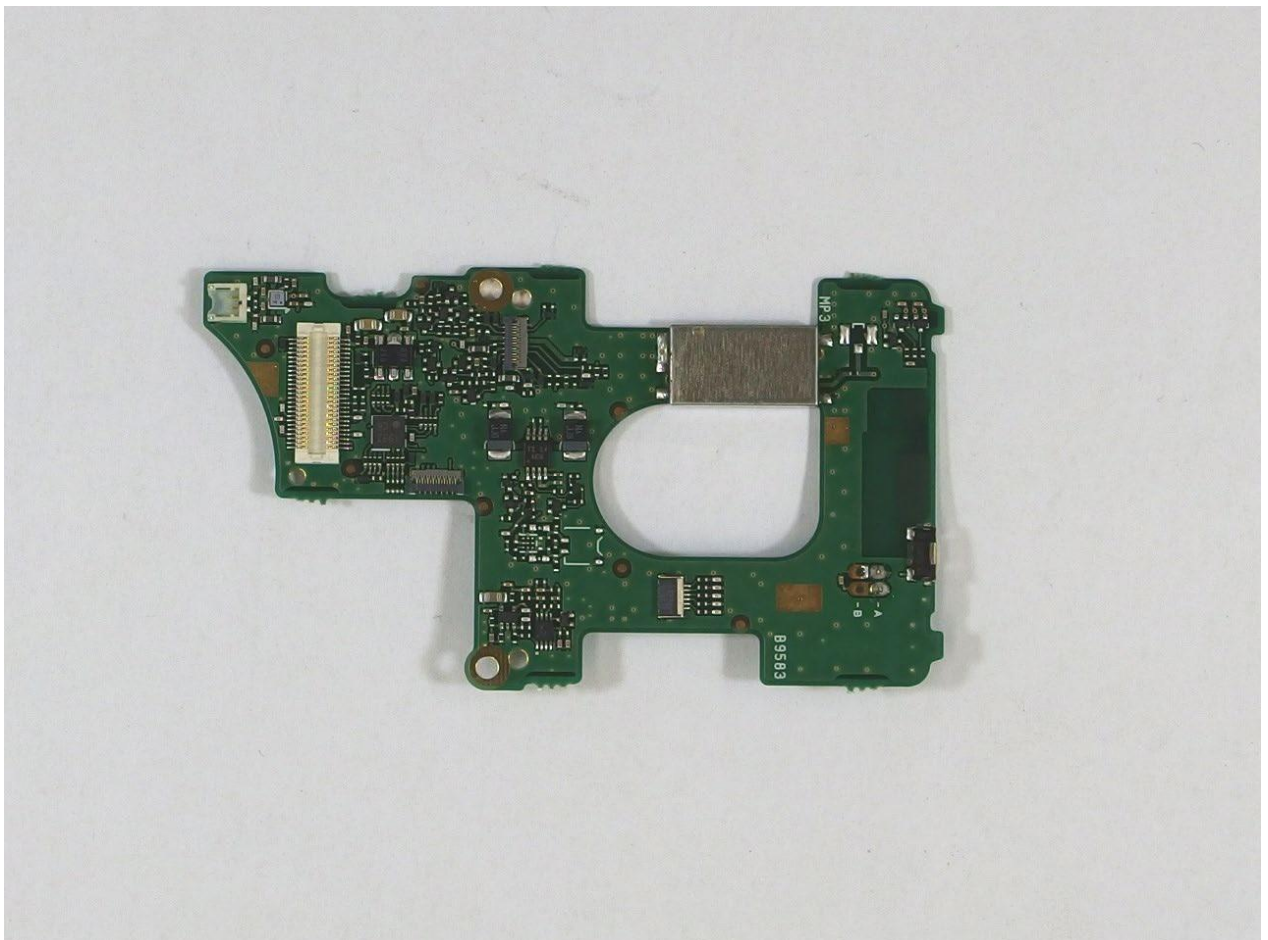
IC-F3400DT/DS FRONT SIDE B
