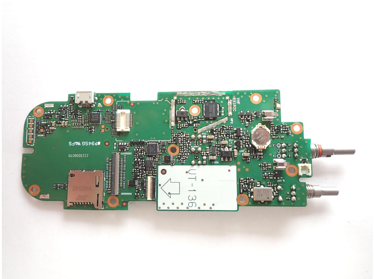
IC-F3400DT/DS MAIN SIDE A
