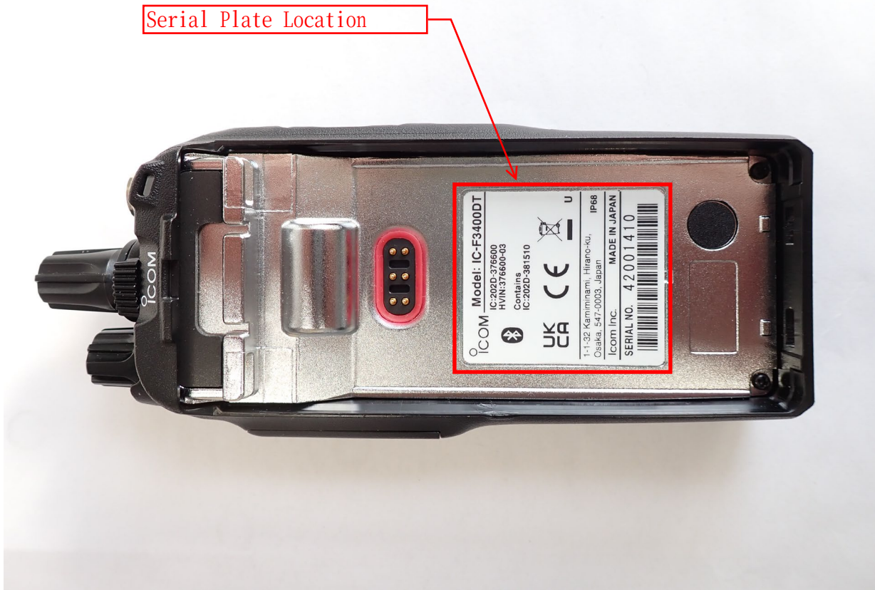
IC-F3400DT REAR SIDE
