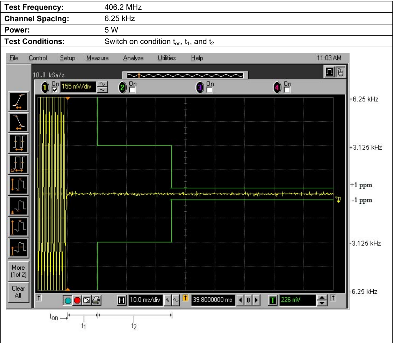
Plot 5.15.3.1. Transient Frequency Behavior for 6.25 kHz Channel Spacing
