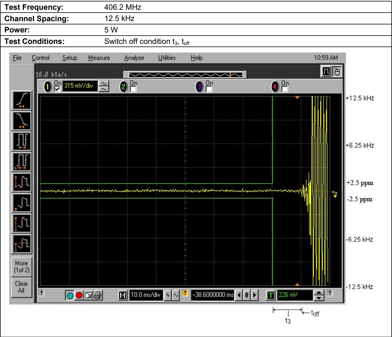
Plot 5.15.3.4. Transient Frequency Behavior for 12.5 kHz Channel Spacing
