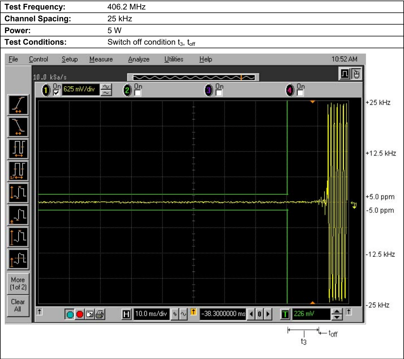
Plot 5.15.3.6. Transient Frequency Behavior for 25 kHz Channel Spacing
