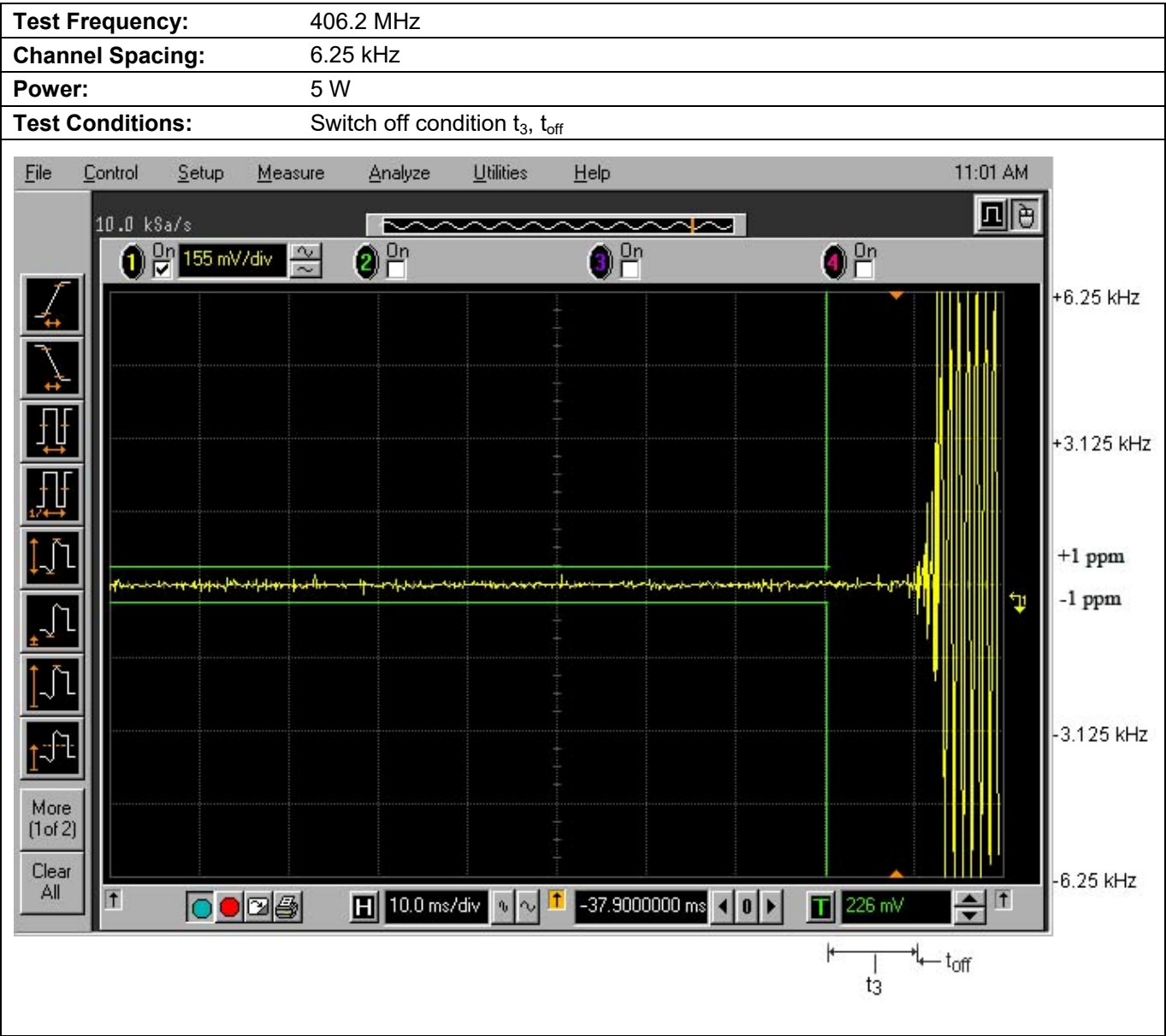
Plot 5.15.3.2. Transient Frequency Behavior for 6.25 kHz Channel Spacing
