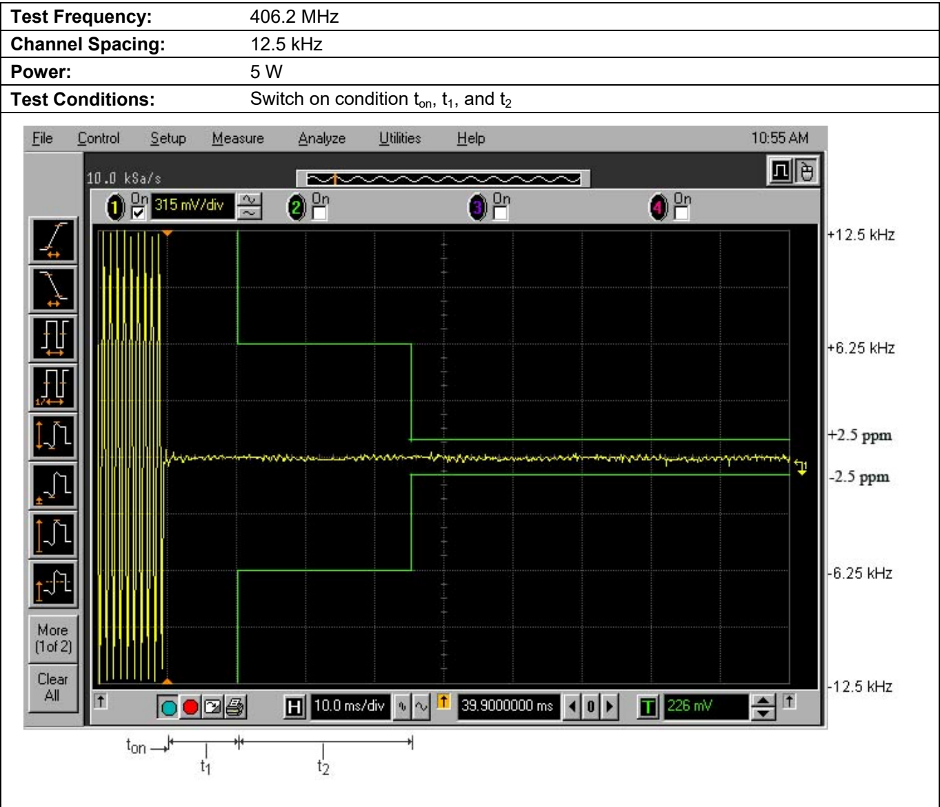
Plot 5.15.3.3. Transient Frequency Behavior for 12.5 kHz Channel Spacing
