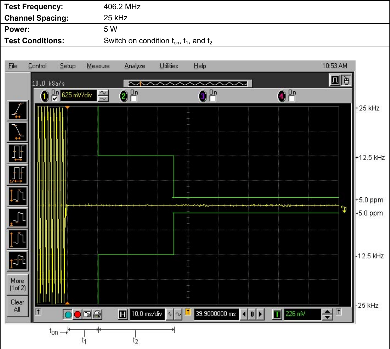
Plot 5.15.3.5. Transient Frequency Behavior for 25 kHz Channel Spacing
