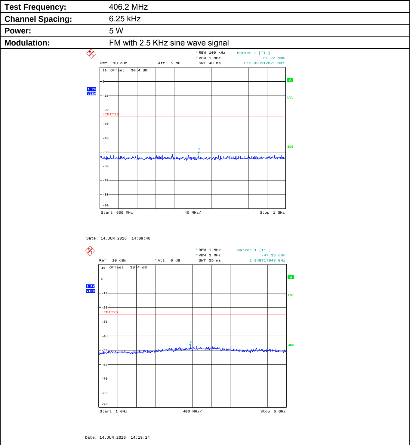
Plot 5.9.4.1.2. Conducted Transmitter Spurious Emissions for 406.2 MHz, High Power, 600 MHz - 5 GHz
