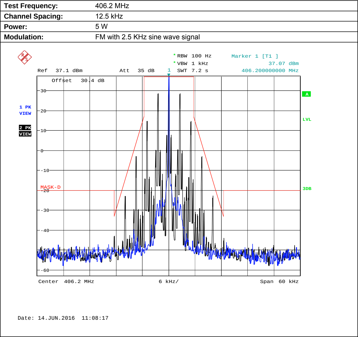
Plot 5.8.4.2.1. Emission Mask D, High Power
