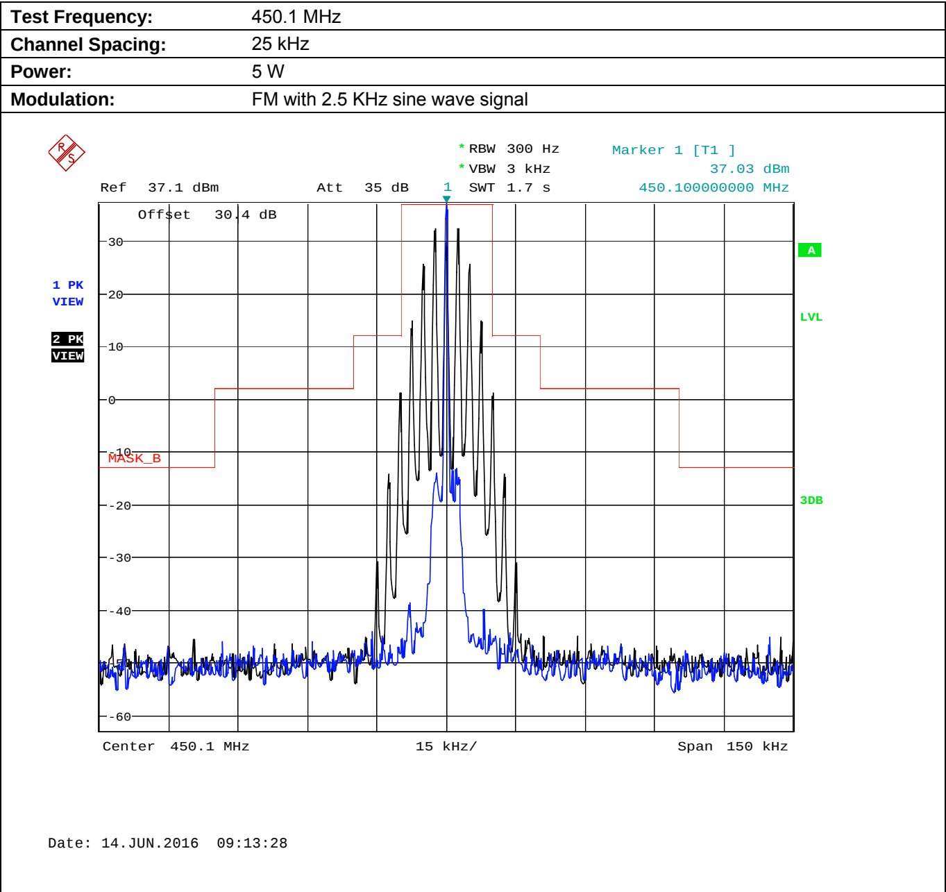
Plot 5.8.4.3.2. Emission Mask B, High Power
