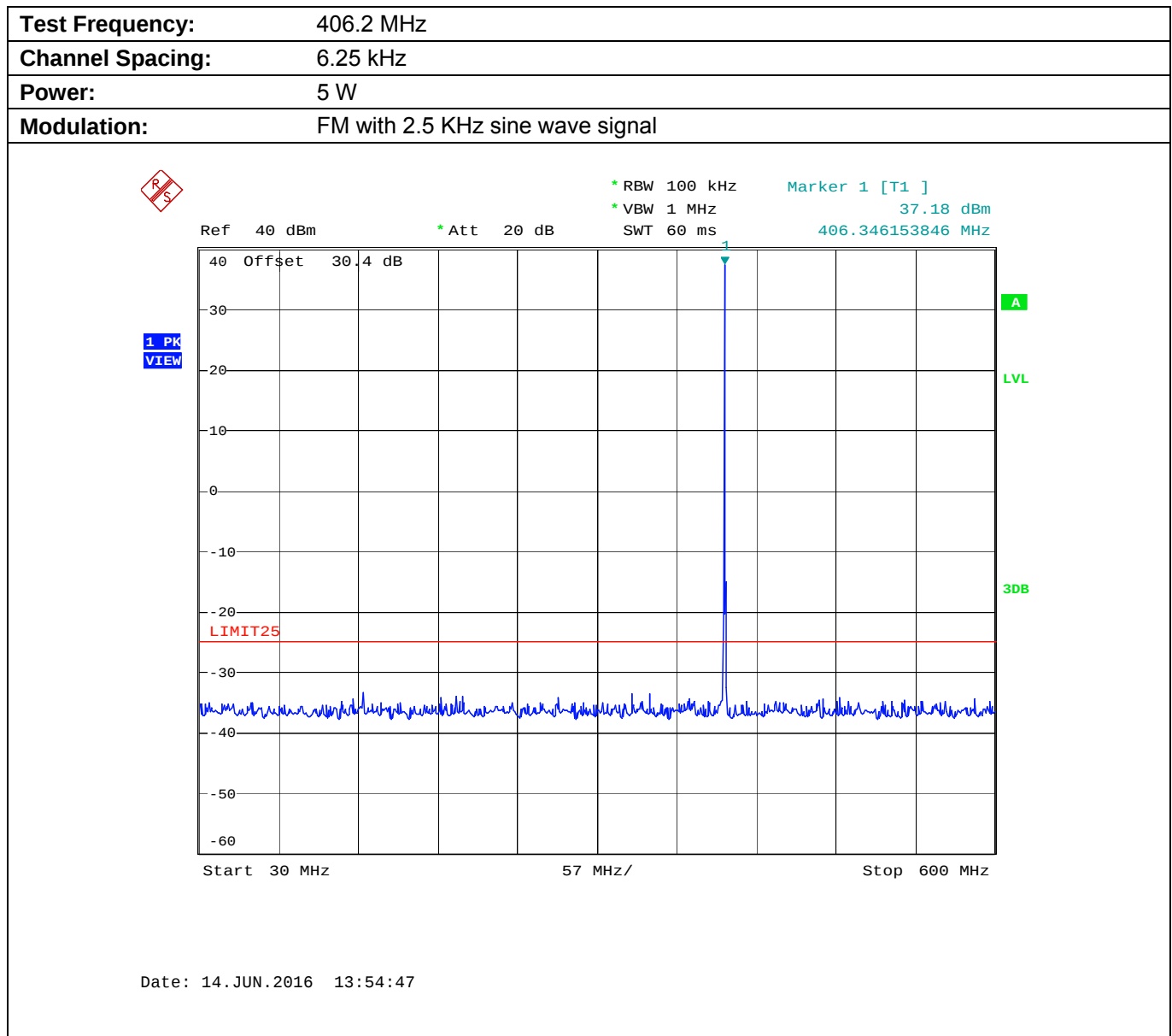
Plot 5.9.4.1.1. Conducted Transmitter Spurious Emissions for 406.2 MHz, High Power, 30 MHz - 600 MHz
