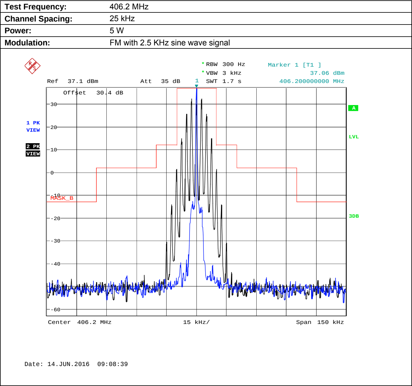
Plot 5.8.4.3.1. Emission Mask B, High Power
