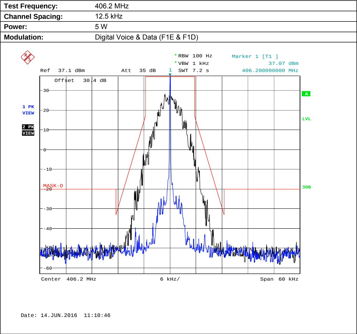
Plot 5.8.4.2.7. Emission Mask D, High Power
