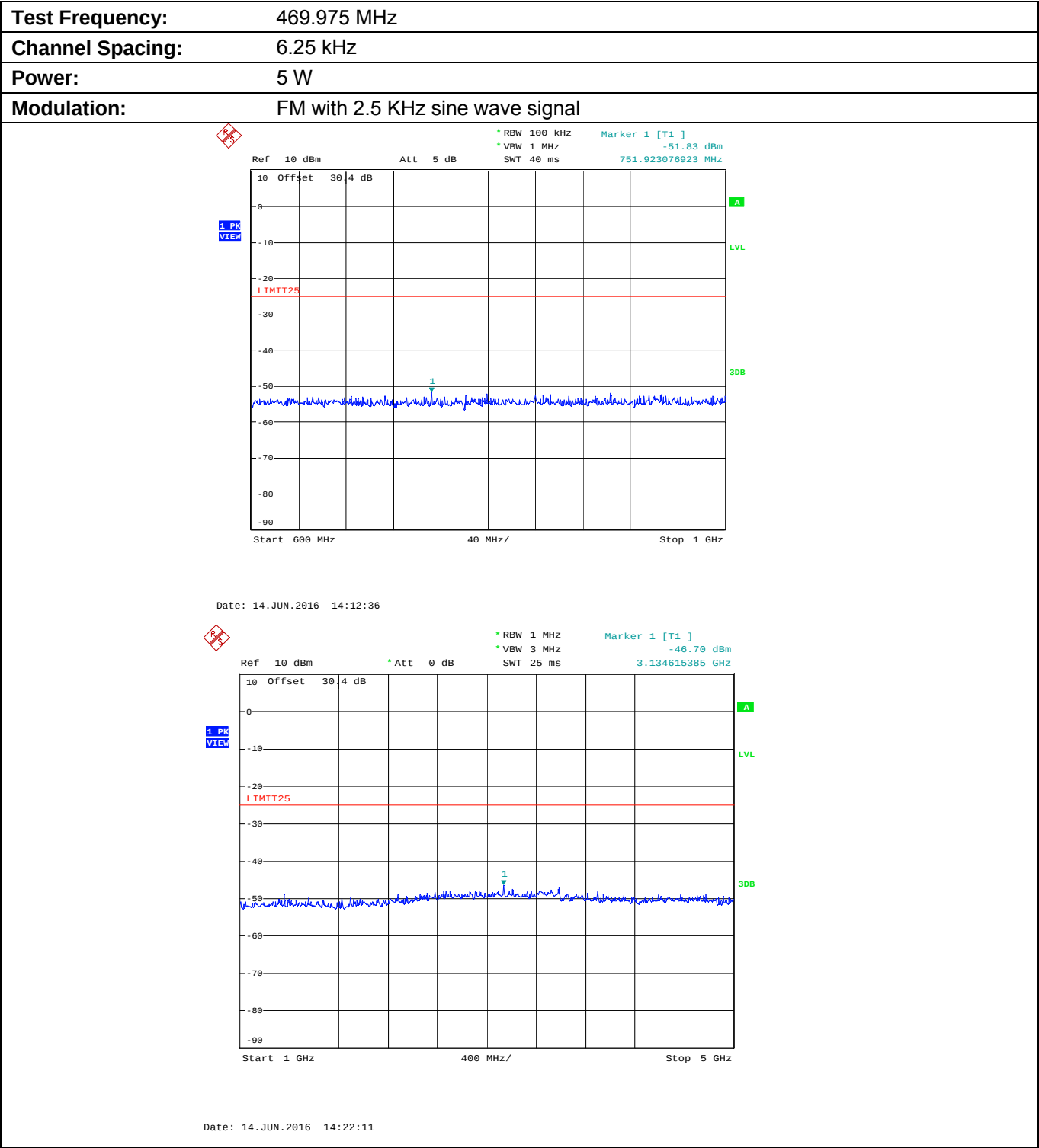
Plot 5.9.4.3.2. Conducted Transmitter Spurious Emissions for 469.975 MHz, High Power, 600 MHz - 5 GHz
