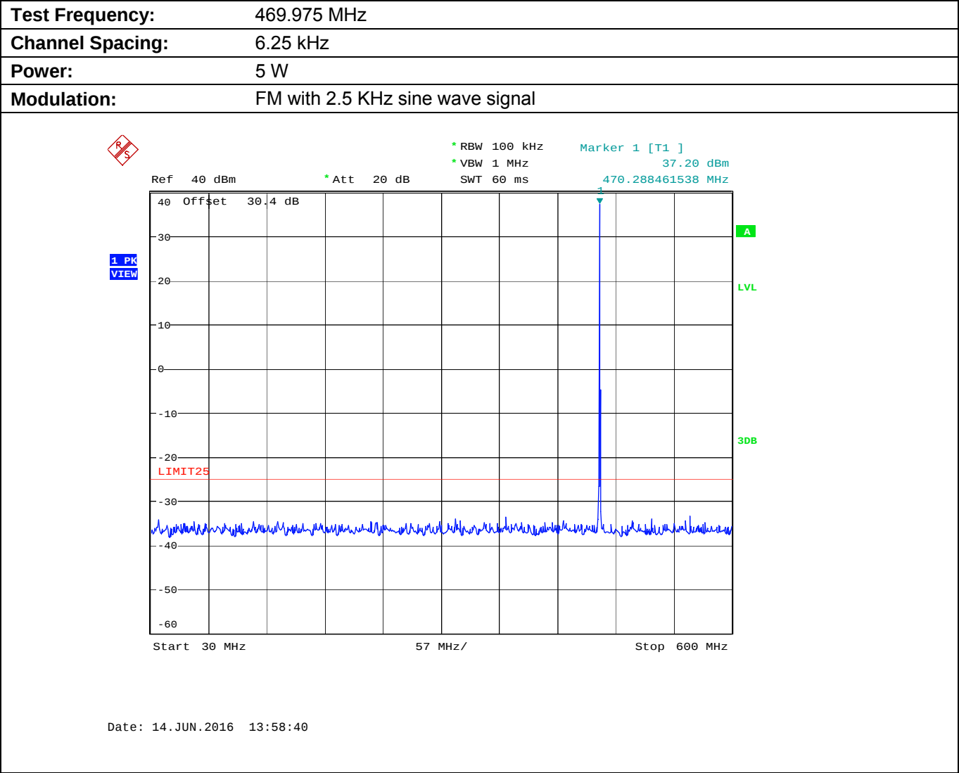
Plot 5.9.4.3.1. Conducted Transmitter Spurious Emissions for 469.975 MHz, High Power, 30 MHz - 600 MHz
