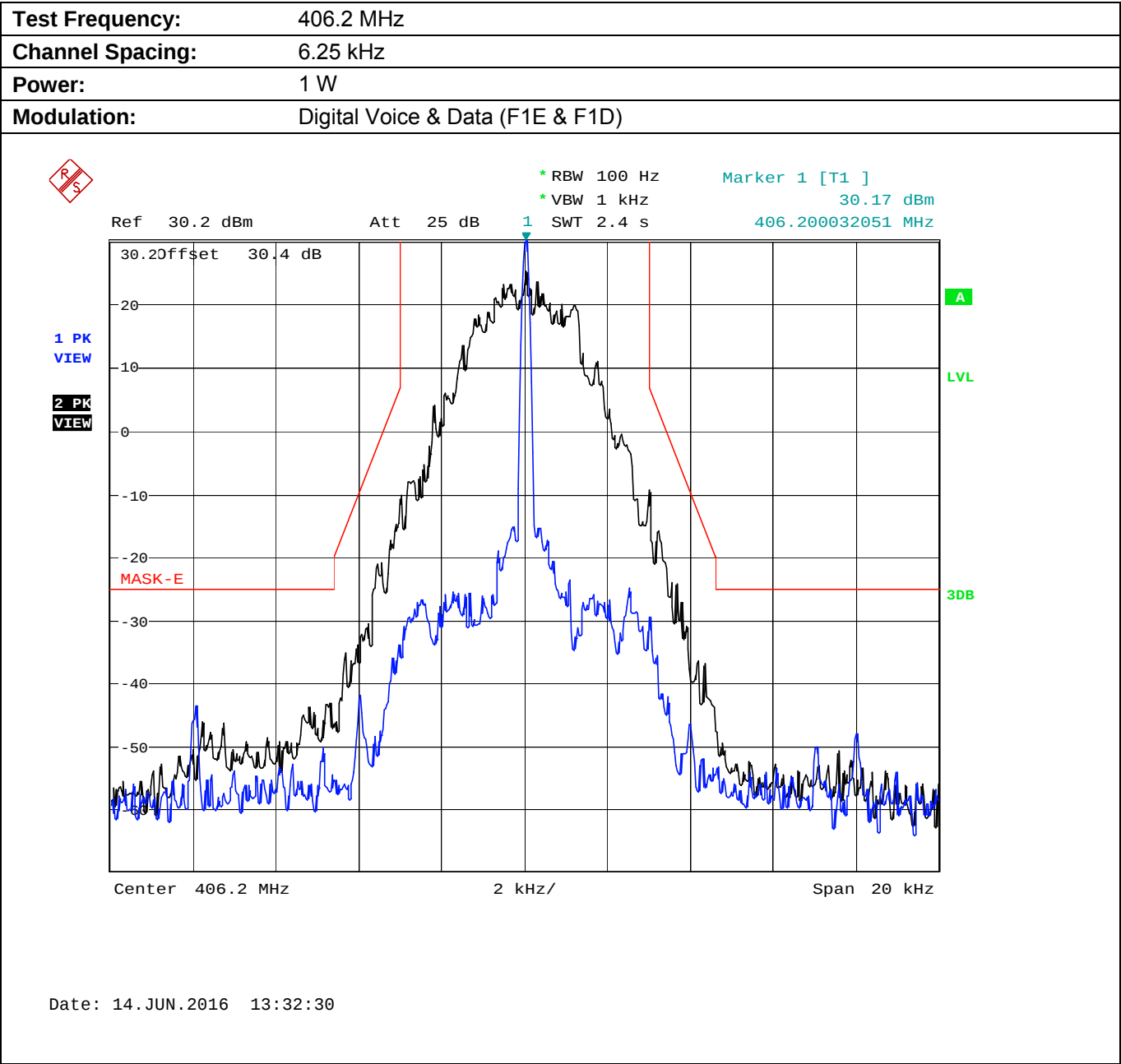
Plot 5.8.4.4. Emission Mask E, Low Power
