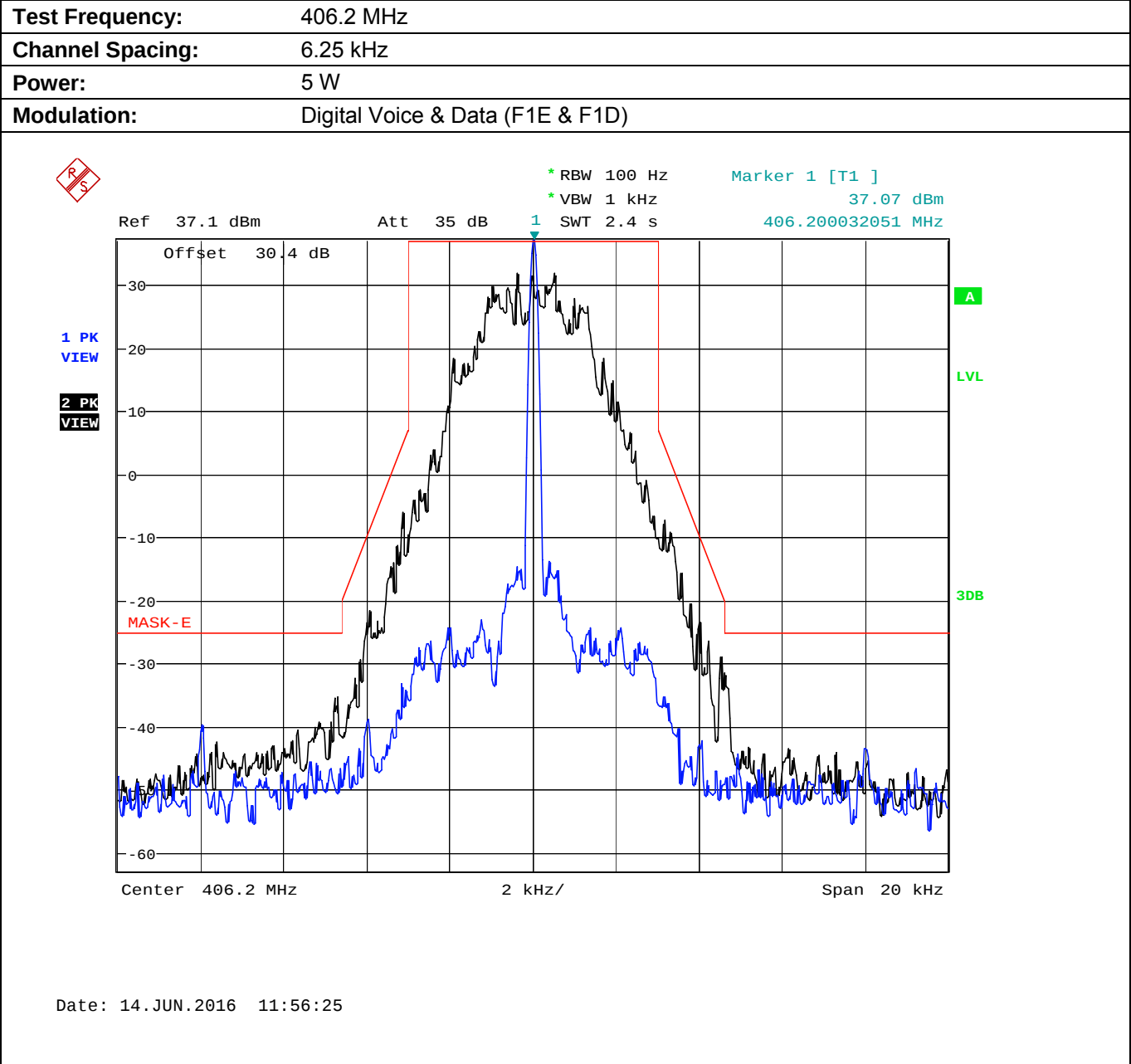
Plot 5.8.4.4.1. Emission Mask E, High Power
