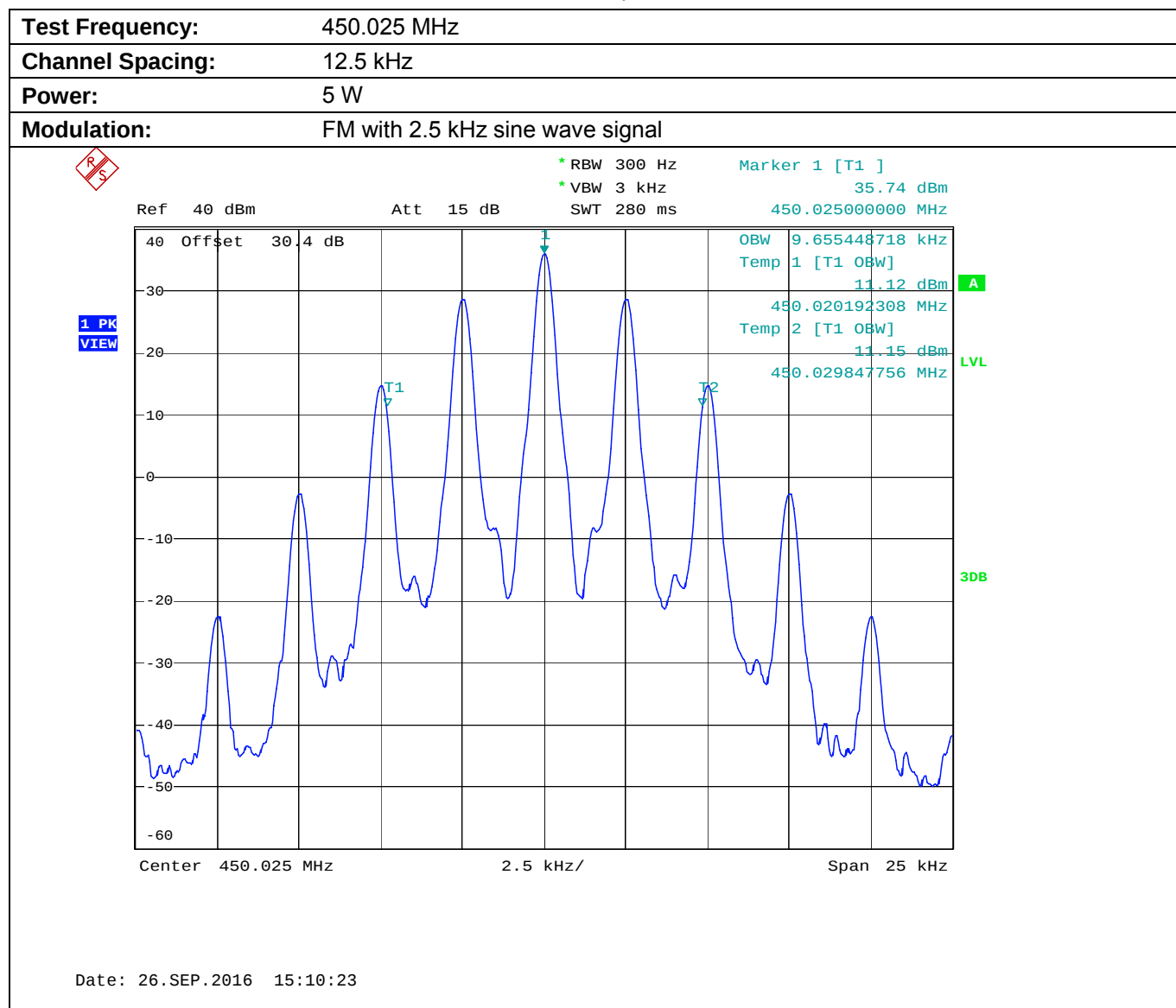
Plot 5.8.4.1.1. Occupied Bandwidth
