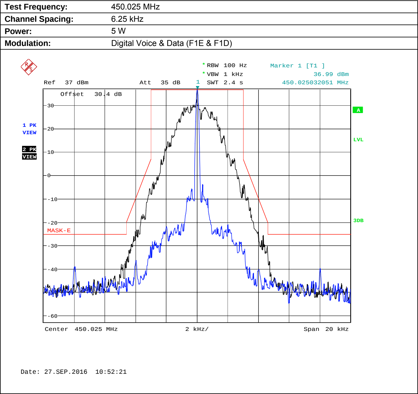
Plot 5.8.4.4.1. Emission Mask E, High Power
