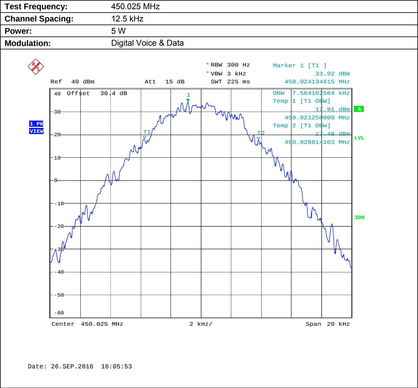
Plot 5.8.4.1.7. Occupied Bandwidth
