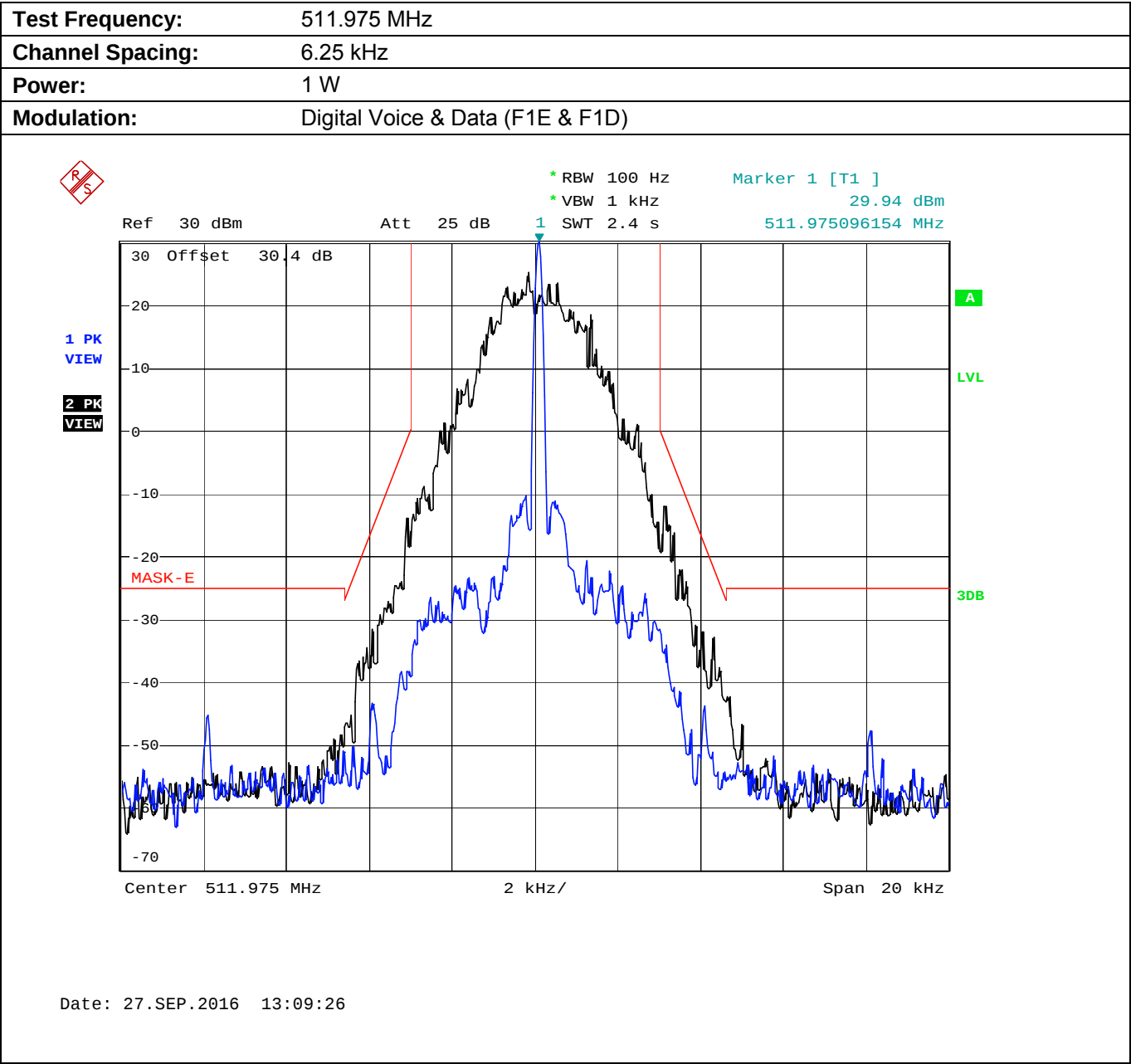
Plot 5.8.4.4.6. Emission Mask E, Low Power
