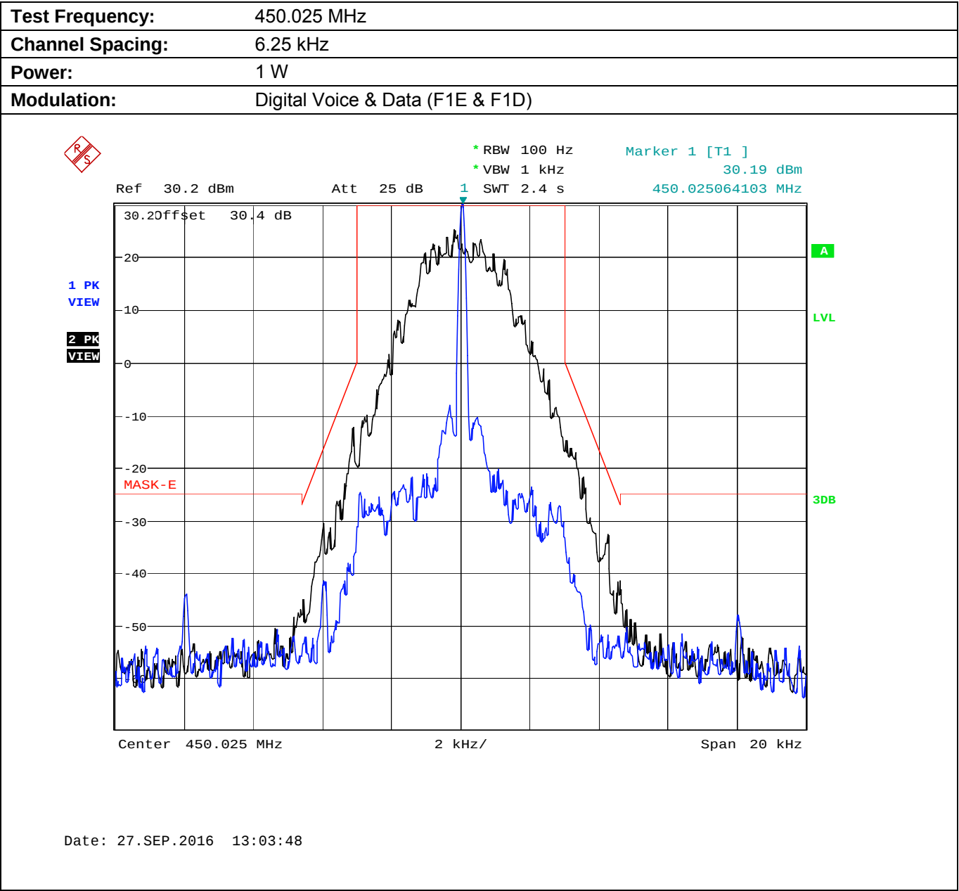
Plot 5.8.4.4. Emission Mask E, Low Power
