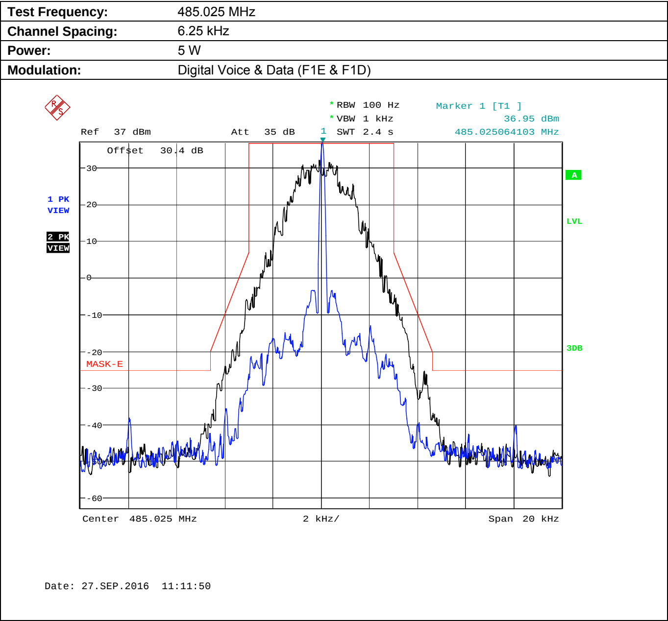
Plot 5.8.4.4.2. Emission Mask E, High Power
