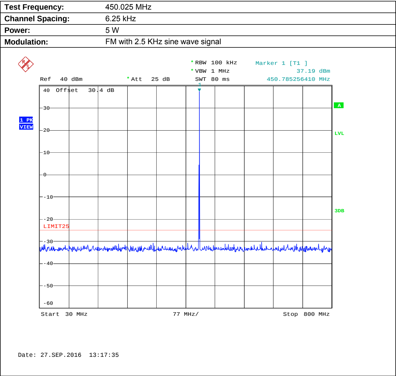
Plot 5.9.4.1.1. Conducted Transmitter Spurious Emissions for 450.025 MHz, High Power, 30 MHz - 800 MHz
