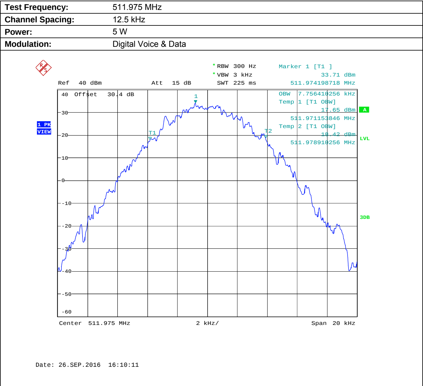
Plot 5.8.4.1.9. Occupied Bandwidth
