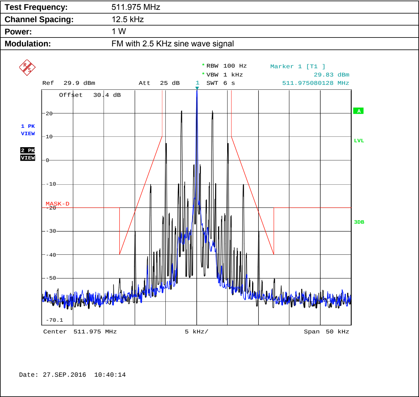
Plot 5.8.4.2.6. Emission Mask D, Low Power
