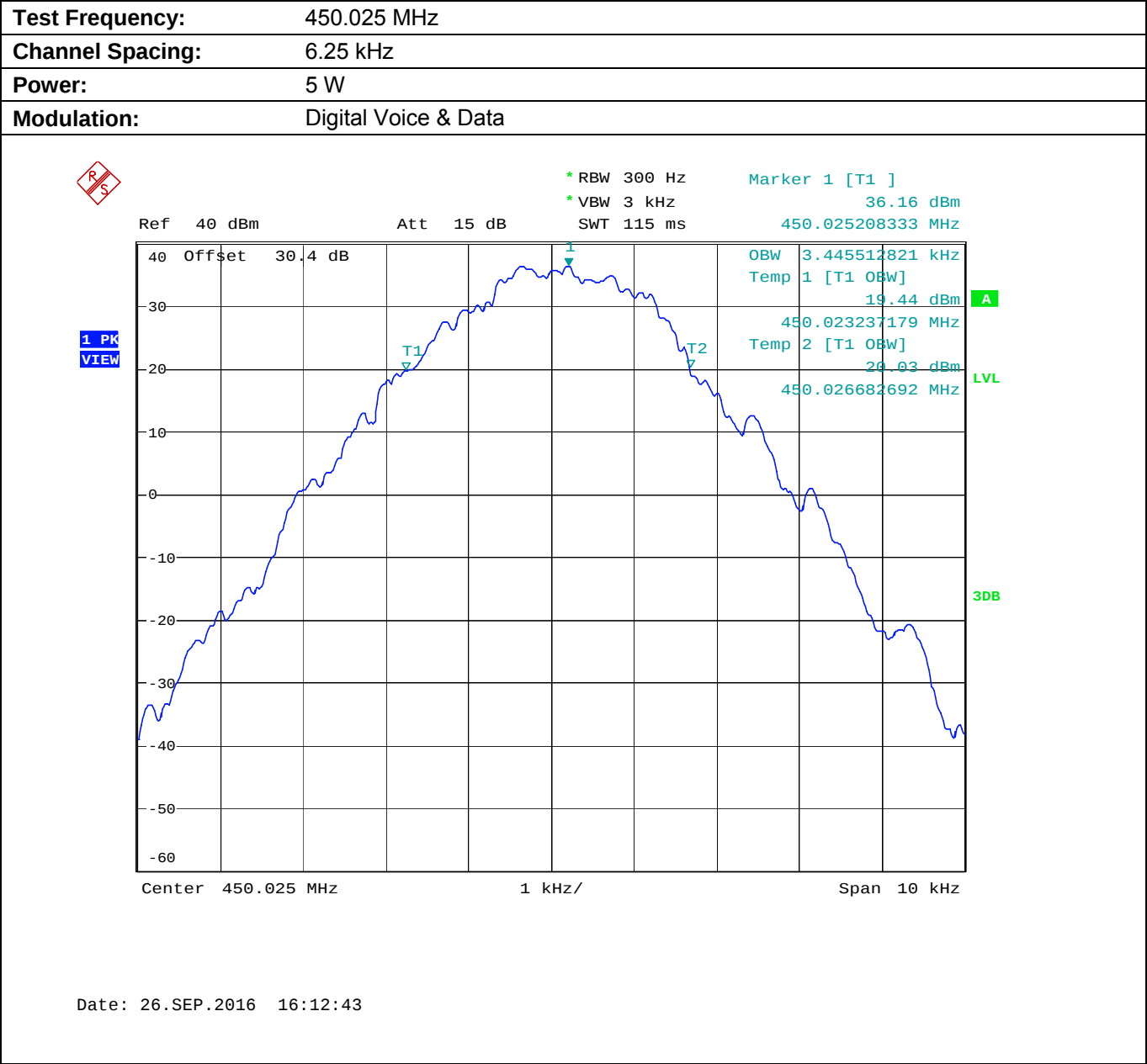
Plot 5.8.4.1.10. Occupied Bandwidth
