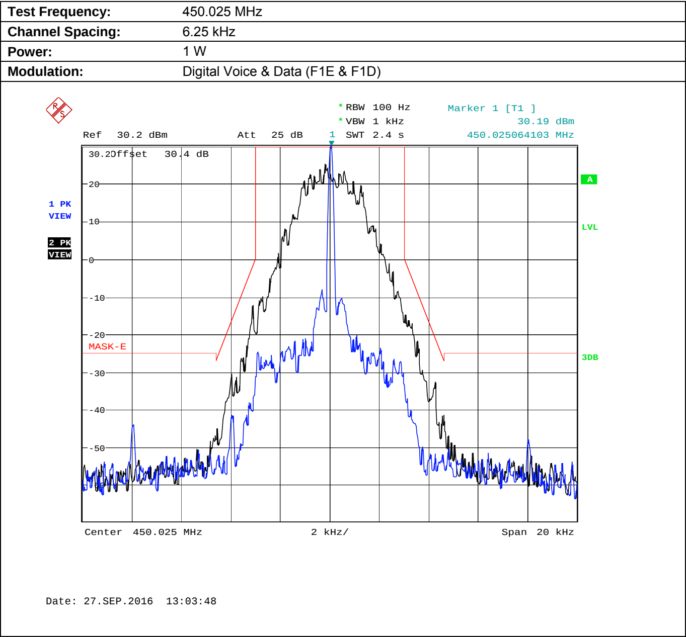
Plot 5.8.4.4.4. Emission Mask E, Low Power
