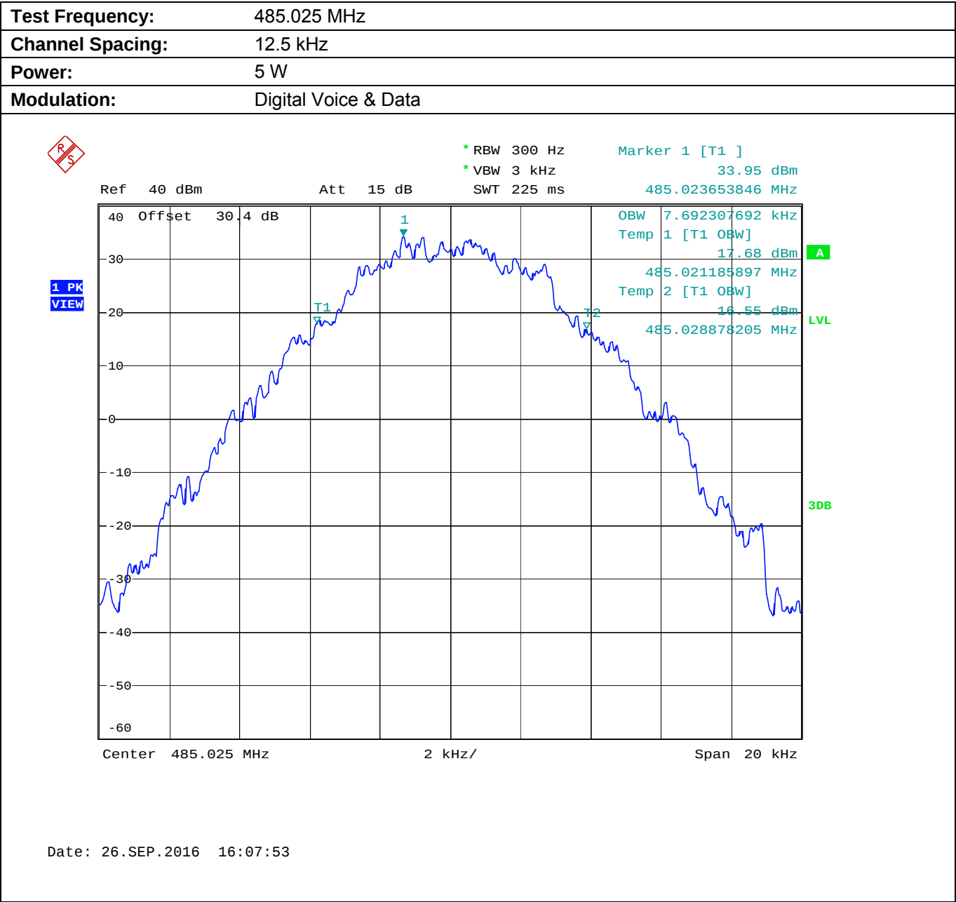
Plot 5.8.4.1.8. Occupied Bandwidth
