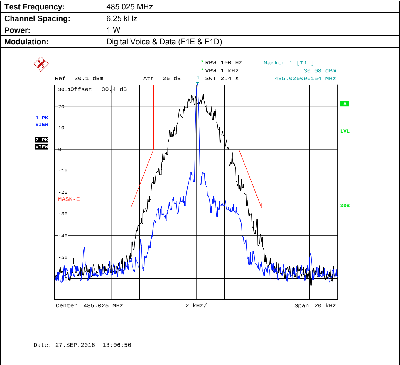
Plot 5.8.4.4.5. Emission Mask E, Low Power
