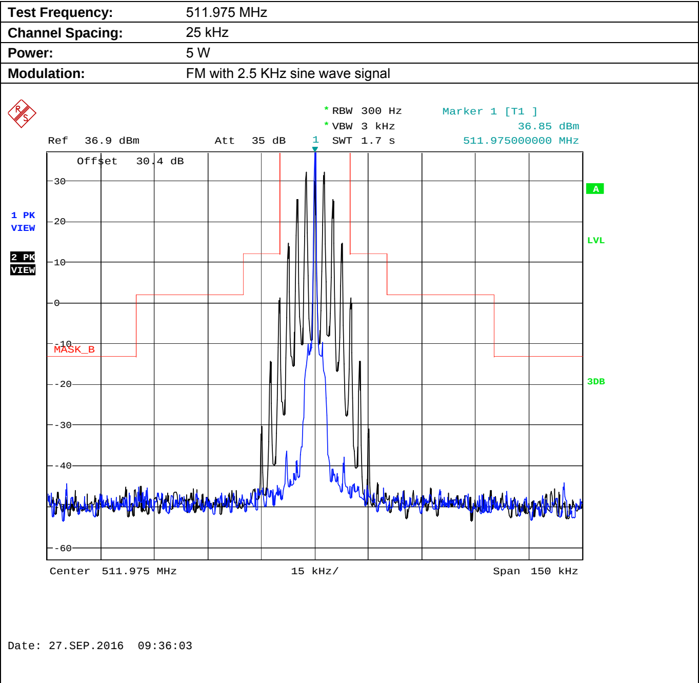
Plot 5.8.4.3.3. Emission Mask B, High Power
