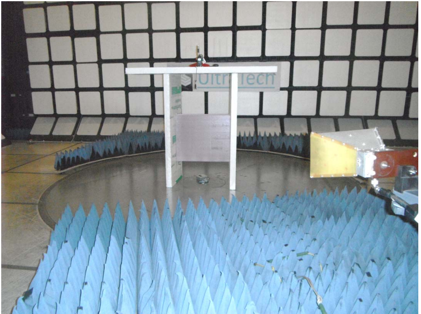
Plot #3: Tx Radiated Emission Test Setup
