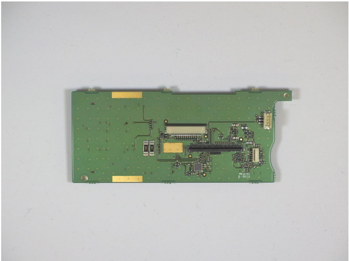
IC-F6400D FRONT-C BOARD SIDE-A
