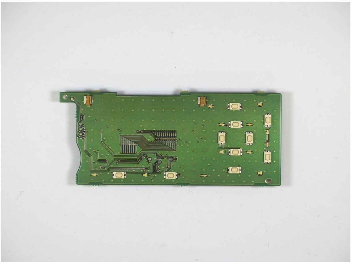
IC-F6400D FRONT-C BOARD SIDE-B
