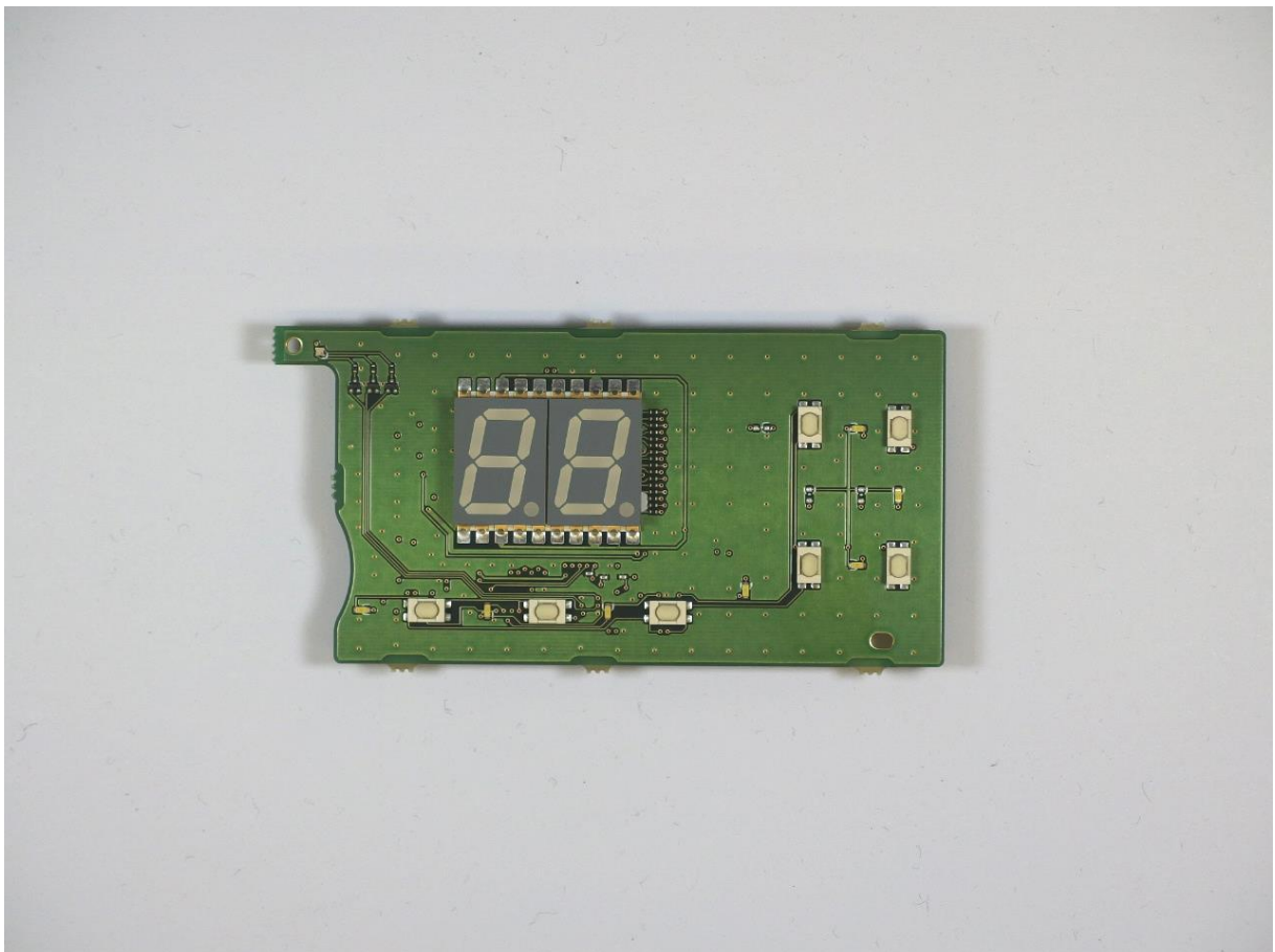
IC-F6400DS FRONT-D BOARD SIDE-B
