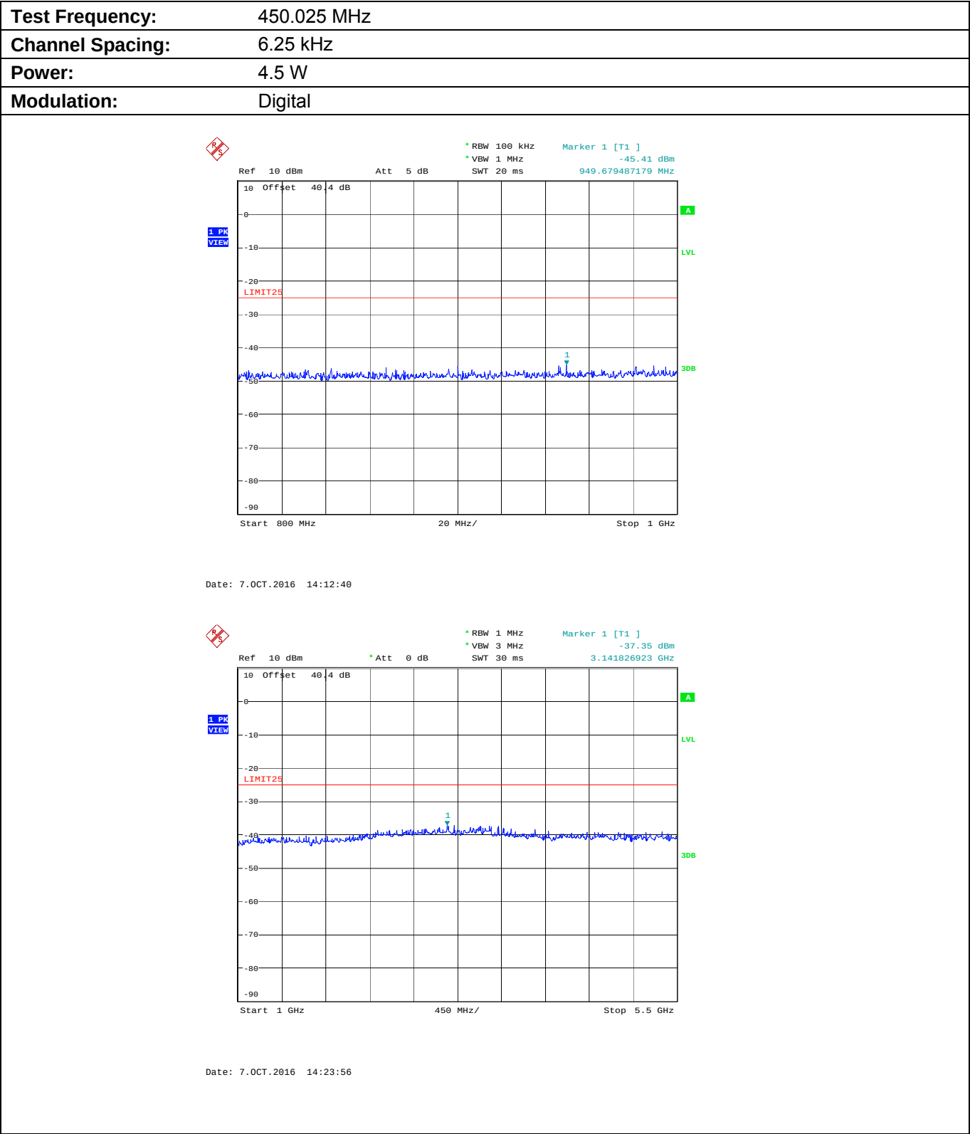
Plot 5.9.4.1.4. Conducted Transmitter Spurious Emissions for 450.025 MHz, Low Power, 0.8 - 5.5 GHz
