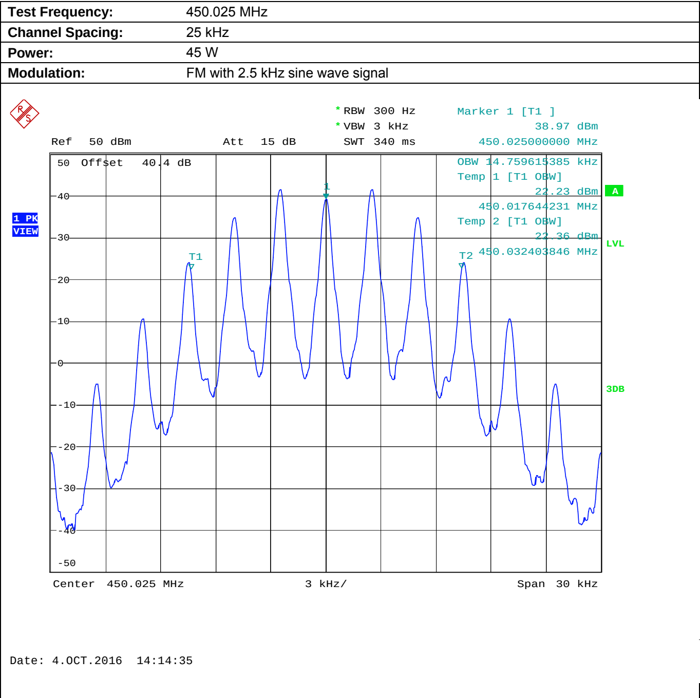
Plot 5.8.4.1.1. Occupied Bandwidth
