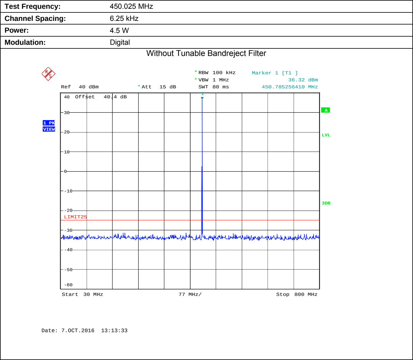
Plot 5.9.4.1.3. Conducted Transmitter Spurious Emissions for 450.025 MHz, Low Power, 30 - 800 MHz
