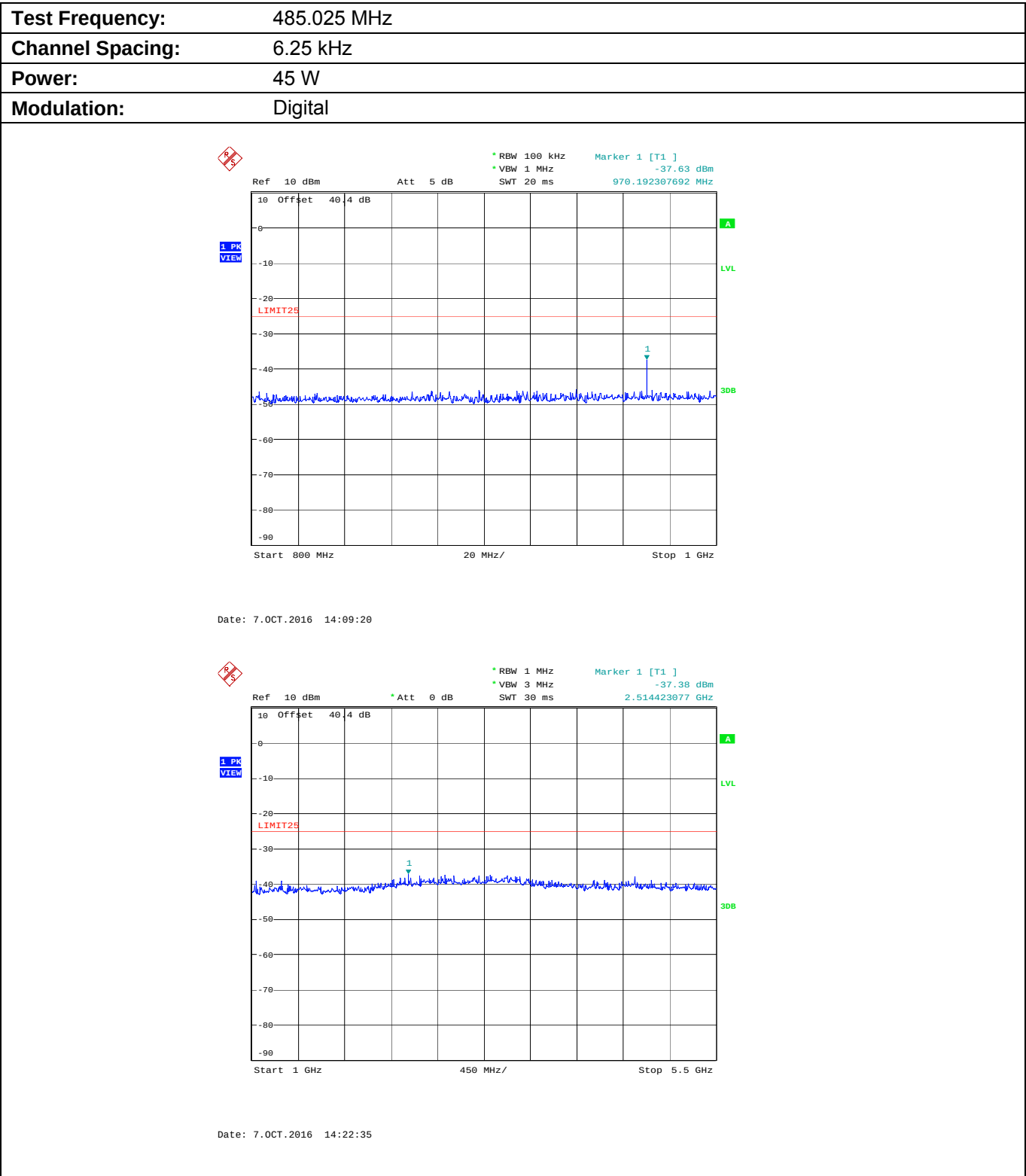
Plot 5.9.4.2.2. Conducted Transmitter Spurious Emissions for 485.025 MHz, High Power, 0.8 - 5.5 GHz
