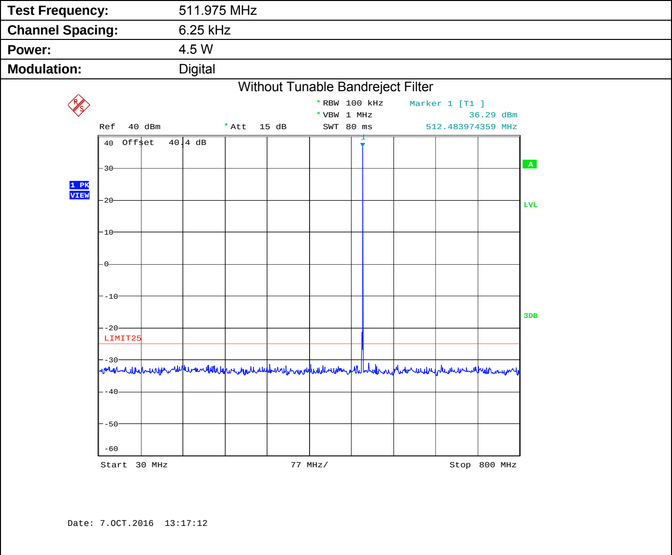
Plot 5.9.4.3.3. Conducted Transmitter Spurious Emissions for 511.975 MHz, Low Power, 30 - 800 MHz
