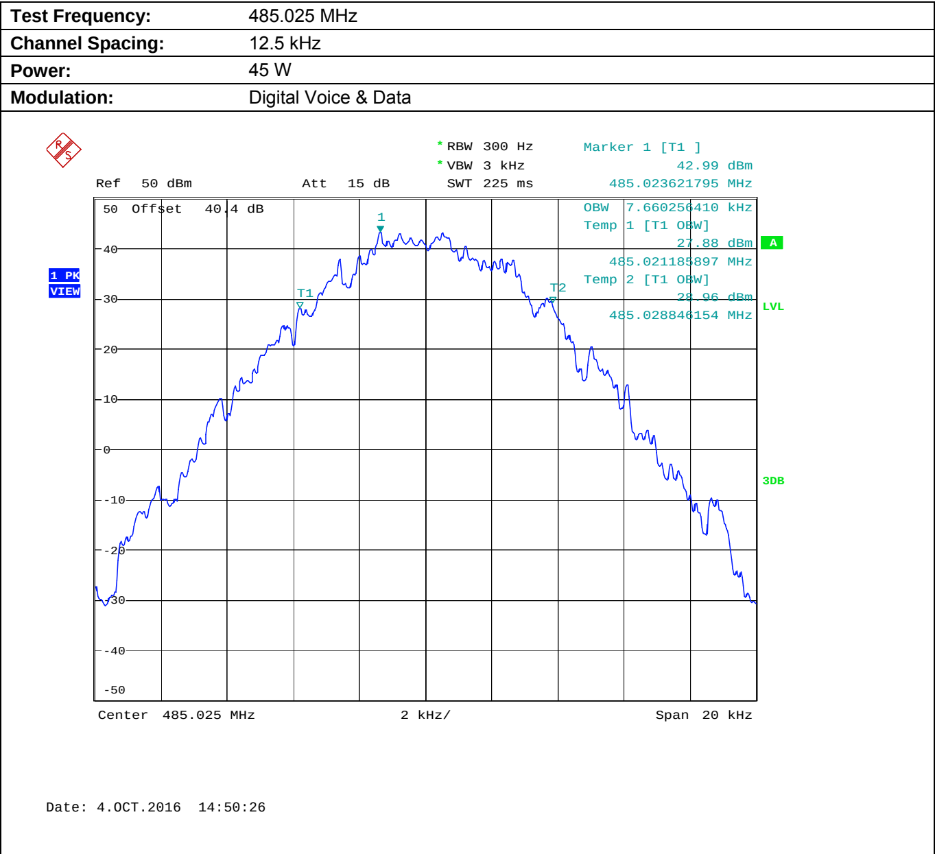
Plot 5.8.4.1.8. Occupied Bandwidth
