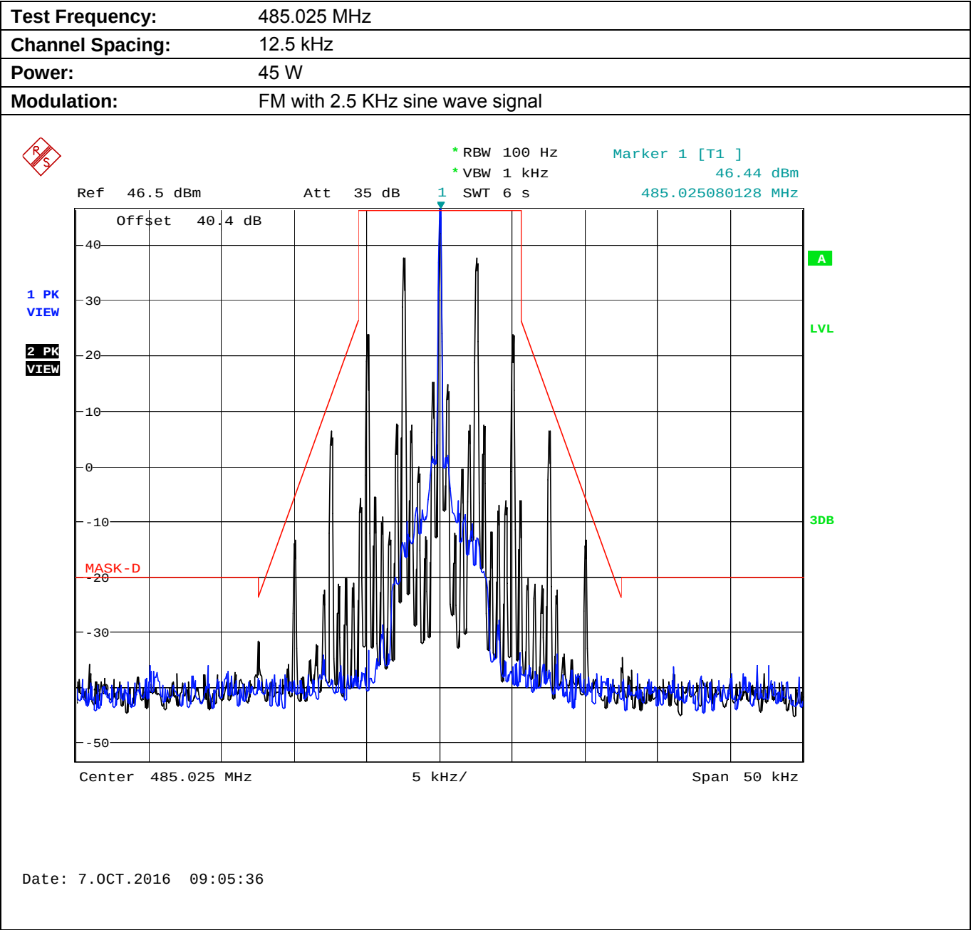
Plot 5.8.4.2.2. Emission Mask D, High Power
