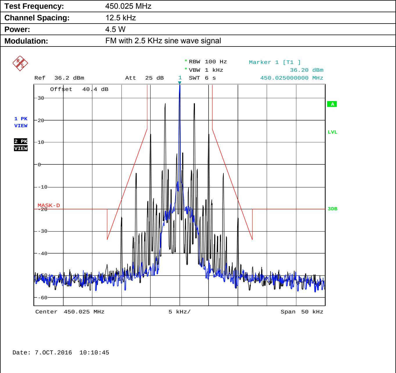
Plot 5.8.4.2.4. Emission Mask D, Low Power
