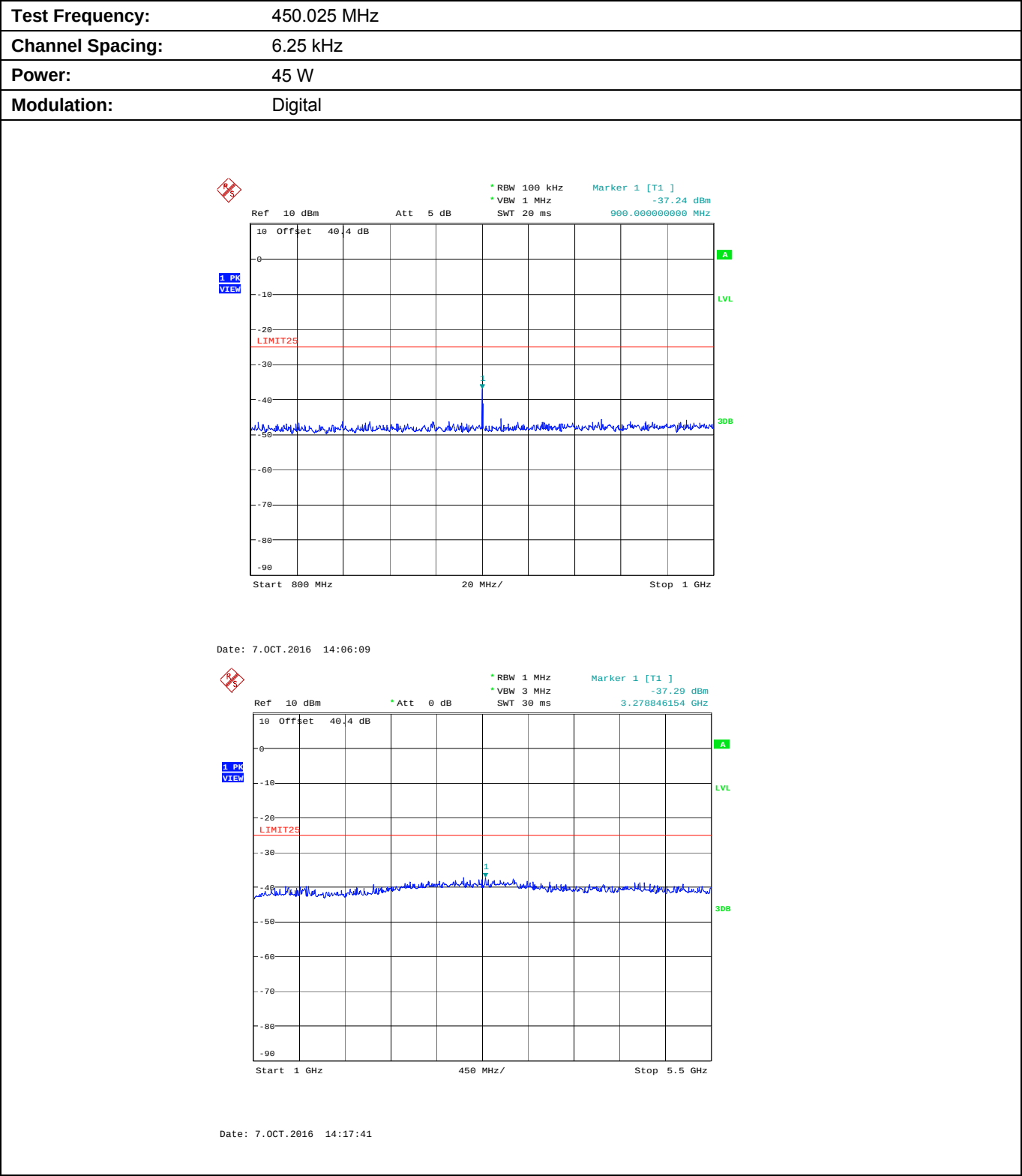
Plot 5.9.4.1.2. Conducted Transmitter Spurious Emissions for 450.025 MHz, High Power, 0.8 - 5.5 GHz
