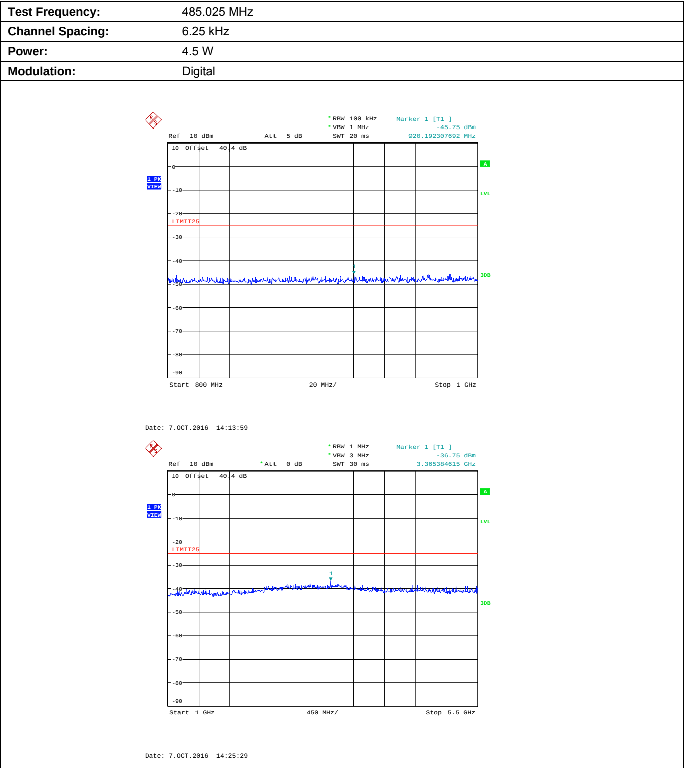
Plot 5.9.4.2.4. Conducted Transmitter Spurious Emissions for 485.025 MHz, Low Power, 0.8 - 5.5 GHz
