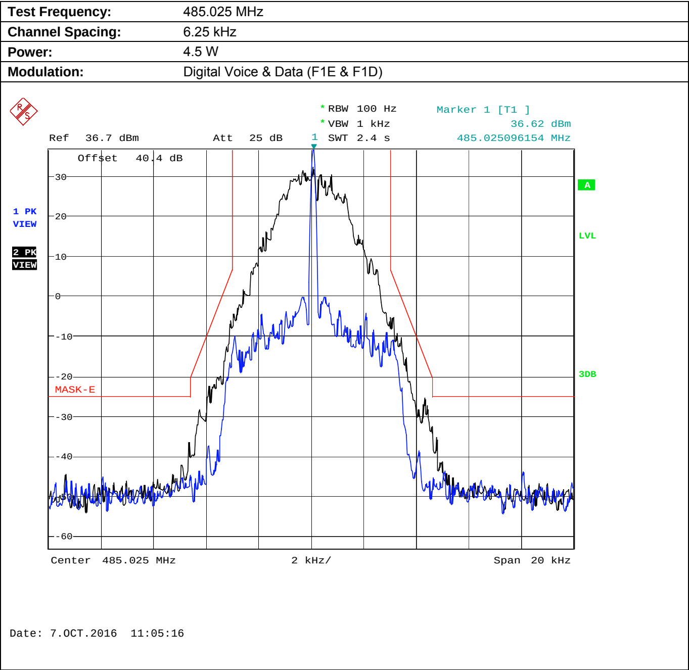
Plot 5.8.4.4.5. Emission Mask E, Low Power
