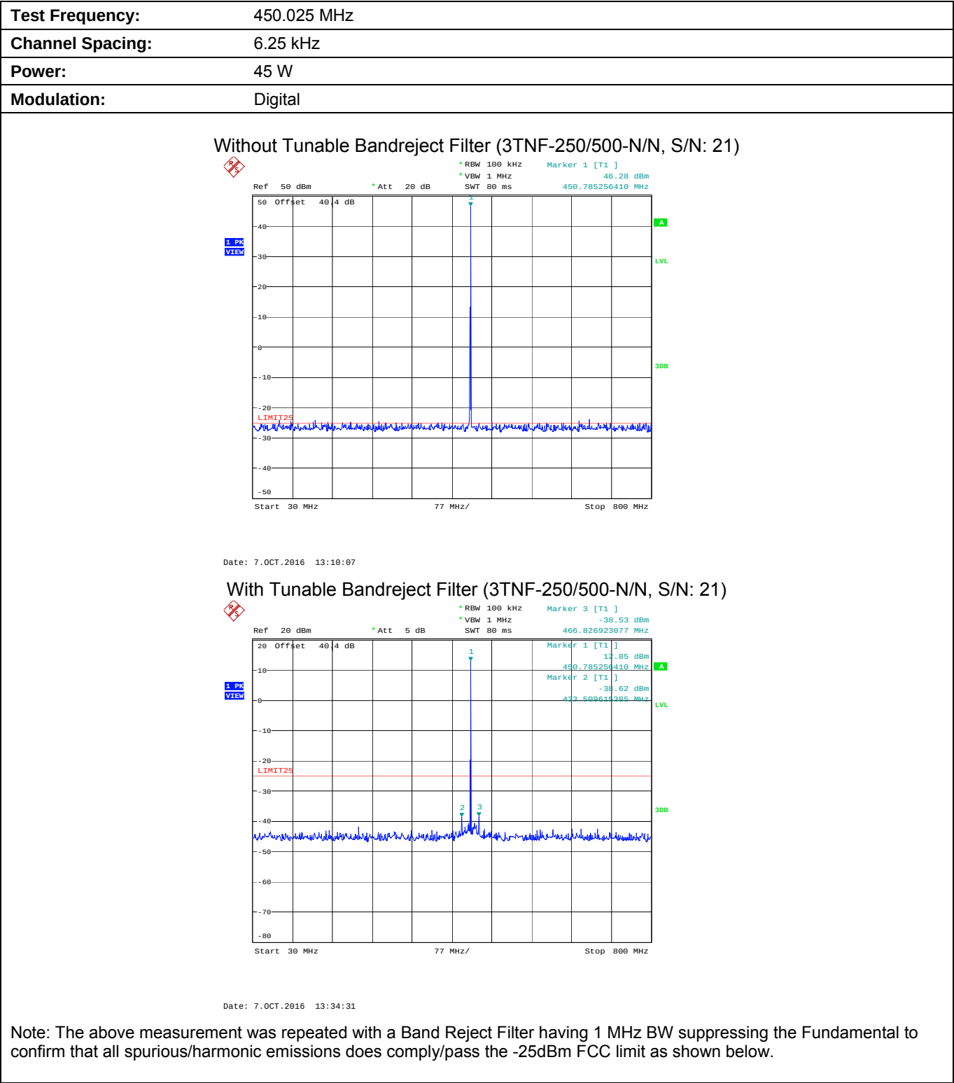
Plot 5.9.4.1.1. Conducted Transmitter Spurious Emissions for 450.025 MHz, High Power, 30 - 800 MHz
