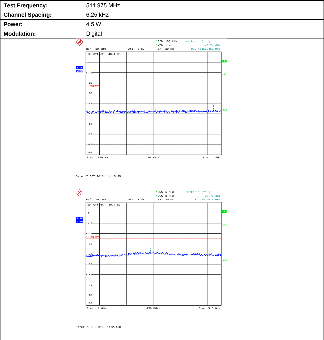
Plot 5.9.4.3.4. Conducted Transmitter Spurious Emissions for 511.975 MHz, Low Power, 0.8 - 5.5 GHz
