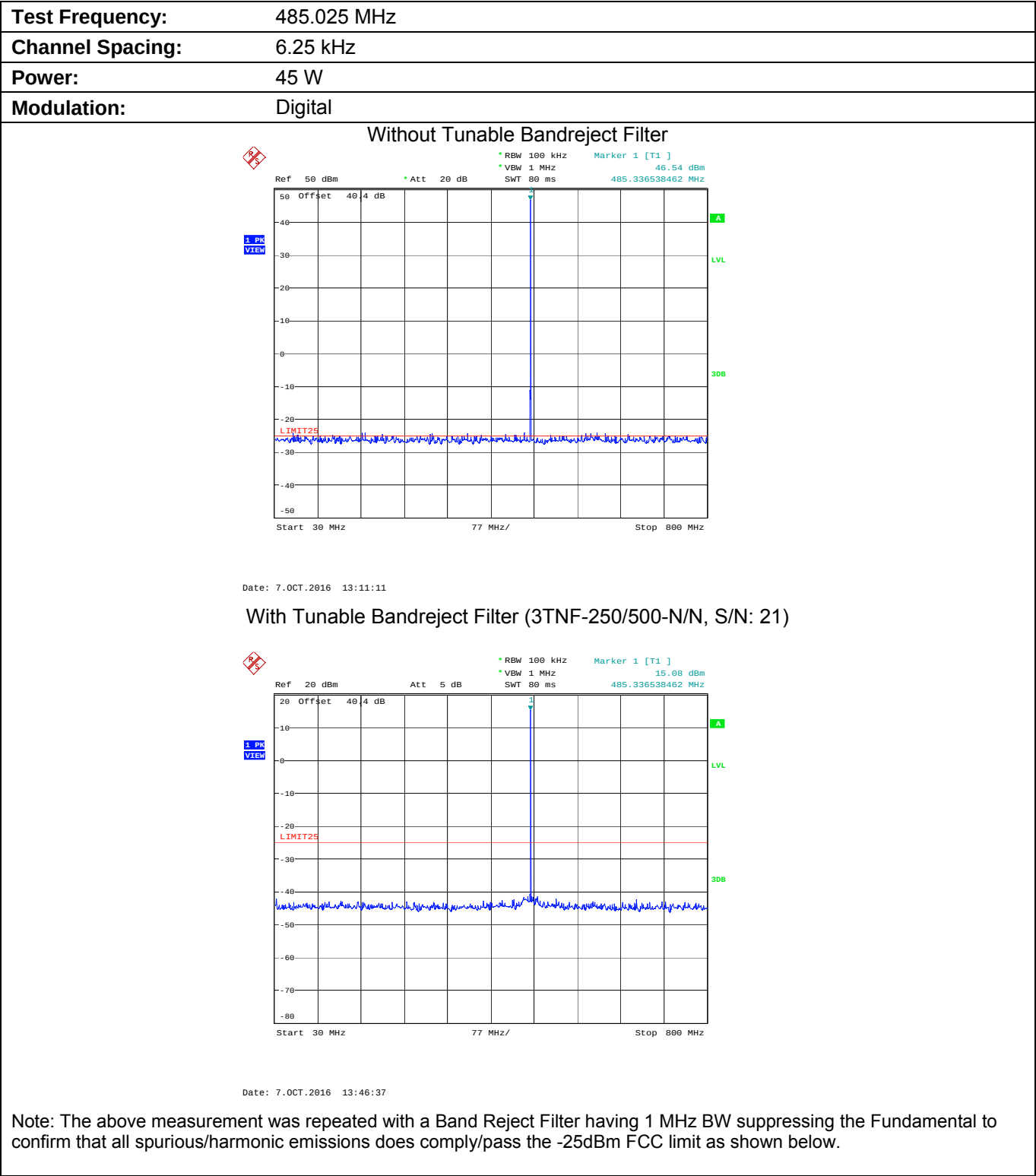
Plot 5.9.4.2.1. Conducted Transmitter Spurious Emissions for 485.025 MHz, High Power, 30 - 800 MHz
