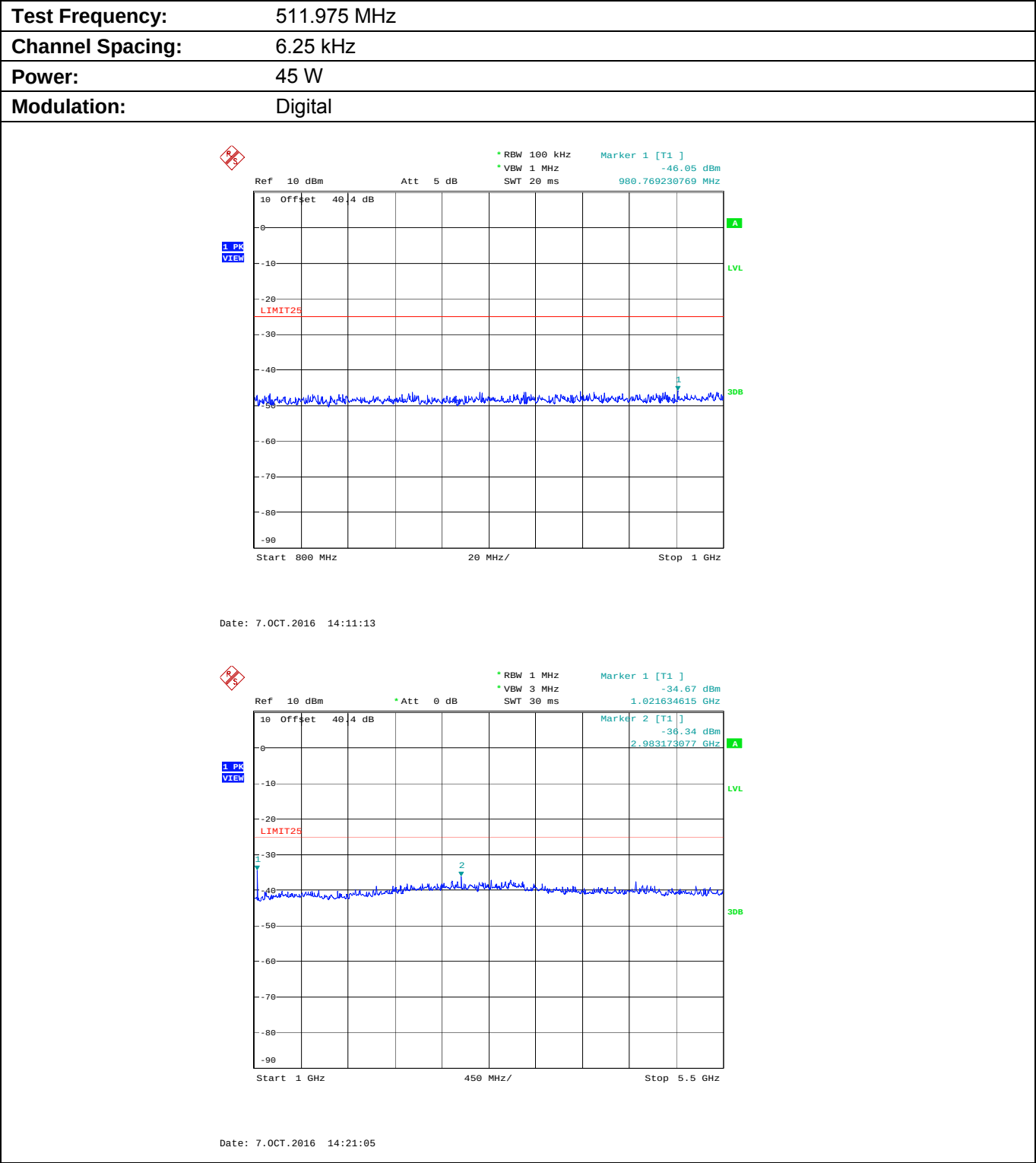
Plot 5.9.4.3.2. Conducted Transmitter Spurious Emissions for 511.975 MHz, High Power, 0.8 - 5.5 GHz
