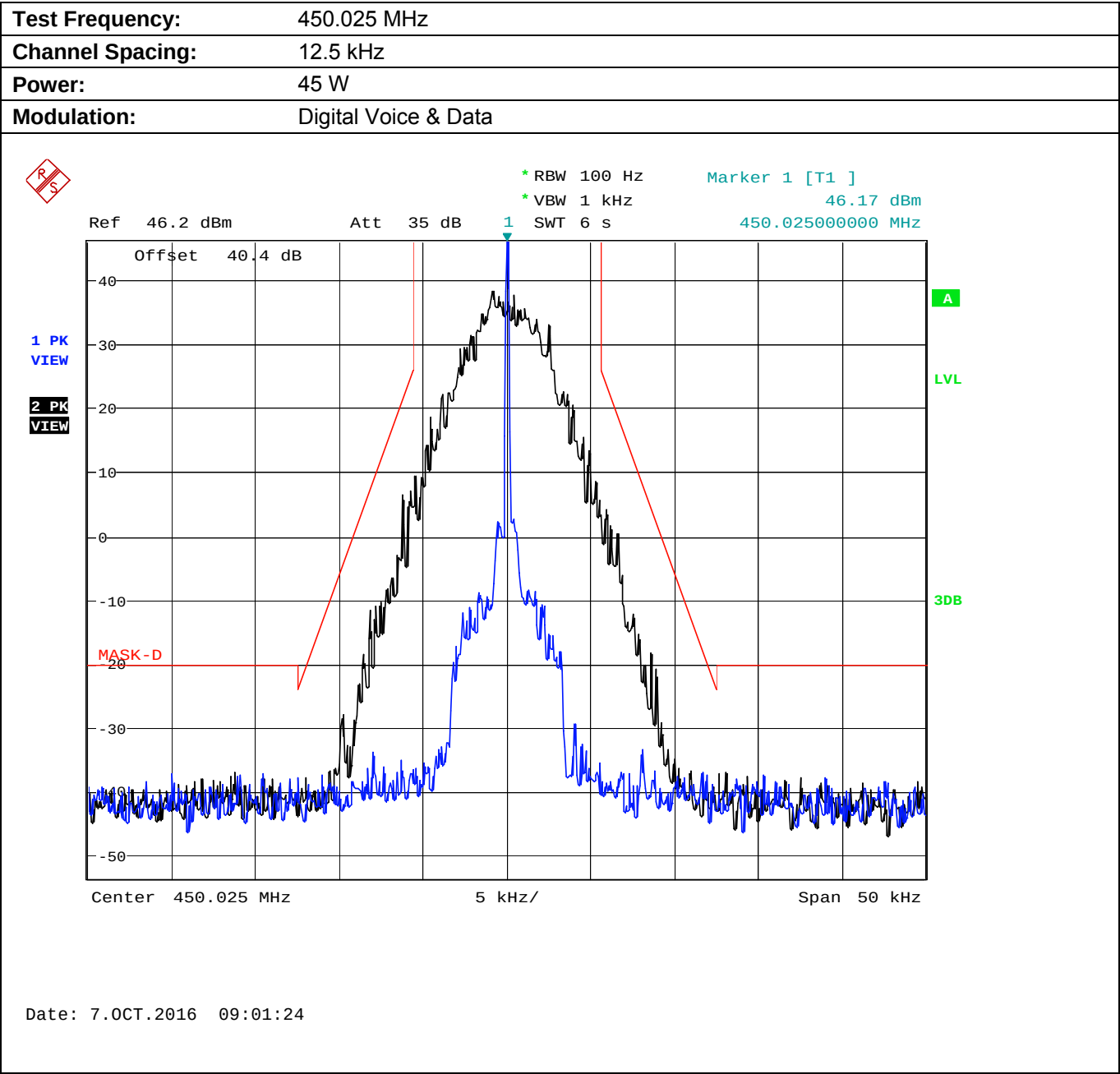
Plot 5.8.4.2.7. Emission Mask D, High Power
