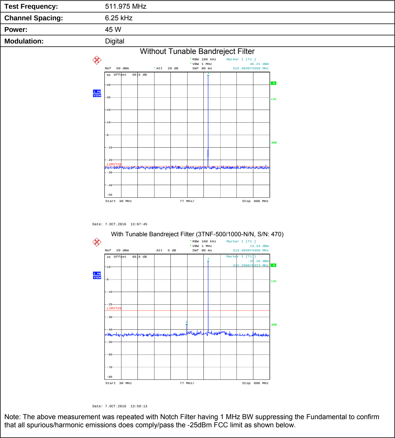
Plot 5.9.4.3.1. Conducted Transmitter Spurious Emissions for 511.975 MHz, High Power, 30 - 800 MHz
