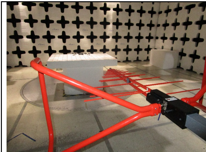
Radiated Emission Below 1G – Front View
