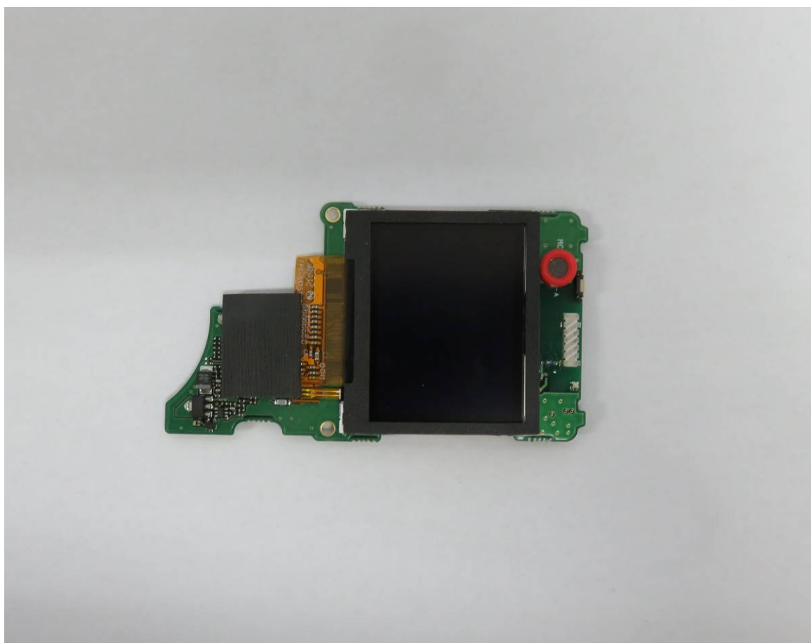
IC-F7020S/T FRONT SIDE A with LCD
