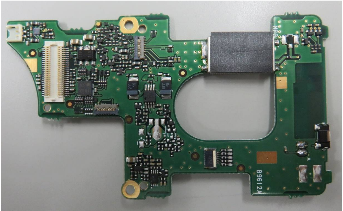
IC-F7020S/T FRONT SIDE B
