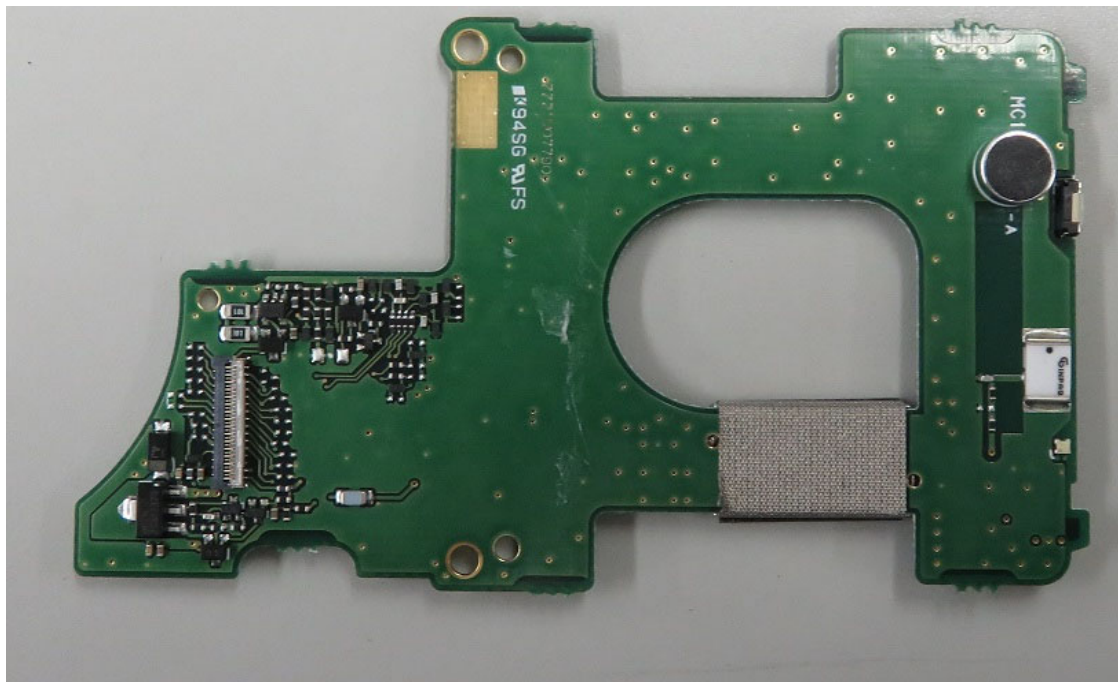
IC-F7020S/T FRONT SIDE A
