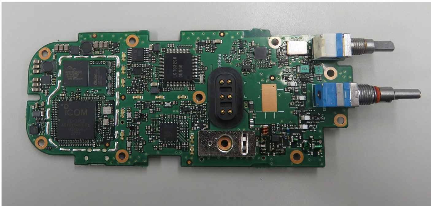
IC-F7020S/T MAIN SIDE B
