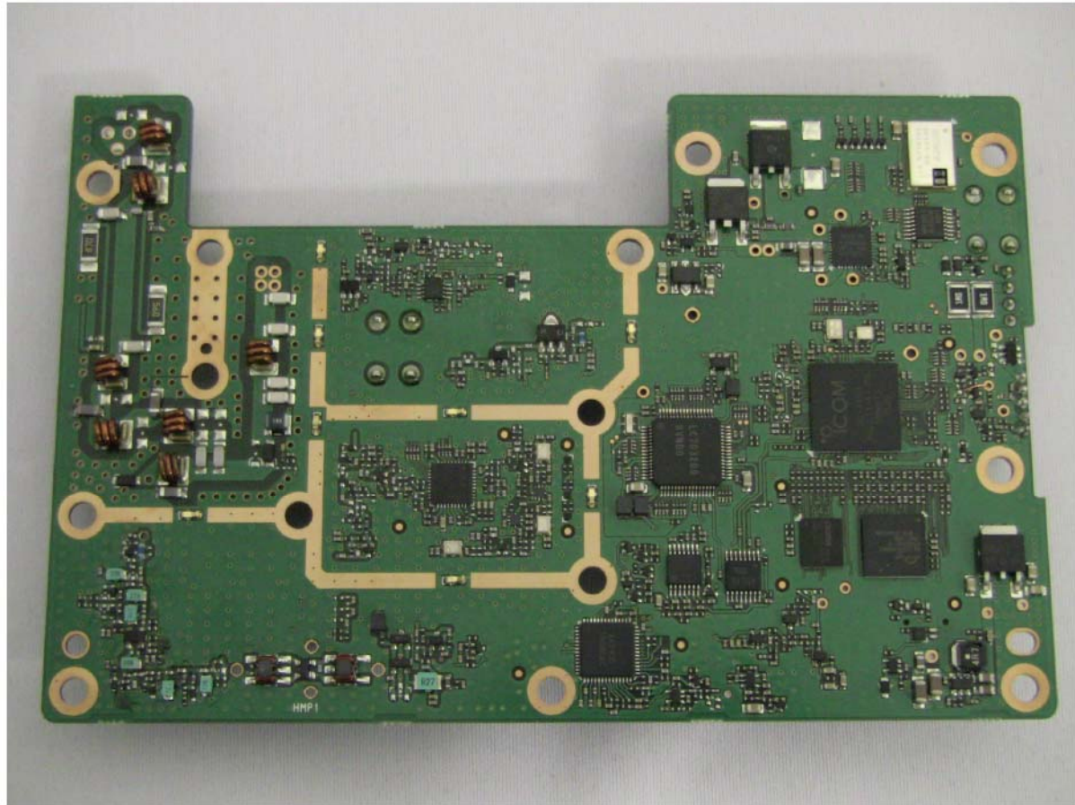
IC-F7520 MAIN-A UNIT B SIDE
